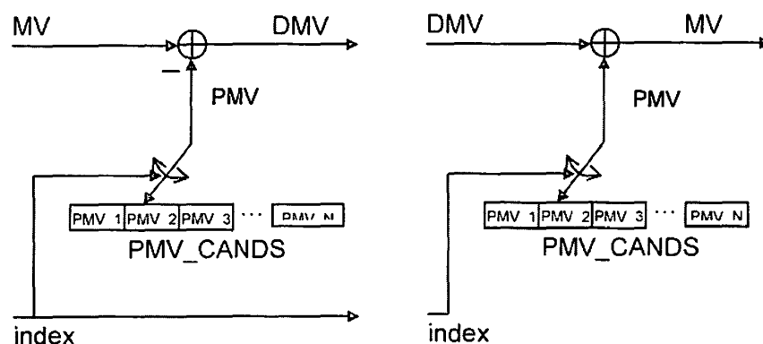
Figure 1 Motion vector coding with signalling of PMV index. Left: encoder, right: decoder.
