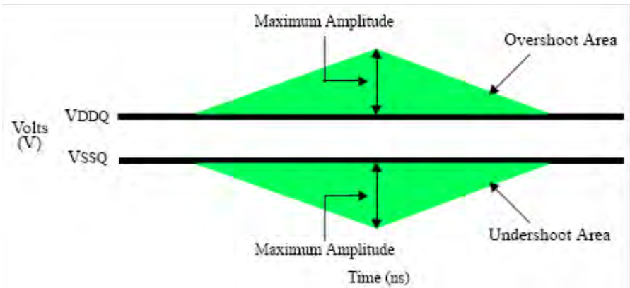
Figure 88 — Clock, Data, Strobe and Mask Overshoot and Undershoot Definition
