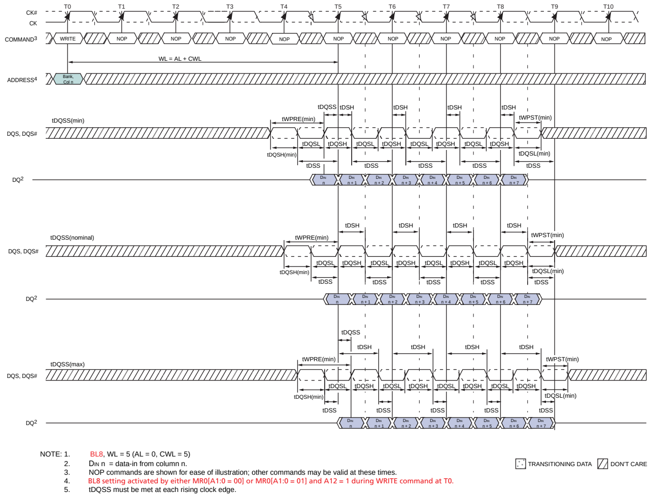
Figure 45 — DDR3 Write Timing Definition
