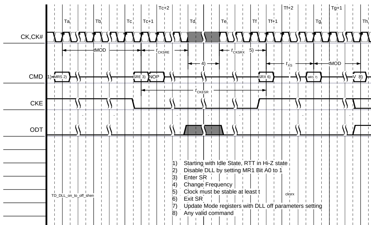
Figure 11 — DLL Switch Sequence from DLL-on to DLL-off
