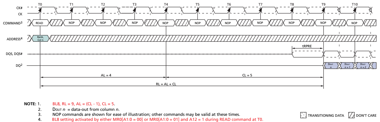
Figure 26 — READ Burst Operation RL = 5 (AL = 0, CL = 5, BL8)
