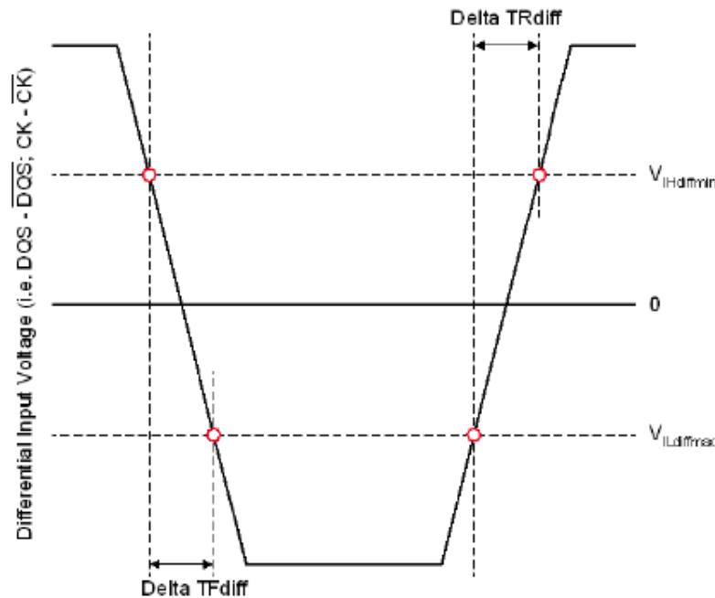
Figure 83 — Differential Input Slew Rate Definition for DQS, DQS# and CK, CK#
