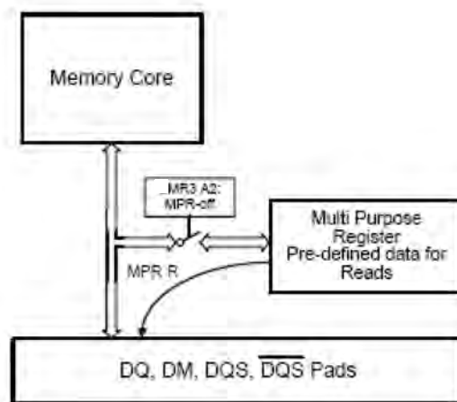
Figure 17 — MPR Block Diagram
