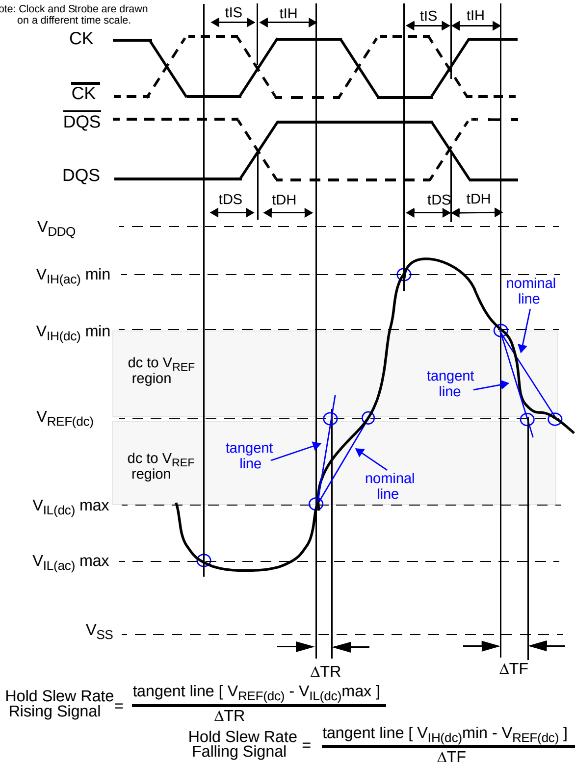
Figure 107 — Illustration of tangent line for for hold time t_{DH} (for DQ with respect to strobe) and t_{IH} (for ADD/CMD with respect to clock)
