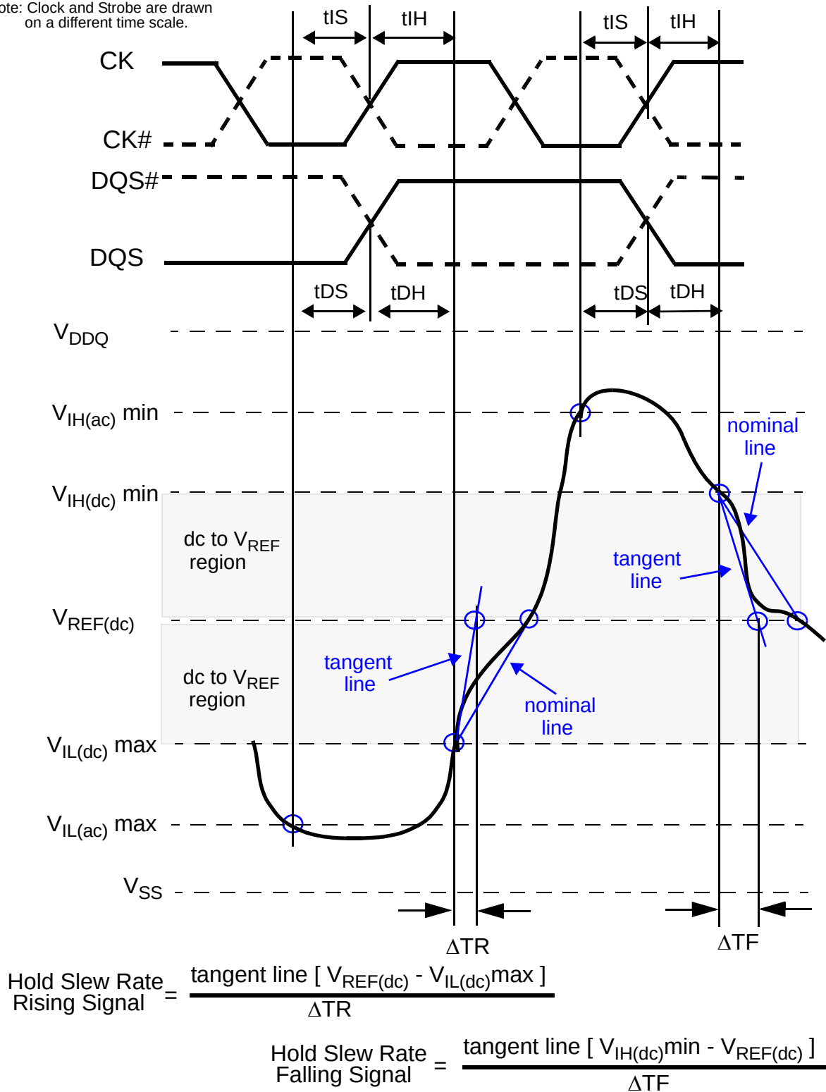
Figure 103 — Illustration of tangent line for for hold time t_{DH} (for DQ with respect to strobe) and t_{IH} (for ADD/CMD with respect to clock)
