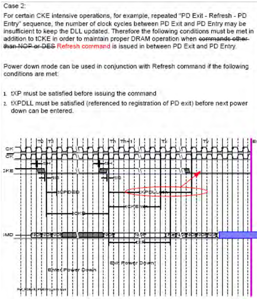
Figure 65 — Power-Down Entry/Exit Clarifications - Case 2
