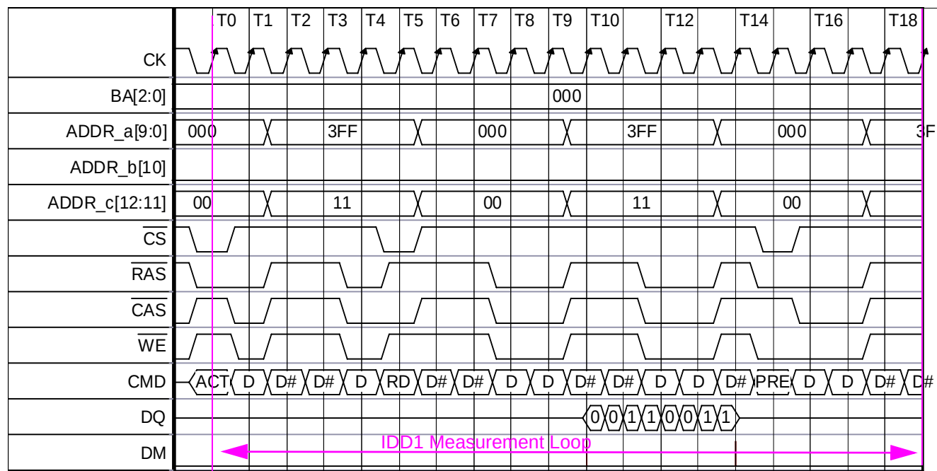
Figure 97 — IDD1 Example (DDR3-800-555, 512Mb x8): Data DQ is shown but the output buffer should be switched off (per MR1 bit A12 = "1") to achieve I_{out} = 0mA . Address inputs are split into 3 parts.
