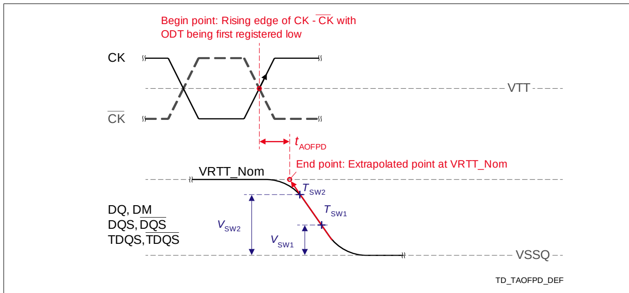
Figure 95 — Definition of t_{\text{AOFPD}}
