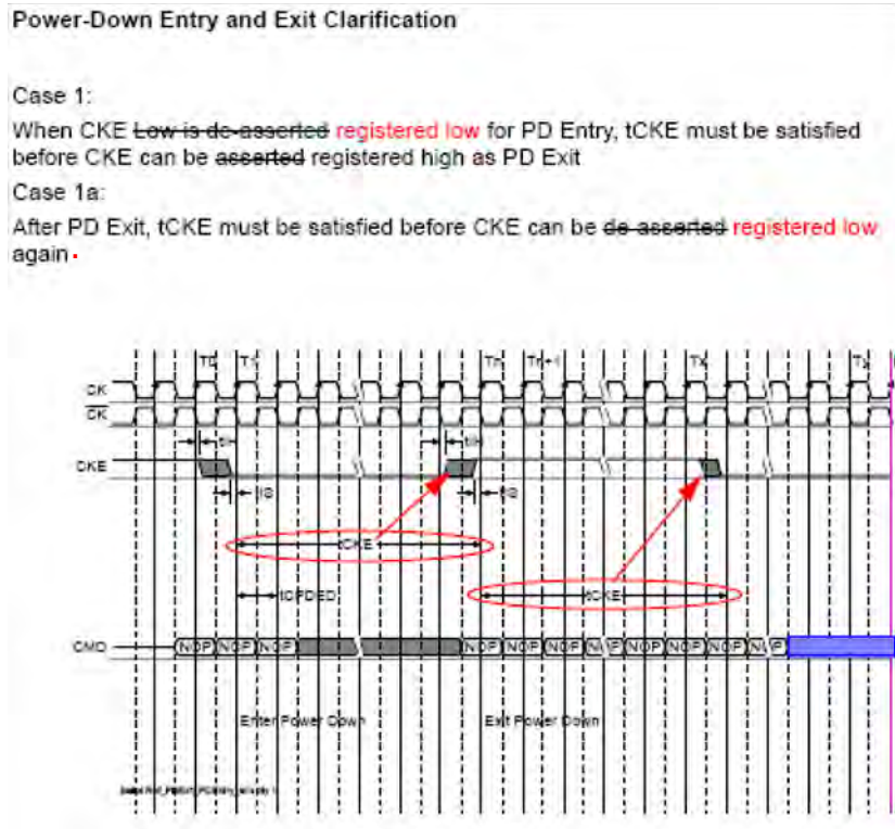
Figure 64 — Power-Down Entry/Exit Clarifications - Case 1
