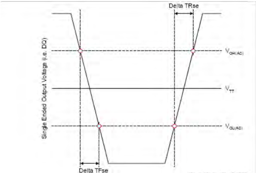
Figure 84 — Single Ended Output Slew Rate Definition
