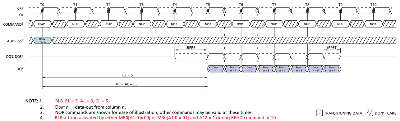
Figure 25 — READ Burst Operation RL = 5 (AL = 0, CL = 5, BL8)
