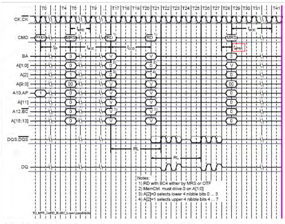
Figure 23 — MPR Readout predefined pattern, BC4, lower nibble then upper nibble
