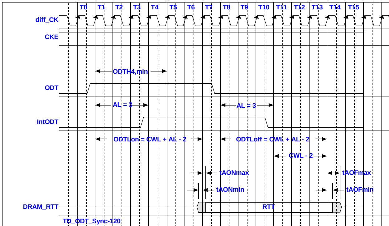
Figure 68 — Synchronous ODT Timing Example for AL = 3 ; CWL = 5 ; ODT_{Lon} = AL + CWL - 2 = 6.0 ; ODT_{Loff} = AL + CWL - 2 = 6
