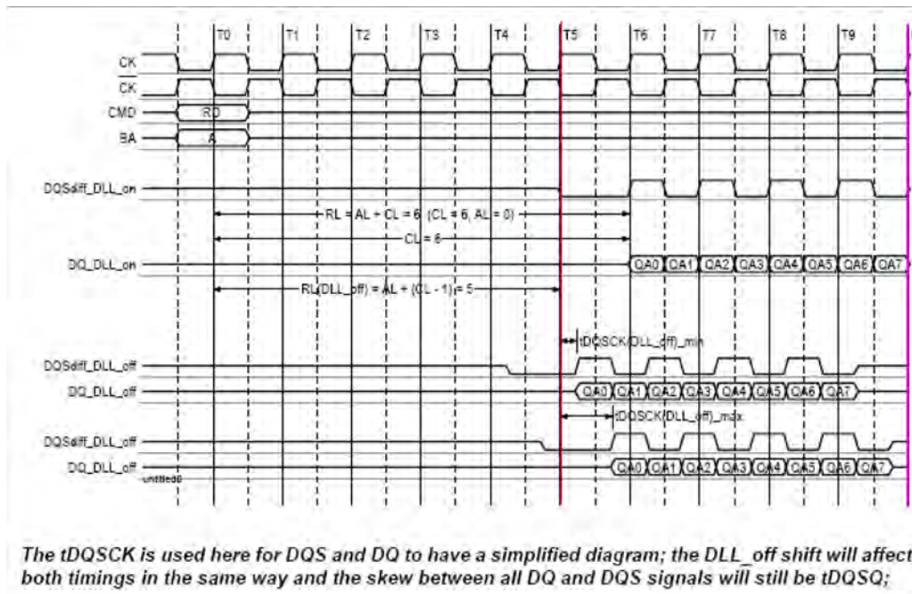
Figure 10 — DLL-off mode READ Timing Operation
