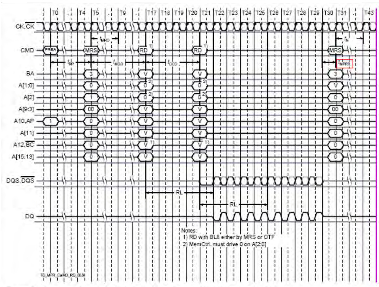
Figure 22 — MPR Readout of predefined pattern, BL8 fixed burst order, back-to-back readout
