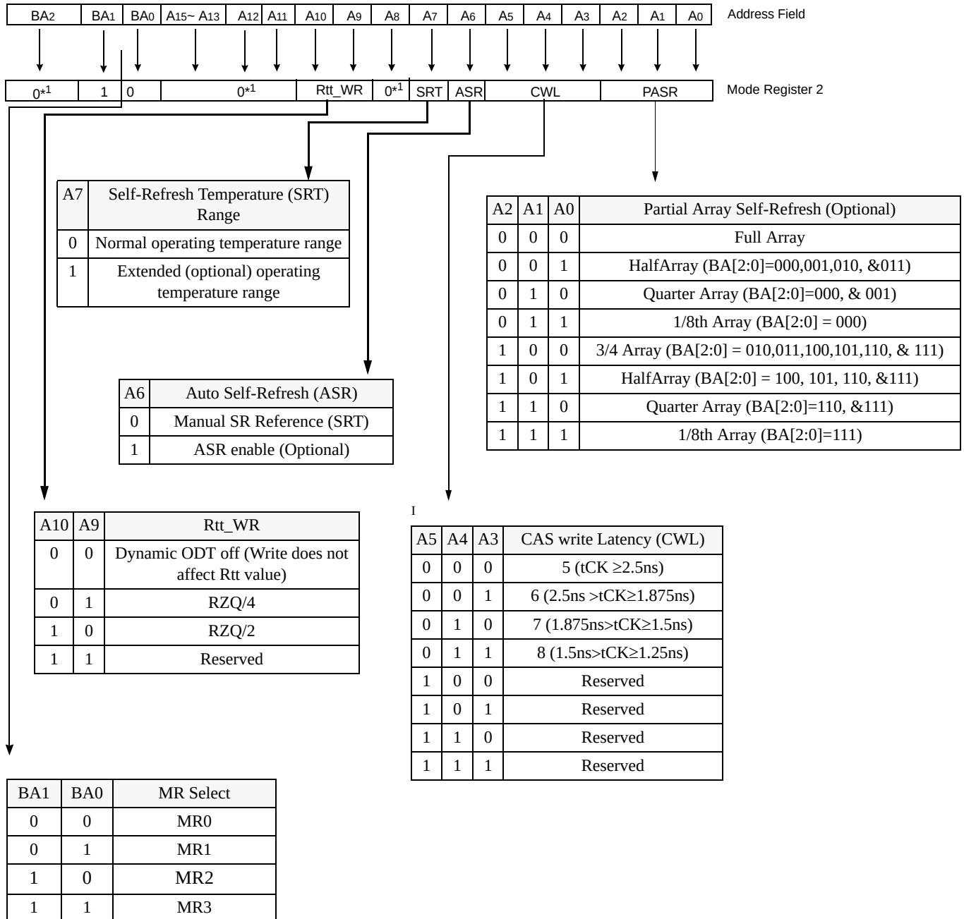
Figure 8 — MR2 Definition
