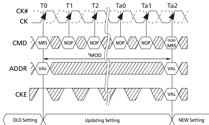
Figure 5 — t_{MOD} Timing
