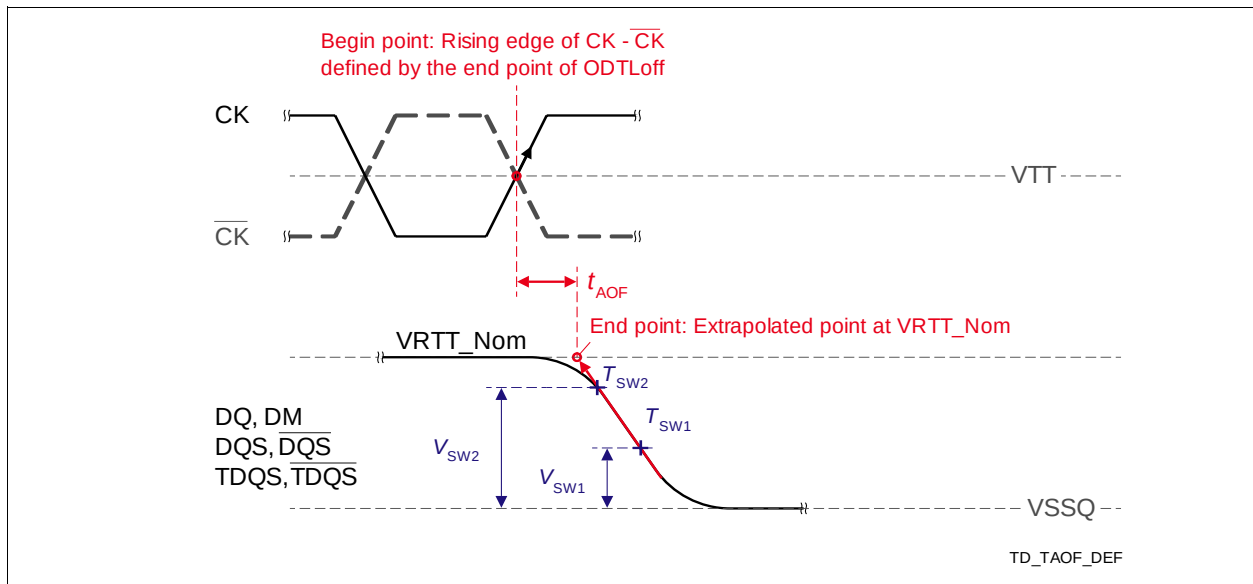
Figure 94 — Definition of t_{\text{AOF}}
