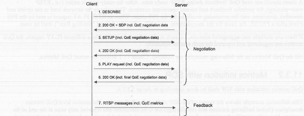
Figure 11.1: QoE metrics negotiation
