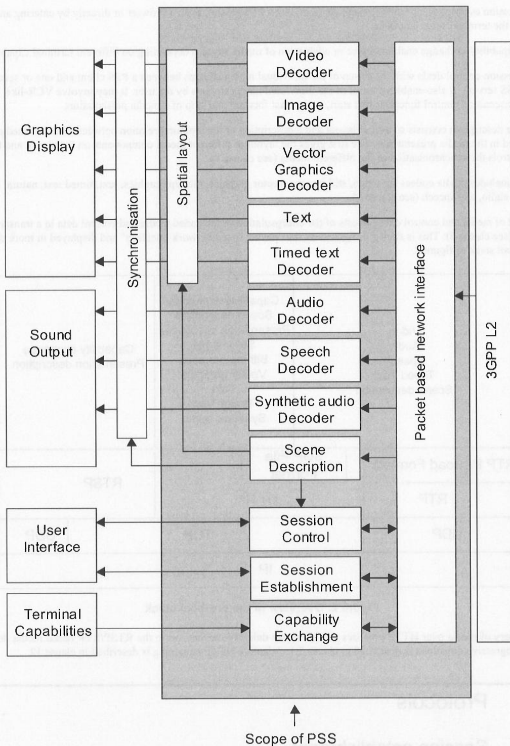
Figure 1: Functional components of a PSS client
