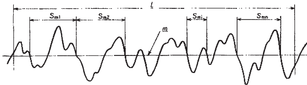
Fig. 5. Determination of S_m
