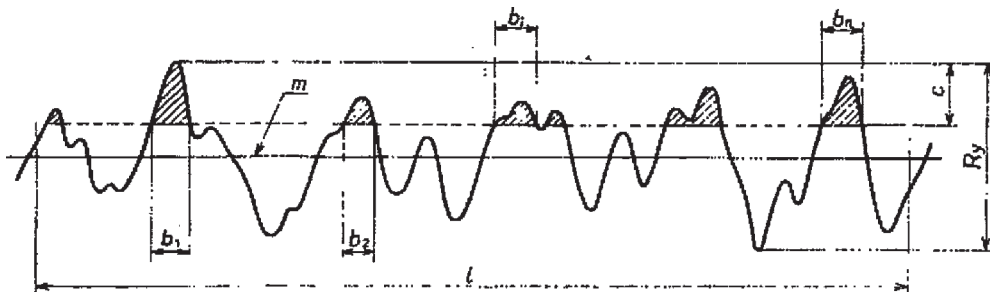
Fig. 7. Determination of t_p
