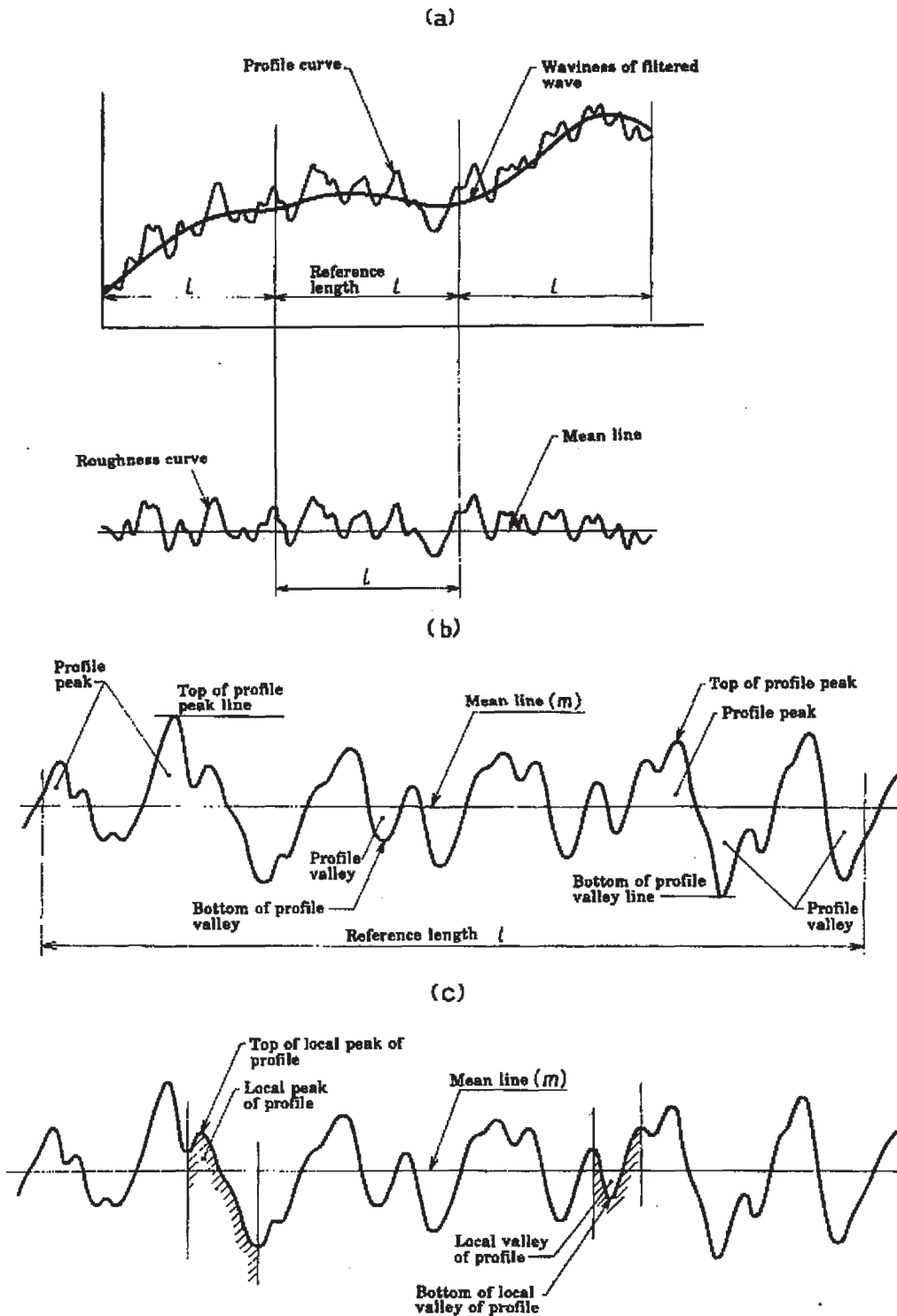
Fig. 1. Explanation on profile curve, roughness curve, mean line, reference length, profile peak, profile valley, local peak of profile and local valley of profile
