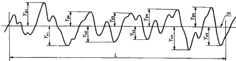
Fig. 4. Determination of R_z
