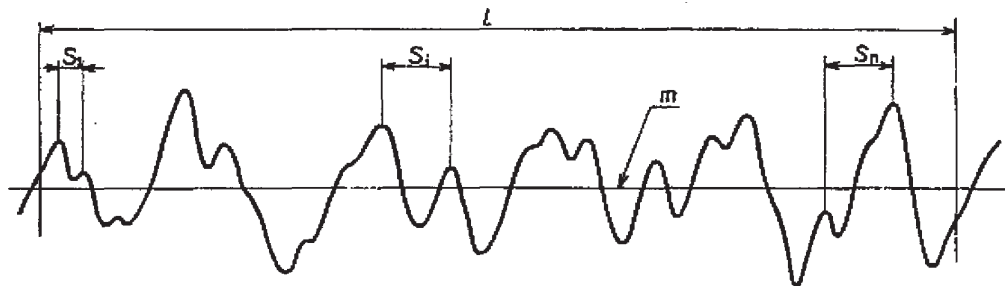
Fig. 6. Determination of S
