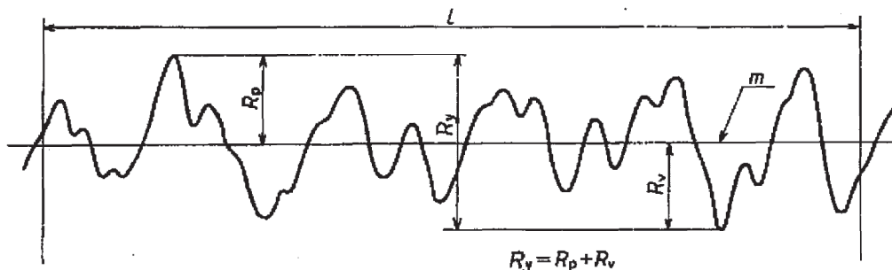
Fig. 3. Determination of R_y
