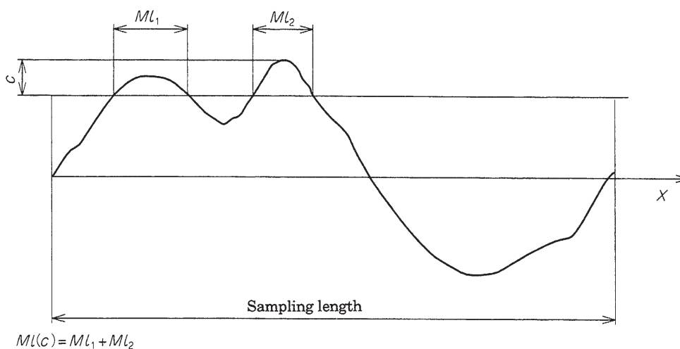
Figure 5 Material length
