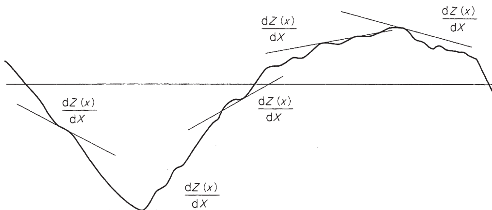
Figure 4 Local slope
