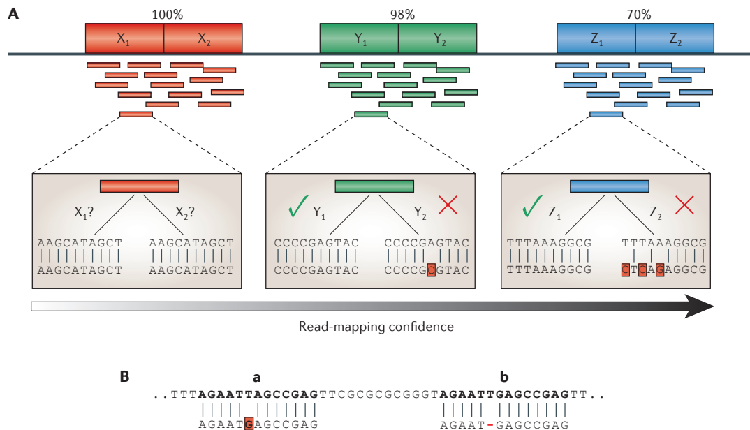
Figure 1 | Ambiguities in read mapping. A | Read-mapping confidence versus repeat-copy similarity. As the similarity between two copies of a repeat increases, the confidence in any read placement within the repeat decreases. At the top of the figure, we show three different tandem repeat regions with two copies each. Directly beneath these tandem repeats are reads that are sequenced from these regions. For each tandem repeat, we have highlighted and zoomed in on a single read. Starting with the leftmost read (red) from tandem repeat X, we have low confidence when mapping this read within the tandem repeat, because it aligns equally well to both X_1 and X_2 . In the middle example (tandem repeat Y, green), we have a higher confidence in the mapping owing to a single nucleotide difference, making the alignment to Y_1 slightly better than Y_2 . In the rightmost example, the blue read that is sequenced from tandem repeat Z aligns perfectly to Z_1 , whereas its alignment to Z_2 contains three mismatches, giving us a high confidence when mapping the read to Z_1 . B | Ambiguity in read mapping. The 13 bp read shown along the bottom maps to two locations, a and b , where there is a mismatch at location a and a deletion at b . If mismatches are considered to be less costly, then the alignment program will put the read in location a . However, the source DNA might have a true deletion in location b , meaning that the true position of the read is b .
