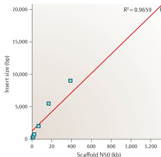
Figure 4 | Longer paired-end libraries improved assembly contiguity in the repetitive potato genome. Each point represents the scaffold N50 size of an assembly of the potato genome that was built using paired-end reads from inserts of a specific size and smaller. Successive points moving from left to right used all previous data plus one additional, longer paired-end library size, which is plotted on the y axis. With the addition of the final, 20 kb library, the scaffold N50 size reached 1.3 Mb. The data in this figure are taken from REF. 56.
