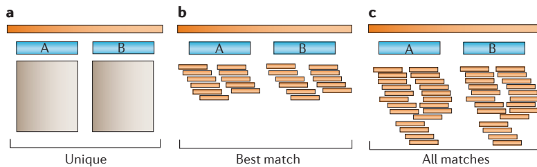
Figure 2 | Three strategies for mapping multi-reads. The shaded rectangles at the top represent intervals along a chromosome. The two blue rectangles below each region represent an identical two-copy repeat containing the paralogous genes A and B. The small orange bars represent reads aligned to specific positions. a | The 'unique' strategy reports only those reads that are uniquely mappable. Because A and B are identical, no alignments are reported. b | The 'best match' alignment strategy reports the best possible alignment for each read, which is determined by the scoring function of the alignment algorithm. In the case of ties, this strategy randomly distributes reads across equally good loci, as shown here. c | The 'all matches' strategy simply reports all alignments for each multi-read, including lower-scoring alignments.
