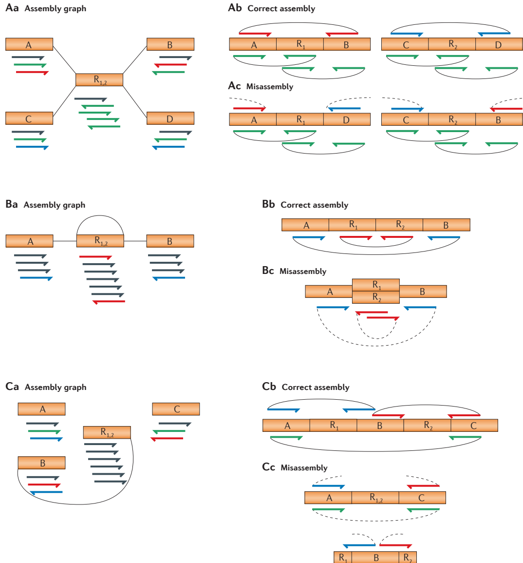
Figure 3 | Assembly errors caused by repeats. A | Rearrangement assembly error caused by repeats. Aa | An example assembly graph involving six contigs, two of which are identical ( R_1 and R_2 ). The arrows shown below each contig represent the reads that are aligned to it. Ab | The true assembly of two contigs, showing mate-pair constraints for the red, blue and green paired reads. Ac | Two incorrectly assembled chimeric contigs caused by the repetitive regions R_1 and R_2 . Note that all reads align perfectly to the misassembled contigs, but the mate-pair constraints are violated. B | A collapsed tandem repeat. Ba | The assembly graph contains four contigs, where R_1 and R_2 are identical repeats. Bb | The true assembly, showing mate-pair constraints for the red and blue paired reads, which are oriented correctly and spaced the correct distance apart. Bc | A misassembly that is caused by collapsing repeats R_1 and R_2 on top of each other. Read alignments remain consistent, but mate-pair distances are compressed. A different misassembly of this region might reverse the order of R_1 and R_2 . C | A collapsed interspersed repeat. Ca | The assembly graph contains five contigs, where R_1 and R_2 are identical repeats. Cb | In the correct assembly, R_1 and R_2 are separated by a unique sequence. Cc | The two copies of the repeat are collapsed onto one another. The unique sequence is then left out of the assembly and appears as an isolated contig with partial repeats on its flank.
