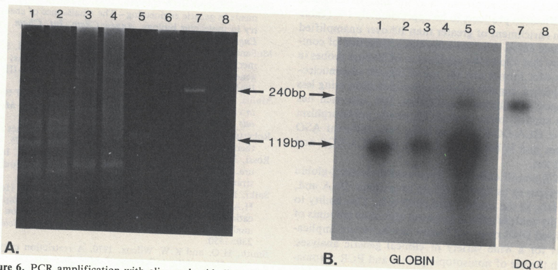
Figure 6. PCR amplification with oligonucleotide linker primers. (A) Ethidium-bromide-stained gel showing total amplified products. (1) Primers PC03 and PC04 on Molt-4 DNA; (2) PC03 and PC04 on GM2064 DNA; (3) GH18 and GH19 on Molt-4; (4) GH18 and GH19 on GM2064; (5) GH18 and GH19 on pBR328:: \beta^A DNA; (6) PC03 and PC04 on Molt-4, no enzyme; (7) primers GH26 and GH27 on LG-2 DNA; (8) GH26 and GH27 on LCL721.180 DNA. (B) Southern blots showing specific amplified products. Lanes are numbered as in A. Lanes 1 through 6 were hybridized to the labeled RS06 oligonucleotide probe. Lanes 7 and 8 were hybridized to a cloned DB \alpha cDNA probe labeled by nick translation.
