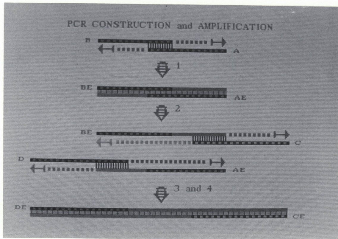
Figure 4. PCR construction and amplification. Oligonucleotides with complementary overlapping 3' ends are extended on each other using DNA polymerase. The double-stranded DNA product of this reaction is extended on both ends by a second stage of several PCR cycles depicted by reactions 2, 3, and 4.
