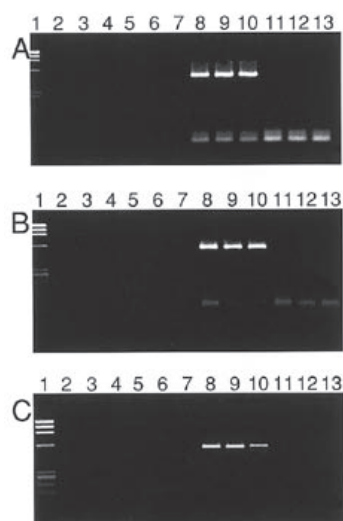
Figure 5. (A) ApoB PCRs with conventional primers; (B) ApoB PCRs with tailed primers; (C) ApoB HANDS PCRs. (A–C) Lane 1, \phi X174/ Hae III size marker; lanes 2–4, with template DNA, without Taq DNA polymerase; lanes 5–7, without template DNA, without Taq DNA polymerase; lanes 8–10, with template DNA, with Taq DNA polymerase; lanes 11–13, without template DNA, with Taq DNA polymerase.
