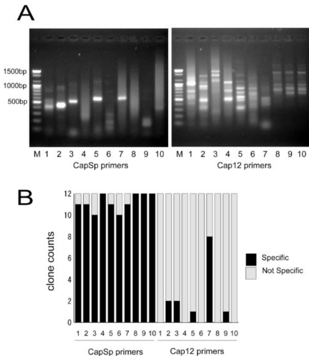
Fig. 4. Improvement of 5'-RACE by the SDSS algorithm. (A) The 5'-RACE products obtained using the primers designed based on the uniqueness of the SDSS (left) and the 3'-end 12mer (right) were separated by gel electrophoresis. (B) The 5'-RACE products shown in (A) were cloned. For each target, twelve clones were sequenced to examine how effectively the bona fide target is cloned. Closed and gray boxes indicate the true and false targets, respectively.
