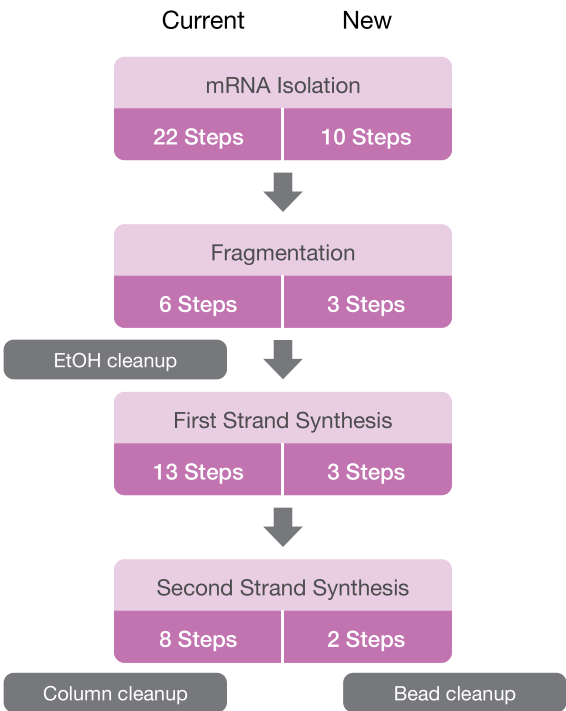
Figure 3: TruSeq RNA Sample Preparation Reagents Provide Significant Savings in Time and Effort
