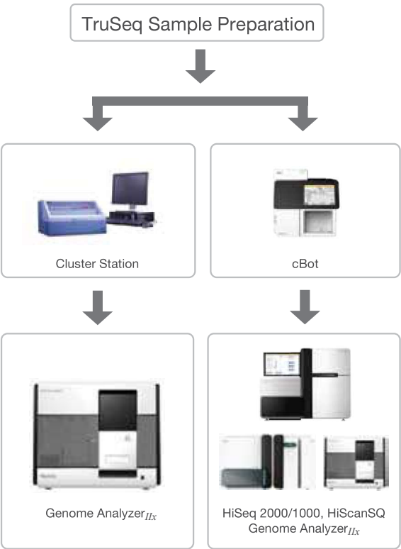
Figure 5. Illumina's Complete Sequencing Solution
