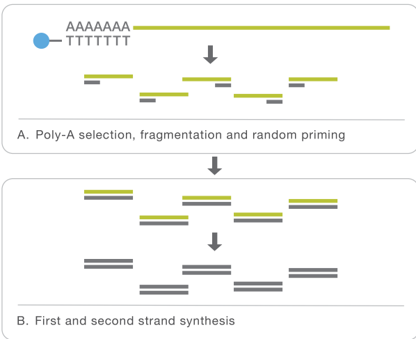
Figure 2: Optimized TruSeq RNA Sample Preparation
