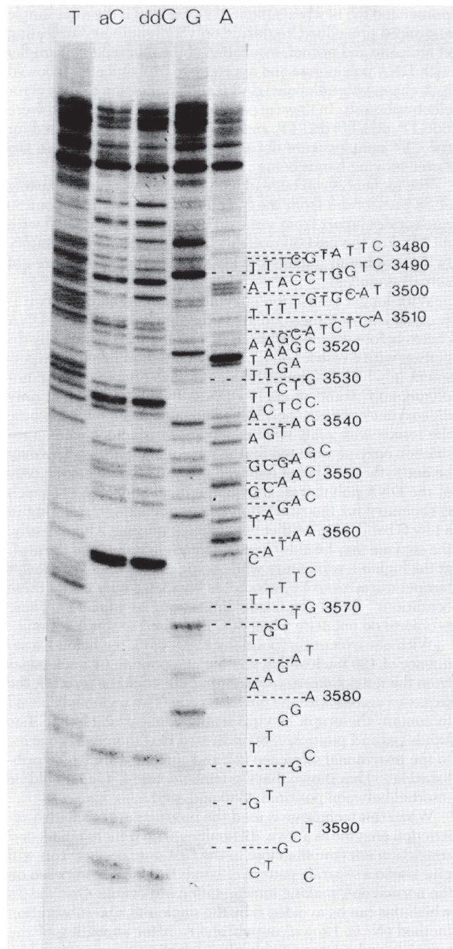
FIG. 3. Autoradiograph of an experiment with fragment A8 as primer on the viral strand of \phi X174 DNA using the single-site ribosubstitution method. Electrophoresis was on a 12% gel at 40 mA for 6 hr. The top 5.5 cm is not shown. Inhibitors used were (left to right) ddTTP, araCTP, ddCTP, ddGTP, and ddATP.
