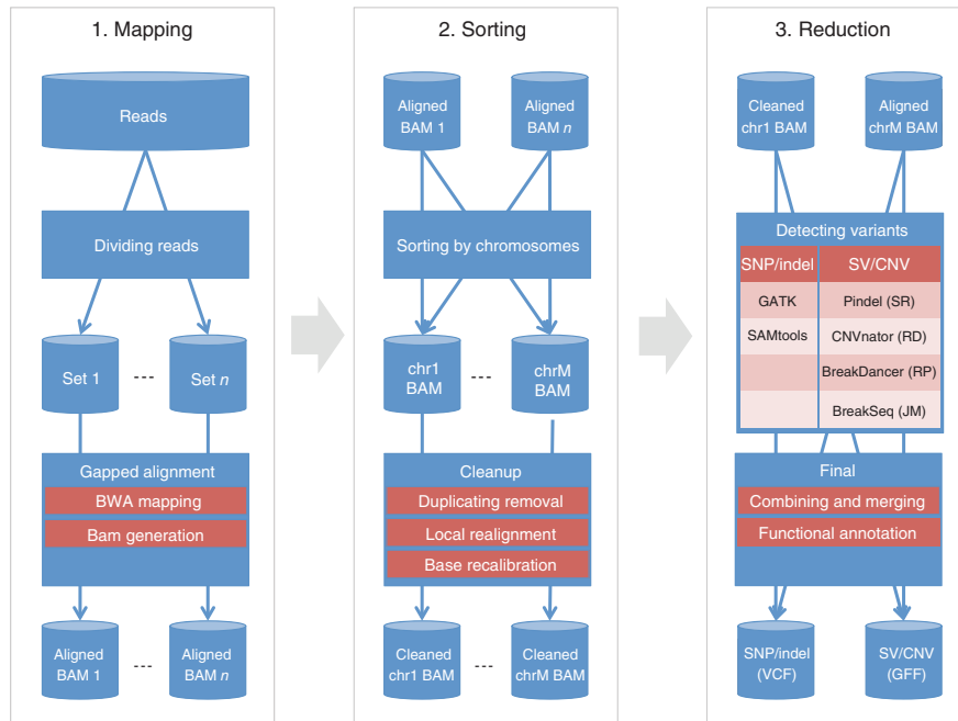
Figure 1 A MapReduce approach for detecting genetic variants from high-throughput genome sequencing. Phase 1 is the mapping phase including sequence alignment. Phase 2 is the sorting phase including sorting alignments by mapped chromosomes. Phase 3 is the reduction phase including variant detection. chr1, chromosome one; chrM, chromosome M; SV, structural variation; SR, split-read analysis; RD, read-depth analysis; RP, read-pair mapping; JM, junction mapping; VCF, variant call format; GFF, general feature format.
