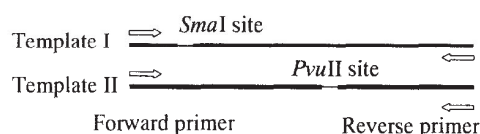
FIG. 1. Schematic representation of PCR templates and primers used by Judo et al. (12). Templates I and II differed in only two nucleotide pairs shown by thin lines.
