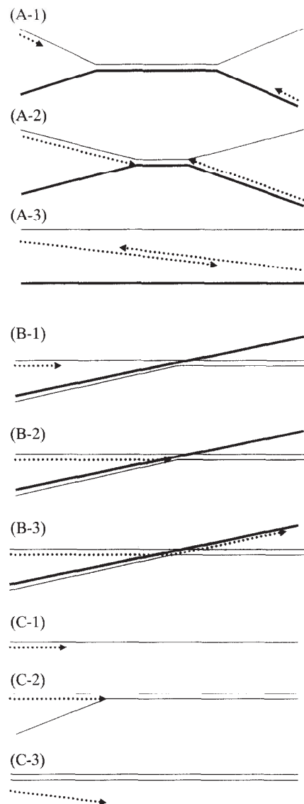
FIG. 5. Models of how chimeras form (8).
