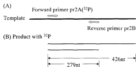
FIG. 3. Schematic representation of the PCR template and primers (A) used by Odelberg et al. (8) for the formation of chimeras, and products (B) after a single thermal cycle.
