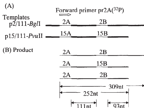
FIG. 4. Schematic representation of the PCR templates and primer (A) used by Odelberg et al. (8) for the formation of chimeras, and products (B) after a single thermal cycle. The two templates had the same sequence except for the two 20-bp sites shown by thin lines.
