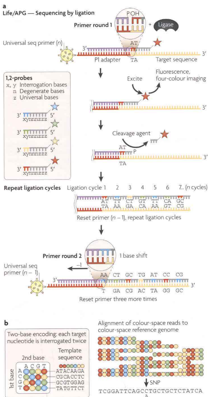
Figure 3 | Next-generation sequencing technologies that use emulsion PCR. a | A four-colour sequencing by ligation method using Life/APG's support oligonucleotide ligation detection (SOLiD) platform is shown. Upon the annealing of a universal primer, a library of 1,2-probes is added. Unlike polymerization, the ligation of a probe to the primer can be performed bi-directionally from either its 5'-PO 4 or 3'-OH end. Appropriate conditions enable the selective hybridization and ligation of probes to complementary positions. Following four-colour imaging, the ligated 1,2-probes are chemically cleaved with silver ions to generate a 5'-PO 4 group. The SOLiD cycle is repeated nine more times. The extended primer is then stripped and four more ligation rounds are performed, each with ten ligation cycles. The 1,2-probes are designed to interrogate the first (x) and second (y) positions adjacent to the hybridized primer, such that the 16 dinucleotides are encoded by four dyes (coloured stars). The probes also contain inosine bases (z) to reduce the complexity of the 1,2-probe library and a phosphorothiolate linkage between the fifth and six nucleotides of the probe sequence, which is cleaved with silver ions 106 . Other cleavable probe designs include RNA nucleotides 107,108 and internucleosidic
