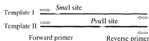
FIG. 1. Schematic representation of PCR templates and primers used by Judo et al. (12). Templates I and II differed in only two nucleotide pairs shown by thin lines.
