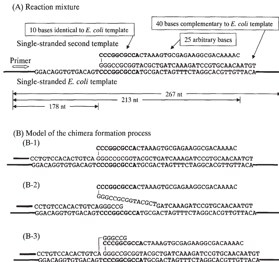
FIG. 6. Schematic representation of the PCR templates and primer used by Patel et al. (9) for the formation of chimeras (A), and a model of the process (B). The sequence in boldface type in the second template was the same as that in the E. coli template.
