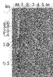
Figure 2. Amplification products generated from walking upstream from exon 1 of the human tissue-type plasminogen activator gene. PCR products in lanes 1–5 were obtained from the EcoRV , ScaI , DraI , PvuII and SspI adaptor-ligated DNA libraries, respectively. Lanes M contain 1 kb DNA size markers (Life Technologies). The sequence of the TPA specific primers were: Primary PCR: 5'-AGA AAC CCG ACCTAC CAC GGC TTG CTC CTT-3'. Secondary PCR: 5'-CCC TTT CCT CGC AGA AAT TTT CTC TCC AGC-3'.
