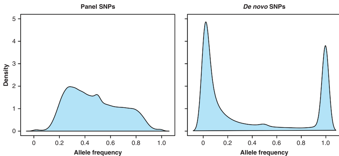
FIG. 3. Distribution of allele frequencies. Polymorphic sites of the target panel (on the left) and de novo genotyped sites (on the right). De novo sites show a prominent sampling of rare alleles.
