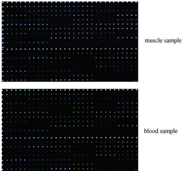
Fig. 1. SNP genotyping of two samples from the same person.
