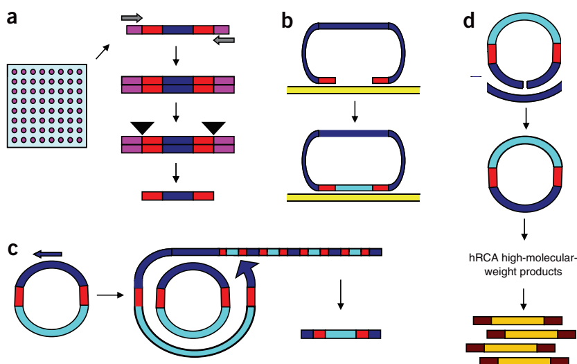
Figure 1 | Schematic of multiplex exon capture. (a) A library of 100-mer targeting oligo precursors is synthesized in parallel on a programmable microarray. Each oligo consists of common 15 nt flanking sequences (purple), unique 20 nt targeting arms (red) and a common 30 nt linker (dark blue). The oligos are released and PCR amplified with a single set of primers directed at the common flanking sequences. Double digestion with nicking restriction endonucleases (black triangles) releases a library of single-stranded 70-mers. (b) The unique targeting arms (red) of individual targeting oligos are designed to hybridize immediately upstream and downstream of each exon of interest. Hybridization to genomic DNA (yellow) is followed by an enzymatic gap-filling and ligation step, such that a copy of the sequence of interest is incorporated into a circle (light blue). The figure is not drawn to scale; the length of the gap-fill ranged from 60 to 191 bp. (c) Enrichment and amplification of exon-capture circles includes exonuclease digestion of linear material (not shown), linear rolling circle amplification and PCR amplification. Primers for the latter two steps are directed at the common linker sequence (dark blue). (d) To generate a shotgun sequencing library, amplicons are recircularized via their common linker (dark blue) and subjected to hyperbranched RCA with phi29 polymerase and random hexamers. High-molecular-weight products of the hRCA reaction are randomly sheared and appended with universal adaptors to generate the shotgun sequencing library.
