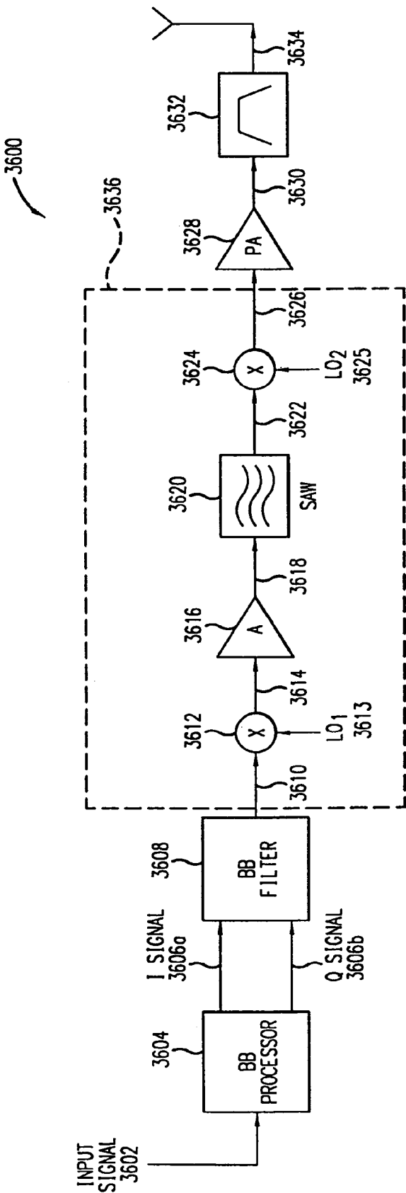
CONVENTIONAL TRANSMITTER
