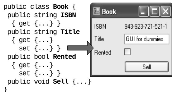
Figure 5: Generation GUI from source code.
