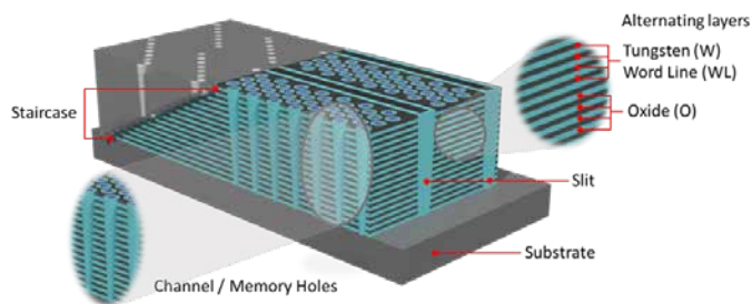
Figure 1. Anatomy of 3D NAND.
