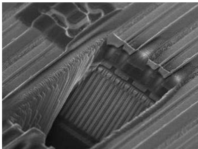
Figure 4. Wide-area diagonal mill of 3D NAND device.
