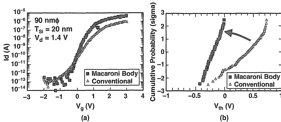
FIGURE 7.16 (a) Typical I_d - V_g characteristics of conventional vertical transistor and “macaroni” body vertical transistor. (b) V_{\text{th}} distribution of conventional and macaroni body vertical transistor.
