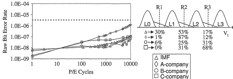
FIGURE 6.71 Erratic over-programming. RBER after programming data, as a function of prior program/erase cycles. Errors were logged at the cycle points noted by the symbols. The dashed line is the RBER where the instantaneous UBER (Uncorrectable Bit Error Rate) reaches 10^{-15} . Nonmonotonic curves result from small sample sizes and erratic RBER behavior. Schematic illustration of the dominant types of program errors and the percentage weighting of each type for each product. The RBER was dominated by cells with higher V_t 's than intended; exceptions exist to some degree and result in percentages sometimes adding to less than 100%. RBER is gradually increased with P/E cycling increasing. The percentage of fail bits for each level is dependent on product (provider). Oxide trap-assisted tunneling is a major root cause.
