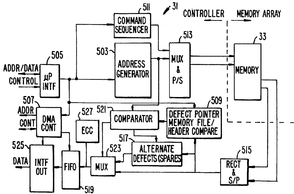
READ DATA PATH CONTROL
