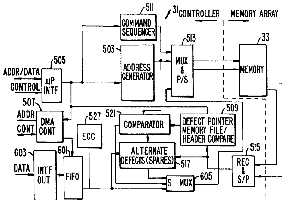
WRITE DATA PATH CONTROL
