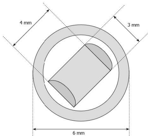
Figure 3 Cross-sectional profile of MM.
