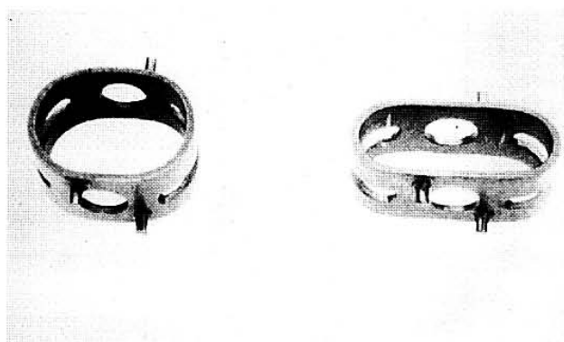
Figure 7: Spinal vertebrae spacer shown in the martensitic state (left) and deployed superelastic state (right). The properties of Nitinol promote more rapid recovery due to the similarity of mechanical properties between the implant and the surrounding tissue.
