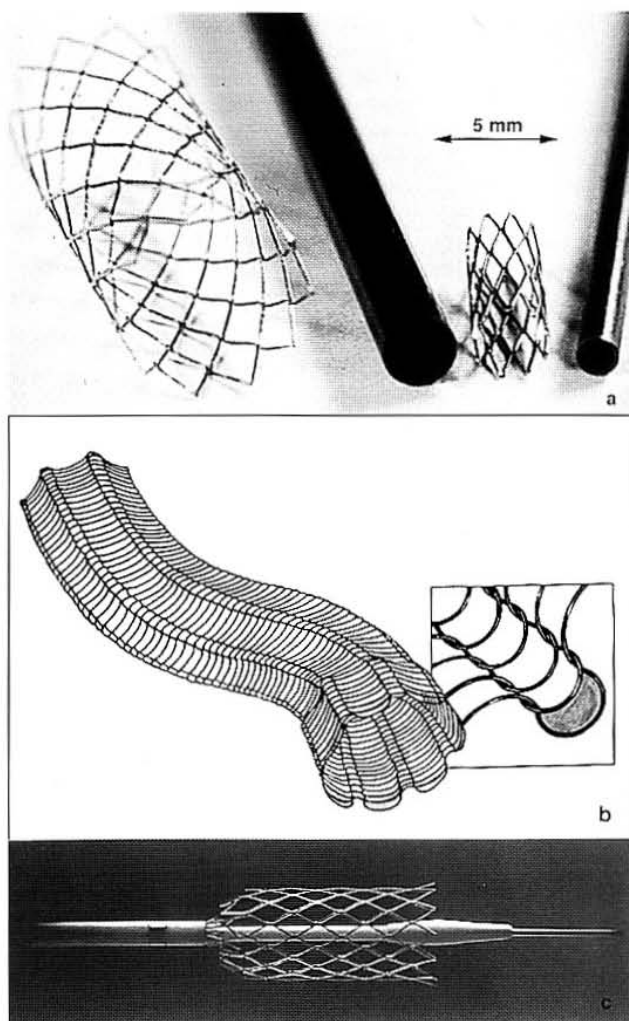
Figure 8: Stents made from Nitinol tubing appear to be of the greatest interest (a), though wire stents, such as the Microvase device shown in (b) are already in use in the United States. Deployment of an Angiomed stent (from tubing) is shown in (c).
