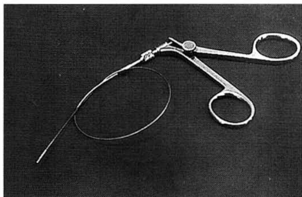
Figure 4: A 1 mm diameter urological grasper demonstrates kink resistance. The shaft consists of a Nitinol wire concentrically placed in a Nitinol tube; the distal end is a stainless steel, hinged "grasper", opening to about a 90° included angle.
