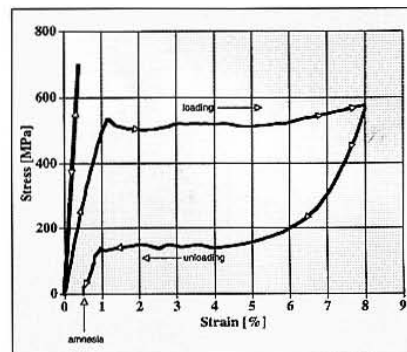
Figure 1: Stress strain curve for a Ti-50.8 at. % Ni alloy tested 10 °C above its A_f temperature. A typical elastic loading-unloading curve for stainless steel is shown in light gray.
