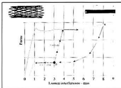
Figure 9: Biased stiffness illustrated in a stent. A stent is manufactured in the open configuration (left), and deformed to a closed position (A). After deformation is complete, it is deployed by releasing from a catheter, following the light gray unloading arrows, until the lumen is filled and expansion stopped (shown by the dark circle marked 'B'). The gentle pressure against the vessel wall is controlled by the unloading arrows, but effort to re-close the vessel are resisted by the stiffness indicated by the unloading arrows. Note that a re-expansion of the stent to a larger diameter moves the circle to the left, but the same biased stiffness is maintained.
