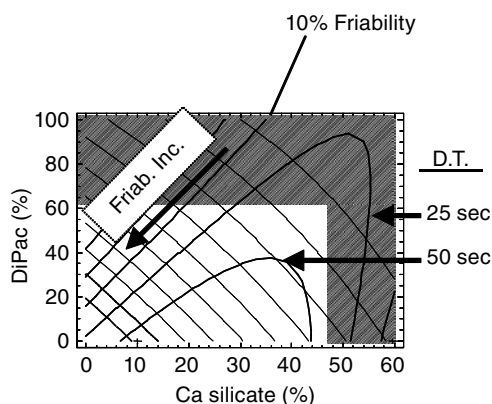
FIGURE 2 An experimental direct compression formulation containing various ratios of DiPac (compactible sugar) and calcium silicate. 15% super disintegrant and 20 MPa of compression force was used. D.T: Disintegration time (seconds) Friab. Inc.: Increasing friability. Source: Redrawn from Ref. 19.
