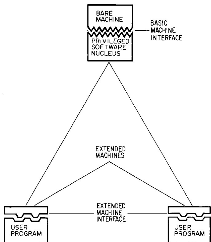
Figure 1. Conventional Extended Machine Organization
