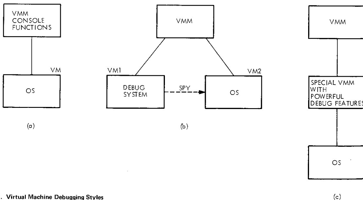
Figure 7. Virtual Machine Debugging Styles
