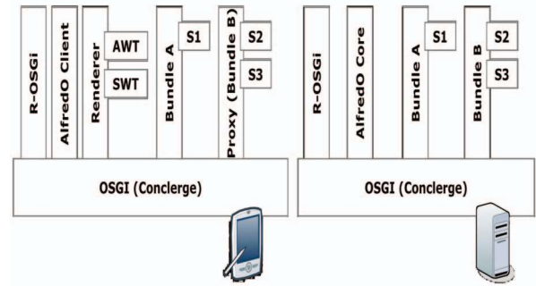
Fig. 5: AlfredO Architecture
