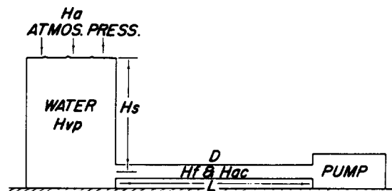
Fig. 3—Forces affecting net positive suction head (NPSH).
