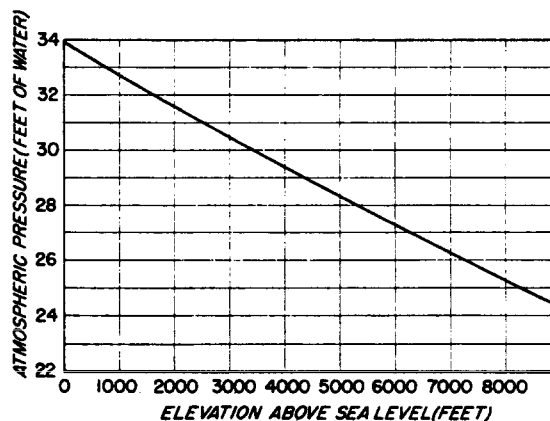
Fig. 4—Atmospheric pressure.
