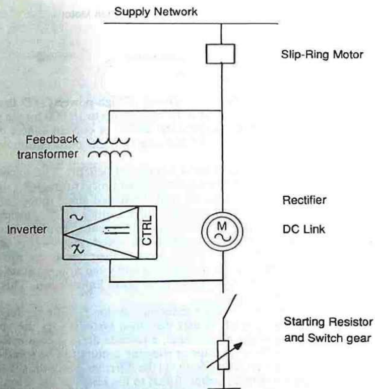
FIG. 20-78 Slip recovery (cascade) drive.
