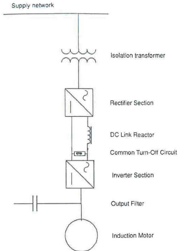
FIG. 20-76 LCI drive with induction motor.
