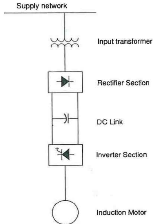
FIG. 20-77 Voltage-source PWM inverter drive.
