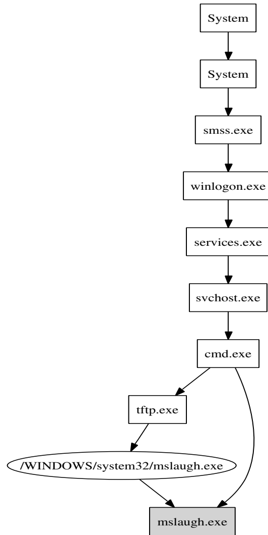
Figure 4.6: Backward information-flow graph for mslaugh attack
