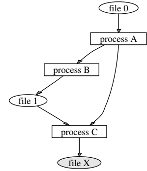
(c) dependency graph generated by GraphGen
