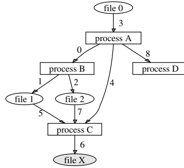
(b) dependency graph for complete event log
