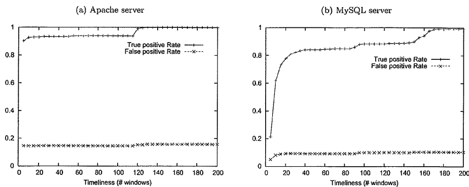
Figure 4: Optimal filters, Timeliness detection
