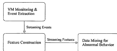
Figure 1: Our VMM IDS high-level design.
