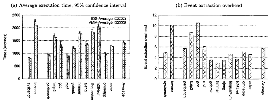
Figure 7: Performance measurements for IOzone, SysBench and SpecINT2006
