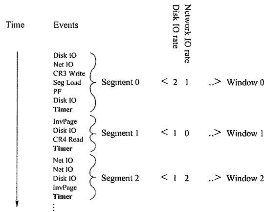
Figure 2: Constructing Features. Events (a) → Basic features (b)
