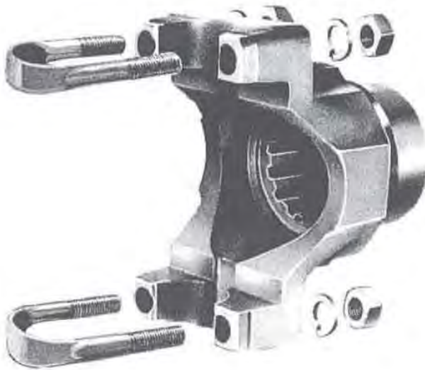
Fig. 1 — End yoke (U-bolt type)
