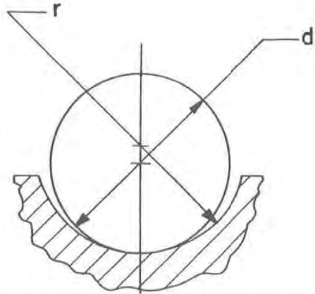
Fig. 4 — Cross section of circular arc ball groove
