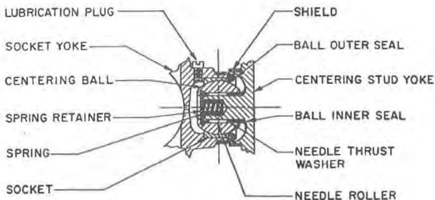
Fig. 10 — Centering ball and stud for driveshaft applications
