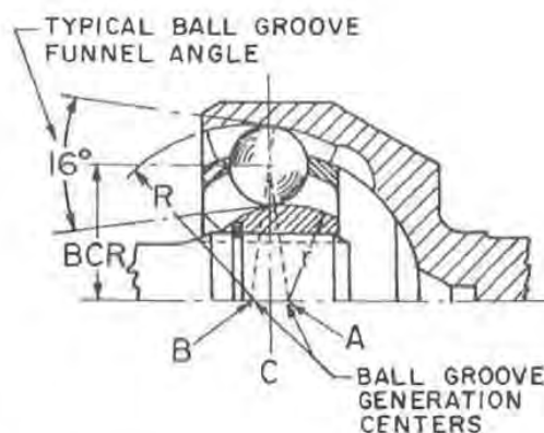
Fig. 10 — Diagram illustrating ball groove funnel angle
