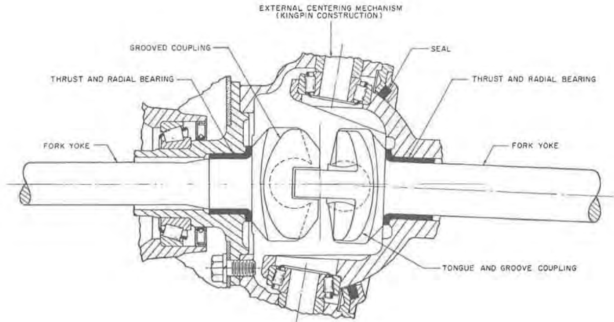
Fig. 1 — Tracta universal joint
