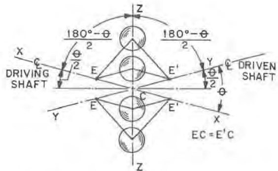
Fig. 3 — Diagram illustrating principle of transmission of constant velocity
