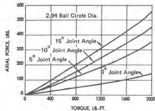
Fig. 12 — Tripot joint axial force characteristics
