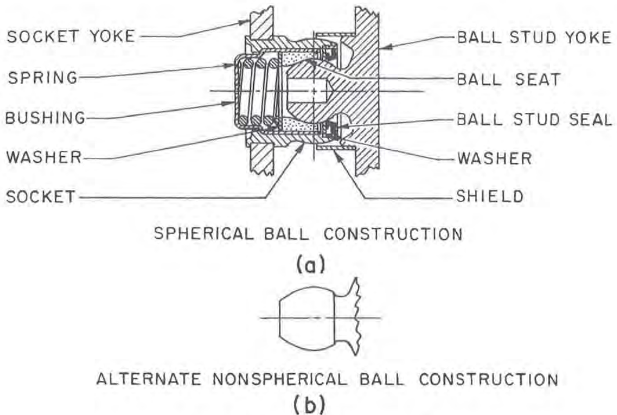
Fig. 11 — Ball stud and seat for driveshaft applications
