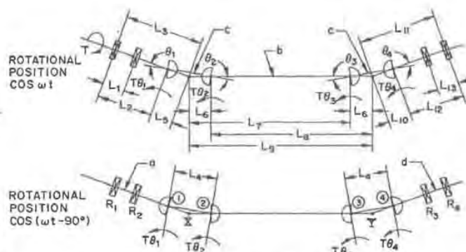
Fig. 5 — Secondary couples in one piece driveline with double Cardan joints
