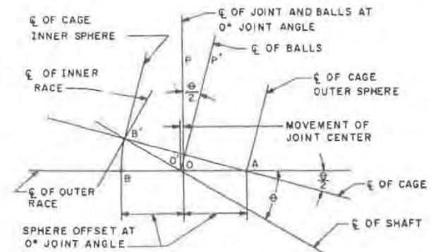
Fig. 2 — Diagram illustrating positioning of cage and balls in bisecting angle plane
