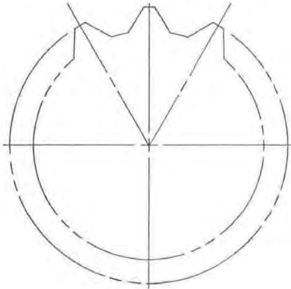
Fig. 13 — Truncated star serrations
