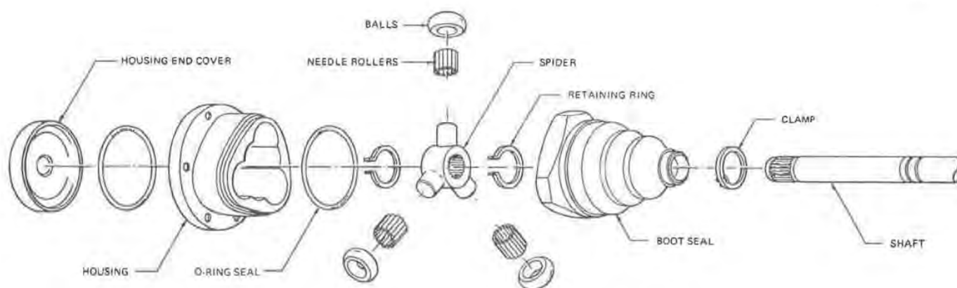
Fig. 8 — Tripot universal joint (end motion type)
