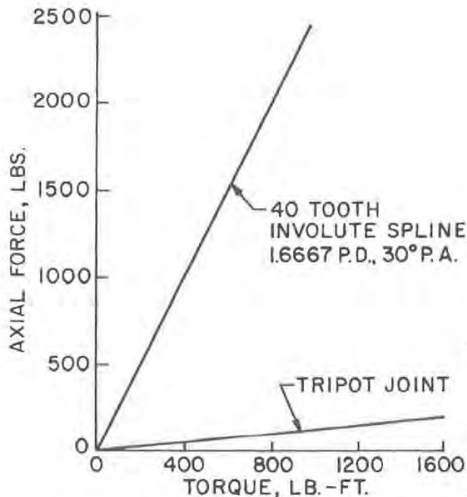
Fig. 11 — Comparison of typical axial force characteristics
