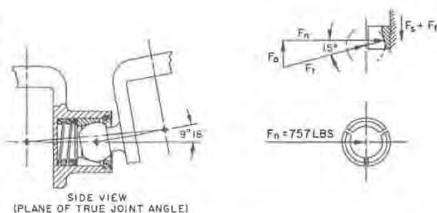
Fig. 12 — Centering mechanism with three segmented seats at WOT start condition load
