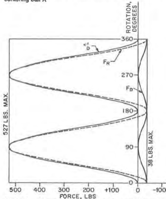
Fig. 6(b) — Harmonic characteristics of dynamic forces on centering ball X
