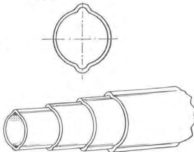
Fig. 24 — Grooved telescoping tubes
