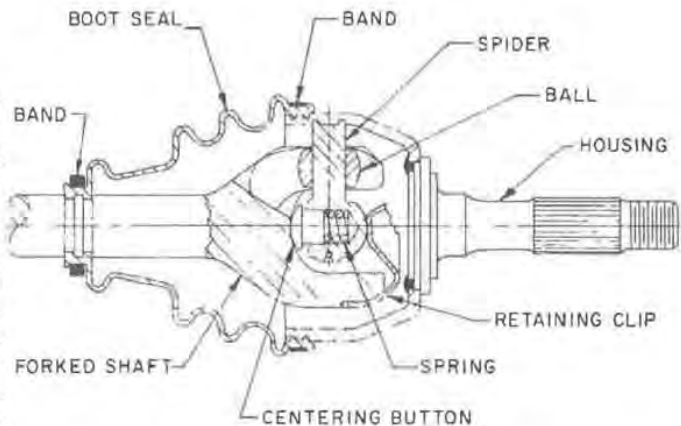
Fig. 1 — Tripot universal joint (fixed center type)
