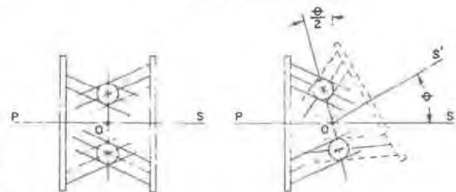
Fig. 2 — Diagram illustrating positioning of balls in bisecting angle plane
