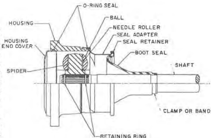
Fig. 1. — Tripot universal joint (end motion type)
