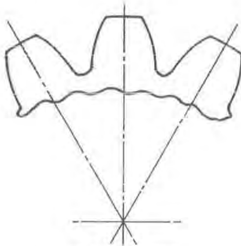
Fig. 1 — Involute spline
