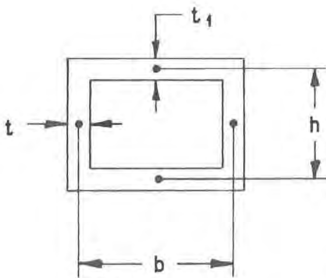
Fig. 1 — Rectangular tube
