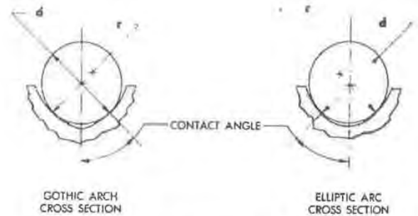
Fig. 19 — Typical ball spline ball groove forms
