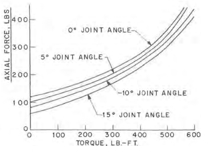
Fig. 7 — Cross groove joint axial force characteristics
