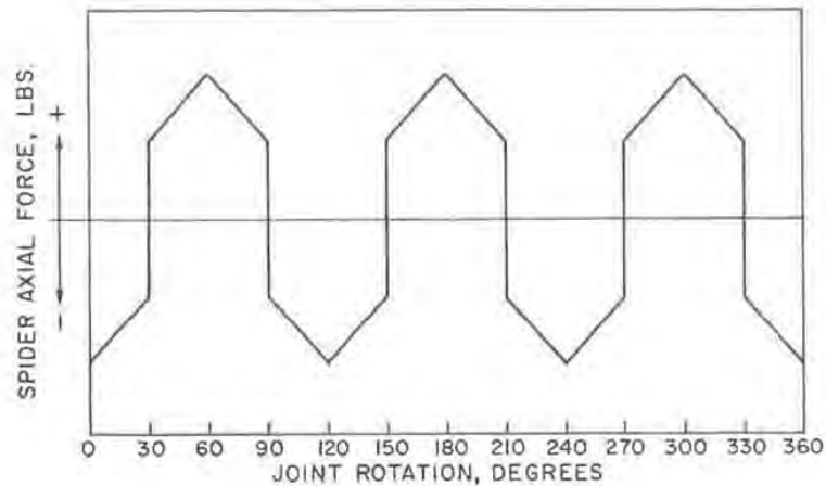
Fig. 7 — Typical theoretical dynamic end thrust
