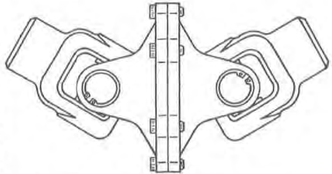
Fig. 1 — Double Cardan universal joint (twin ball and centering plate type)
