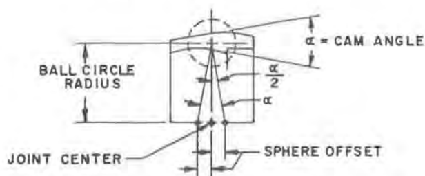
Fig. 5 — Diagram illustrating cam angle formed by cage offset spheres with respect to ball circle radius and joint center
