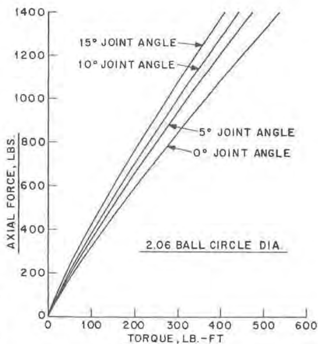
Fig. 7 — Double offset joint axial force characteristics
