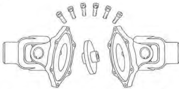
Fig. 2 — Partially disassembled twin ball and centering type of double Cardan universal joint
