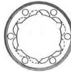
Fig. 4 — End view of typical cross groove joint outer race
