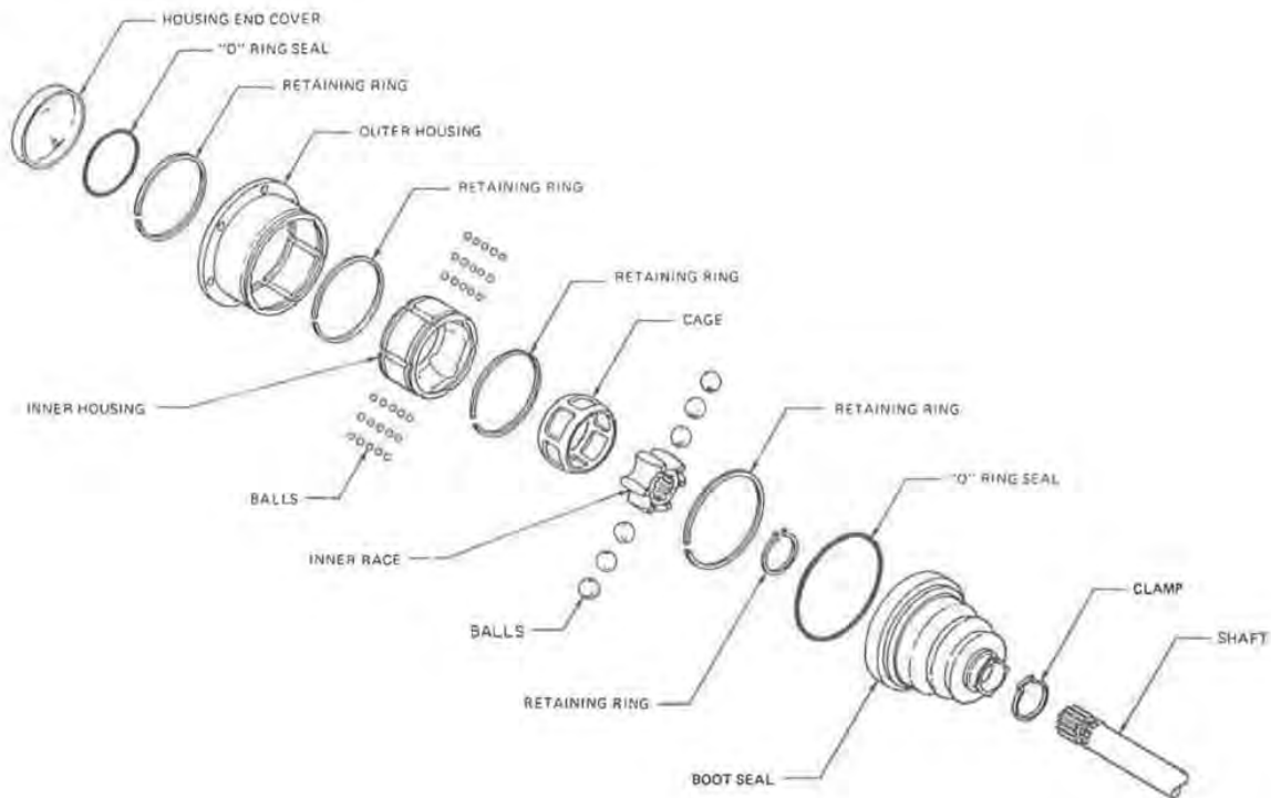
Fig. 2 — Ball spline Rzeppa universal joint
