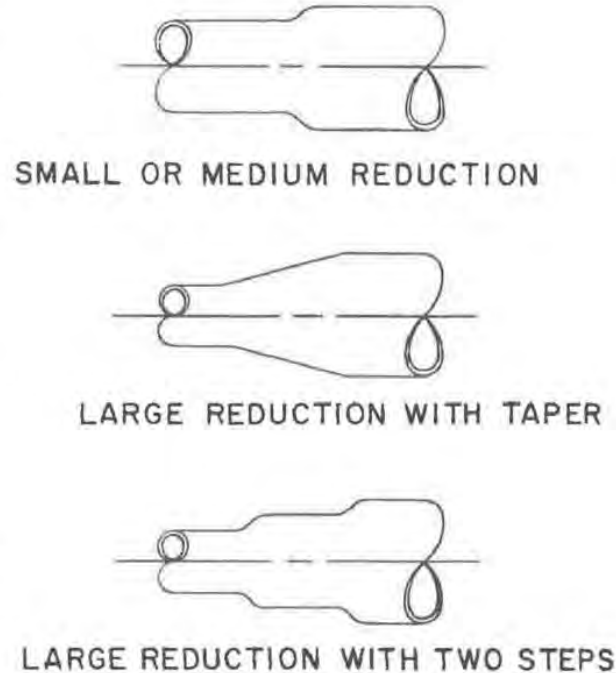
Fig. 3 — Typical swaging configurations
