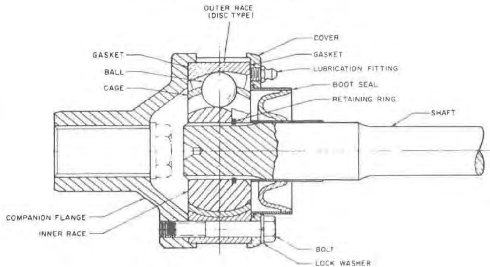
Fig. 8 — Rzeppa universal joint (disc type)
