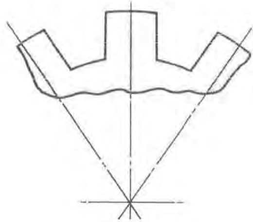
Fig. 2 — Parallel side spline
