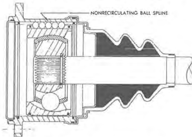
Fig. 17 — Ball spline Rzeppa universal joint
