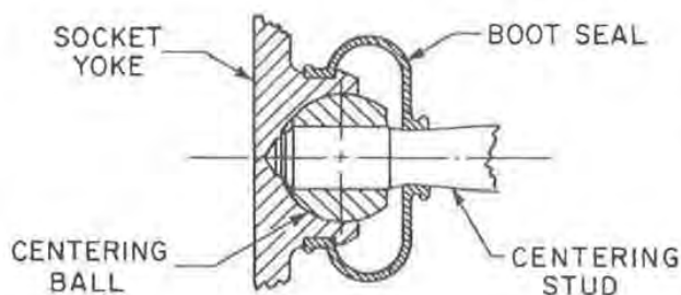
Fig. 9 — Centering ball and stud for axle driveshaft applications
