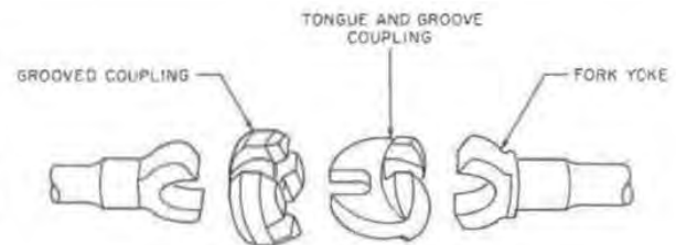
Fig. 3 — Tracta universal joint
