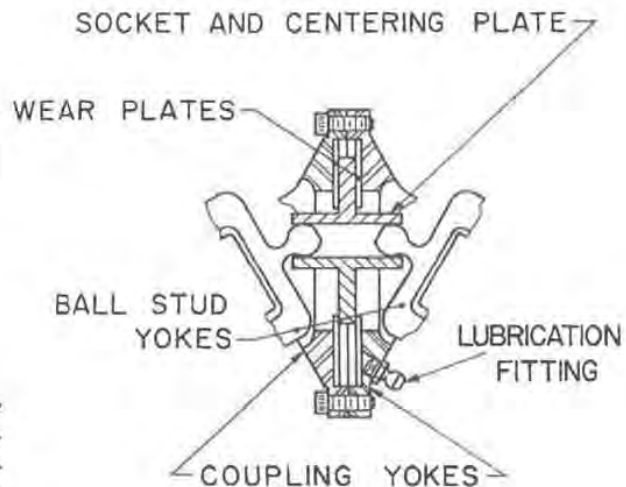
Fig. 3 — Centering device design
