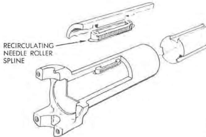
Fig. 16 — Slip yoke with recirculating needle roller spline
