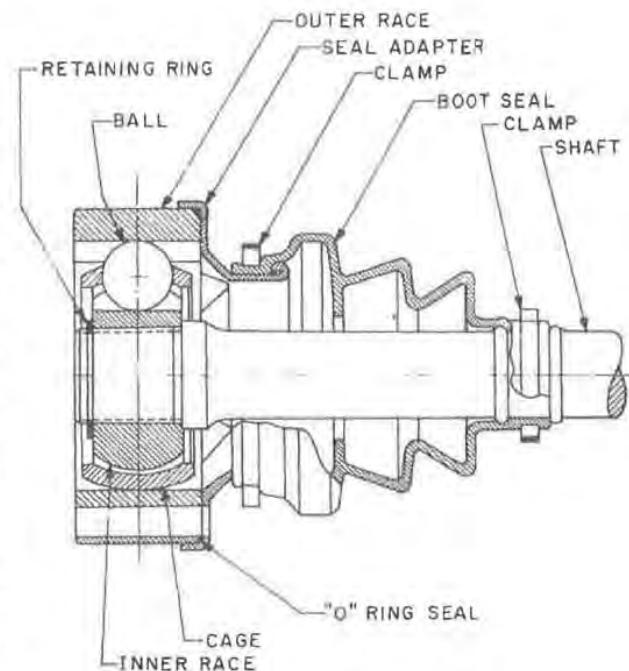
Fig. 1 — Cross groove universal joint
