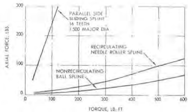
Fig. 20 — Comparison of rolling element spline axial force characteristics with a sliding spline
