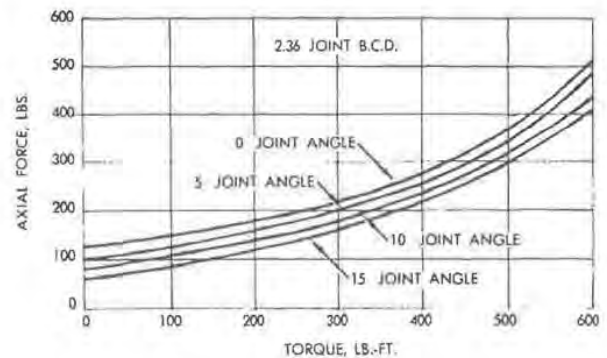
Fig. 30 — Cross groove joint axial force characteristics
