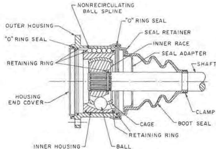
Fig. 1 — Ball spline Rzeppa universal joint
