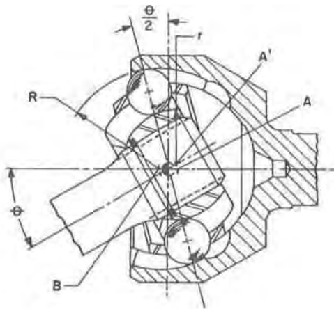
Fig. 2 — Rzeppa universal joint in angulated position
