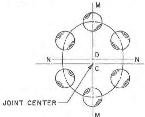
Fig. 5 — Section through plane of balls with joint in angulated position
