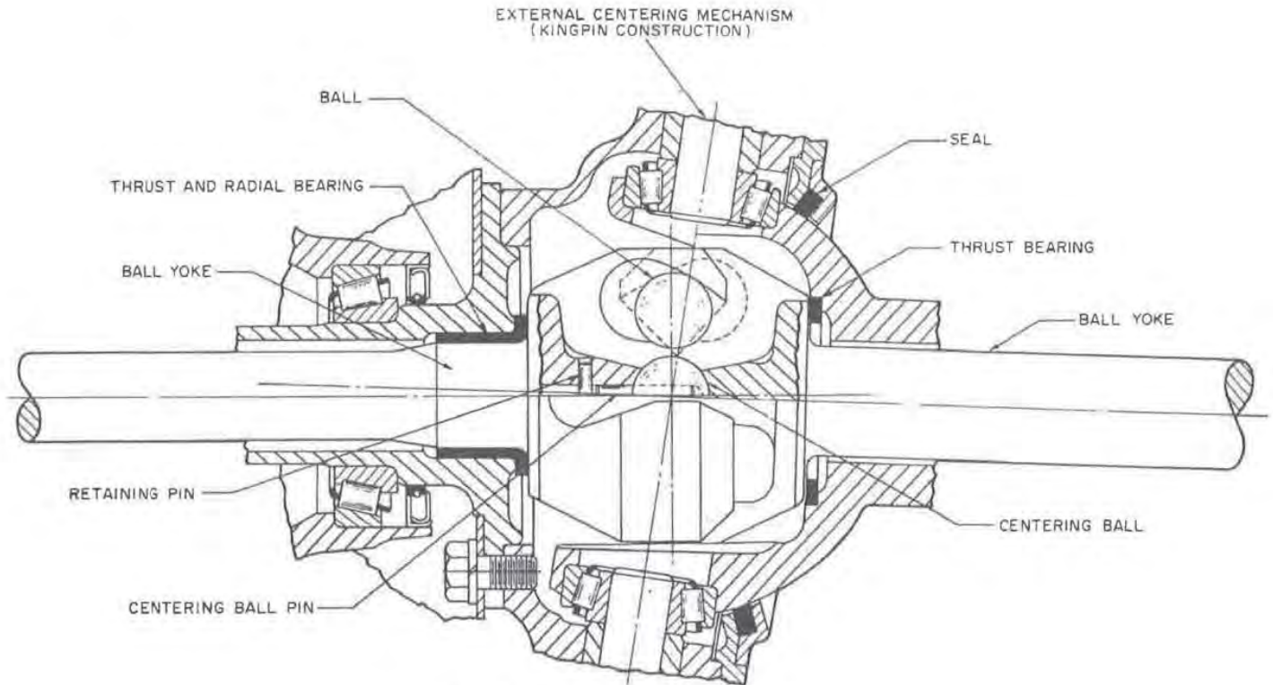
Fig. 1 — Weiss universal joint (fixed center type)
