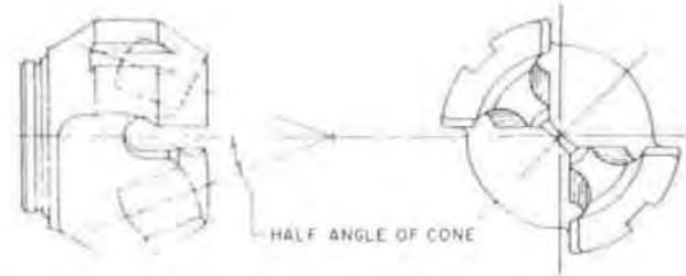
Fig. 4 — Ball yoke
