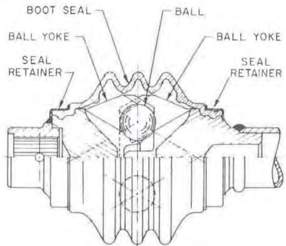
Fig. 1 — Weiss universal joint (end motion type)
