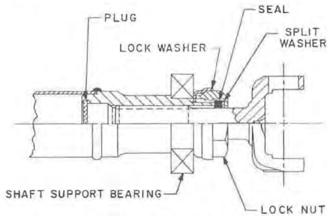
Fig. 12 — Seal design for external splined slip yoke
