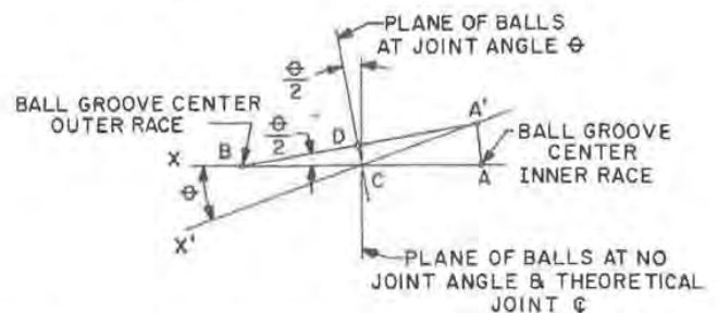
Fig. 4 — Diagram illustrating positioning of balls in bisecting angle plane
