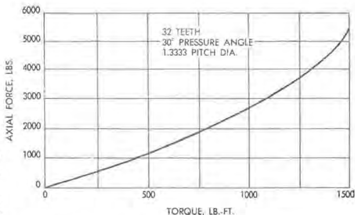
Fig. 3 — Involute sliding spline axial force characteristics
