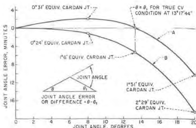
Fig. 7 — Difference in joint angles
