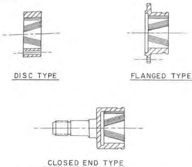
Fig. 3 — Typical cross groove joint outer race constructions
