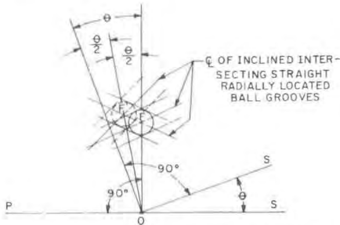
Fig. 3 — Diagram illustrating positioning of balls in bisecting angle plane
