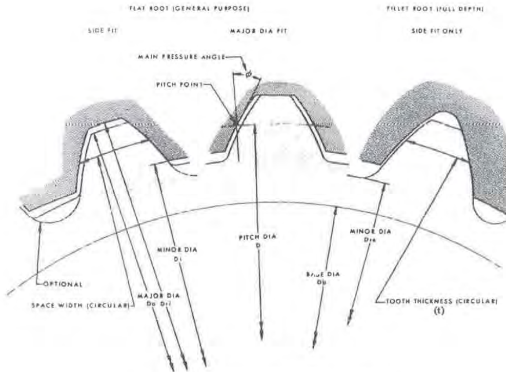
Fig. 5 — Spline nomenclature symbols and terms
