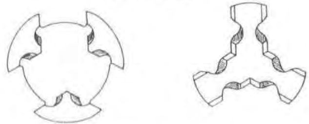
Fig. 5 — End view of ball yokes with parallel pairs of ball grooves
