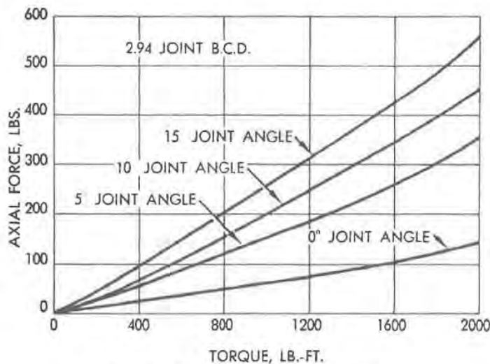
Fig. 28 — Tripot joint axial force characteristics
