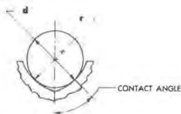
Fig. 5 — Cross section of elliptic arc ball groove
