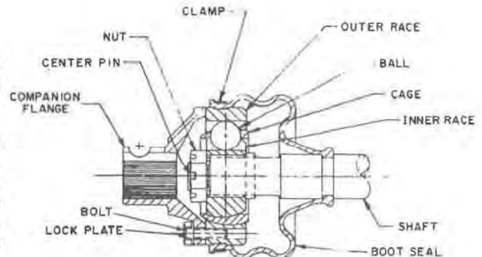
Fig. 1 — Double offset universal joint (fixed center type)
