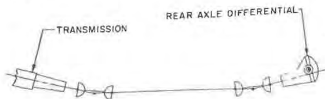
Fig. 4 — Schematic view of one piece driveline with double Cardan joints
