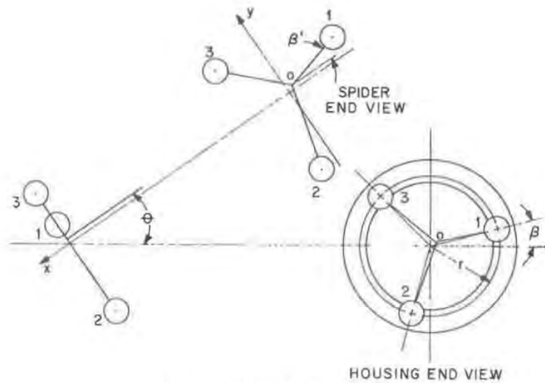
Fig. 2 — Triplot joint angular relationship
