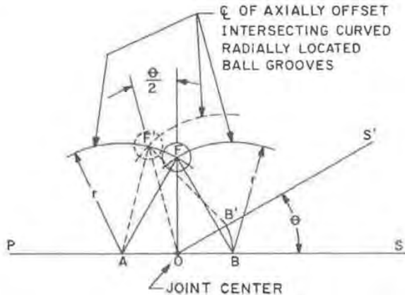
Fig. 2 — Diagram illustrating positioning of balls in bisecting angle plane
