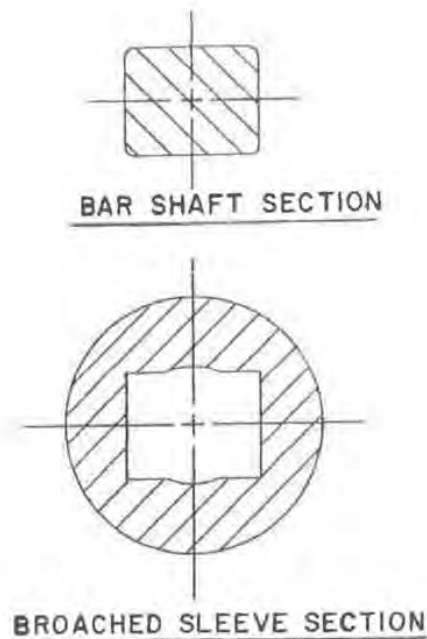
Fig. 21 — Typical rectangular section shaft telescoping components
