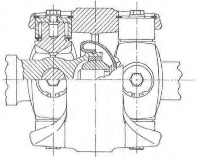
Fig. 1 — Double Cardan universal joint trunnion pin type
