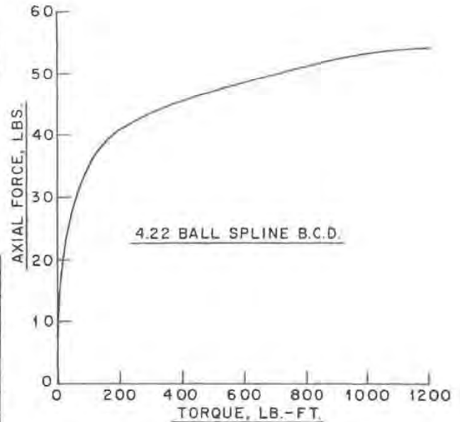
Fig. 27 — Ball spline Rzeppa joint axial force characteristics
