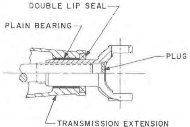
Fig. 9 — Conventional slip yoke sealing design at transmission output shaft
