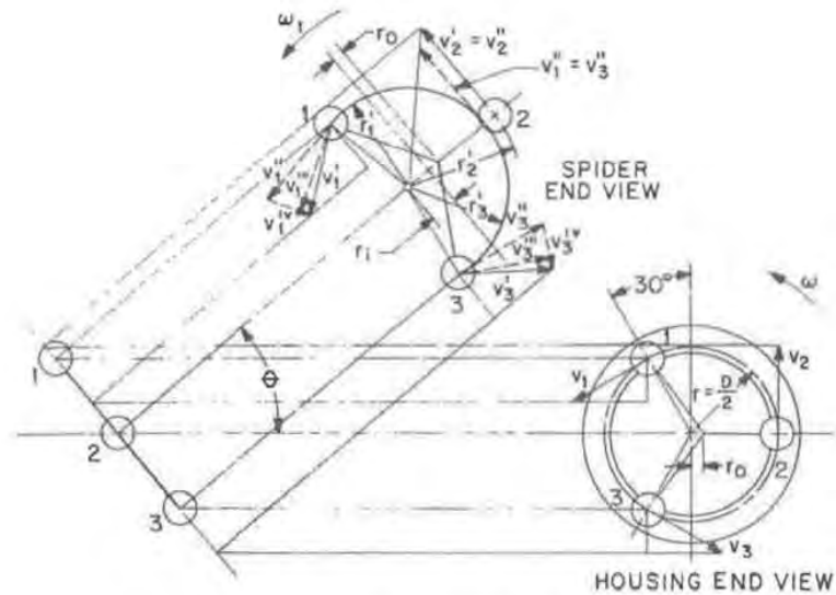
Fig. 4 — Motion analysis for rotational position (b)
