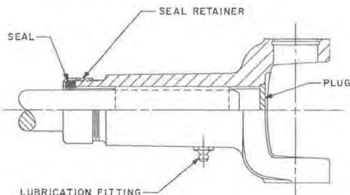
Fig. 11 — Slip yoke sealing design at hub end
