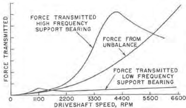
Fig. 3 — Typical shaft support bearing transmissibility characteristics
