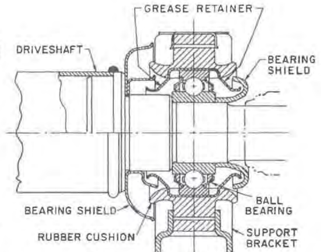
Fig. 2 — Typical truck shaft support bearing
