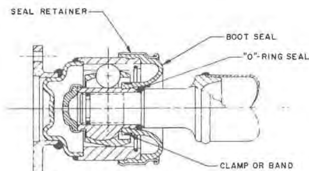
Fig. 6 — Boot seal configuration for high speed driveline application
