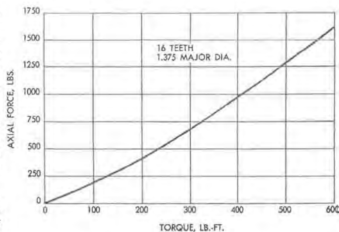
Fig. 4 — Parallel side sliding spline axial force characteristics
