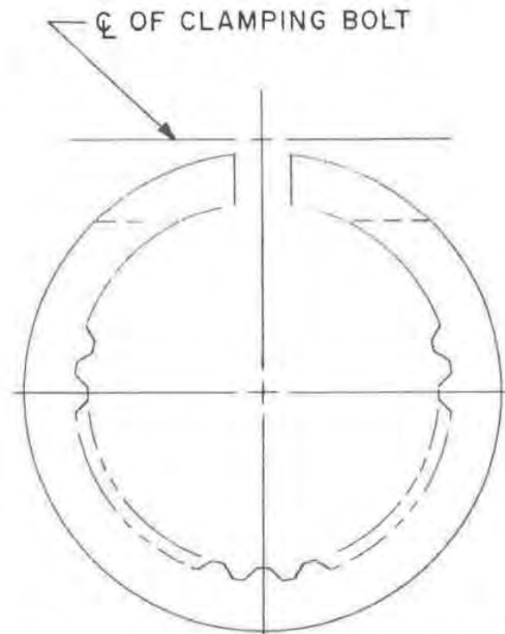
Fig. 14 — Hub end view of partial circle of internal truncated star serrations
