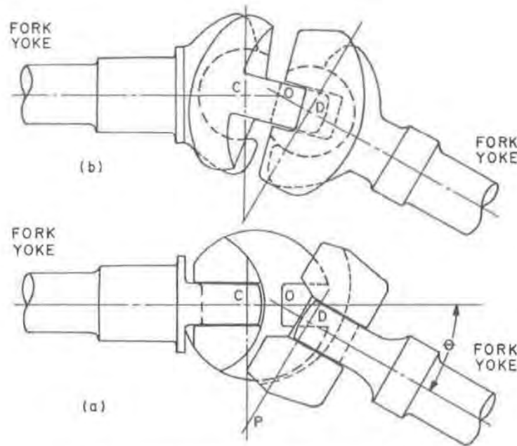
Fig. 2 — Tracta joint in two principal rotational positions 90 deg apart
