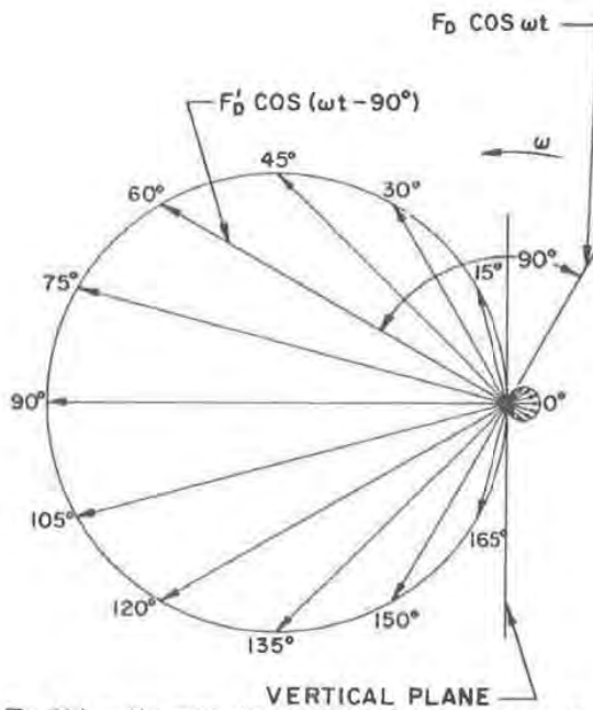
Fig. 6(a) — Harmonic characteristics of dynamic forces on centering ball X
