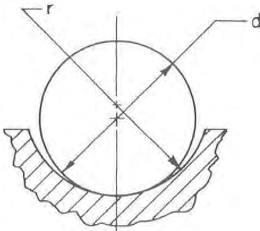
Fig. 2 — Cross section of circular arc ball groove
