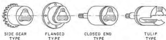
Fig. 9 — Typical tripot joint housing constructions
