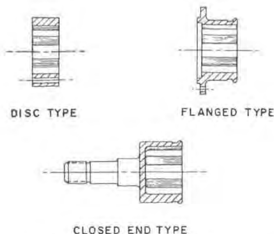
Fig. 3 — Typical double offset joint outer race constructions
