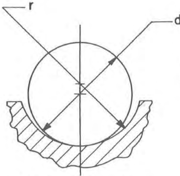
Fig. 6 — Cross section of circular arc ball groove
