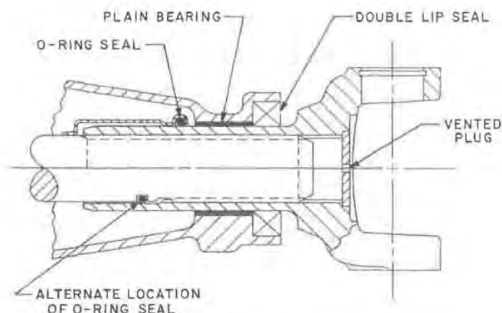
Fig. 10 — Alternate slip yoke sealing designs at transmission output shaft
