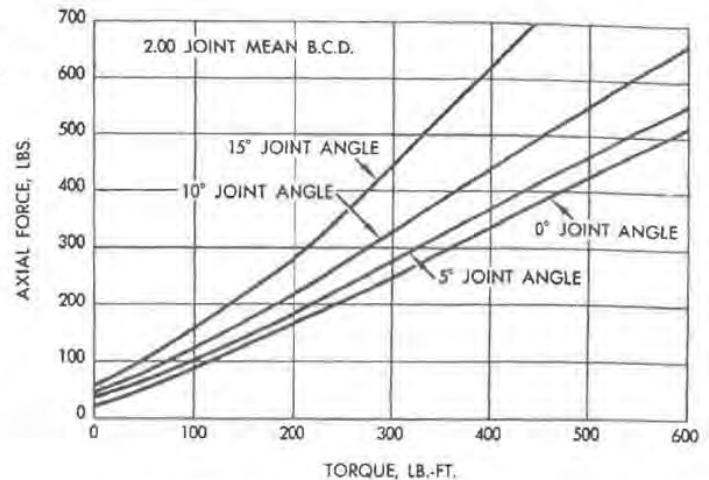
Fig. 7 — Weiss joint axial force characteristics
