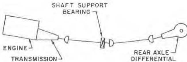
Fig. 1 — Schematic view of two piece driveline with shaft support bearing
