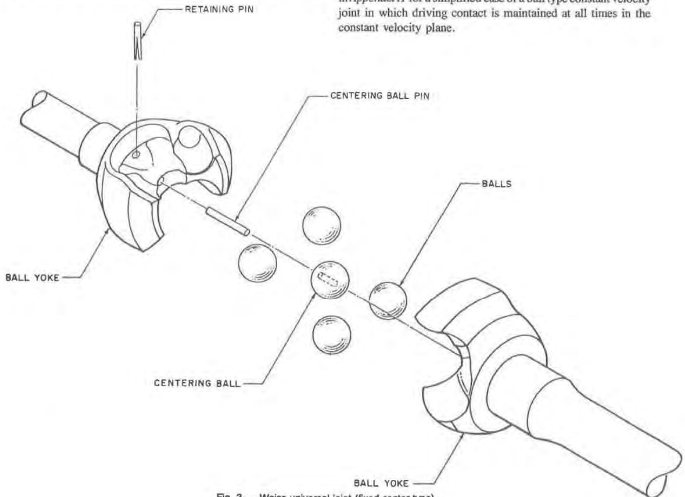
Fig. 3 — Weiss universal joint (fixed center type)
