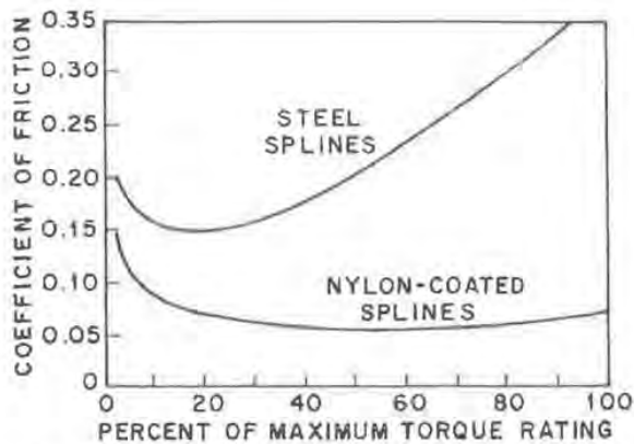
Fig. 7 — Comparison of coefficient of friction versus torque between lubricated steel and nylon coated splines
