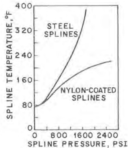
Fig. 8 — Comparison of spline temperature versus spline pressure between steel and nylon coated splines
