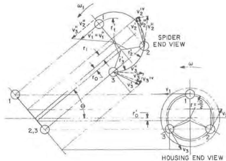
Fig. 3 — Motion analysis for rotational position (a)
