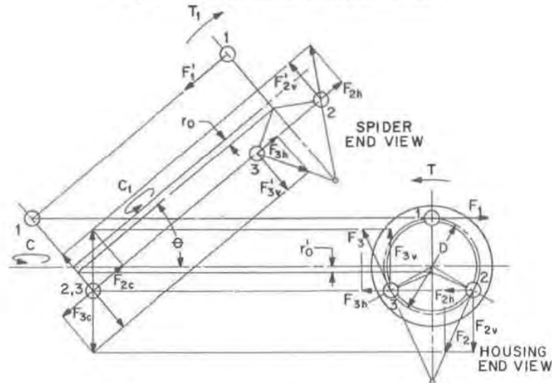
Fig. 5 — Force analysis for rotational position (a)
