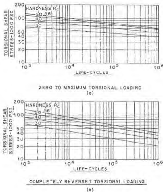
Fig. 6 — S-N curves for spline
