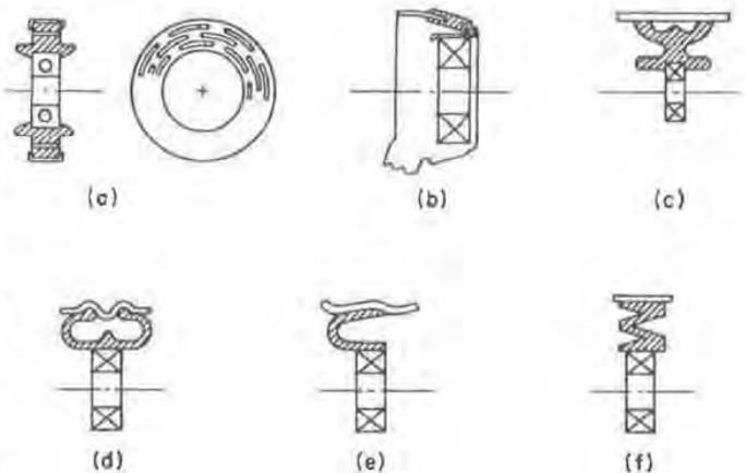
Fig. 4 — Typical shaft support bearing configurations
