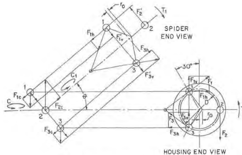
Fig. 6 — Force analysis for rotational position (b)
