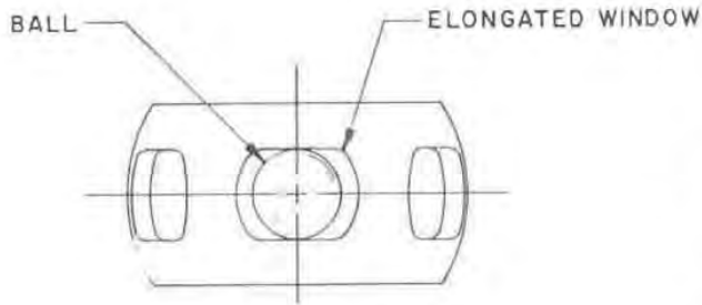
Fig. 6 — Elongated cage windows
