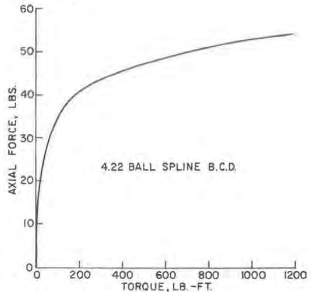
Fig. 3 — Ball spline Rzeppa joint axial force characteristics
