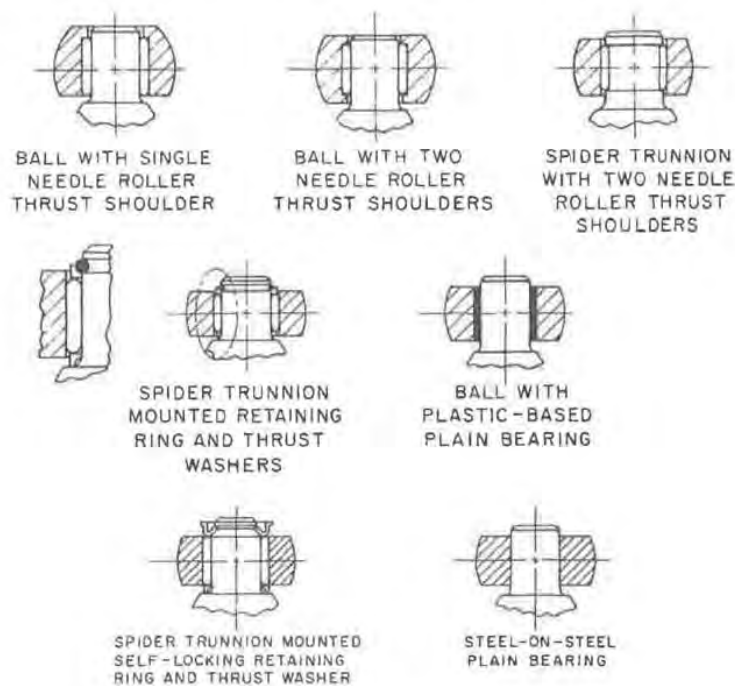
Fig. 10 — Typical tripot joint bearing constructions
