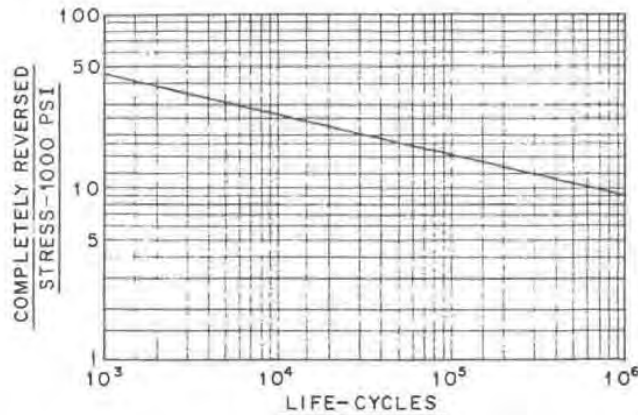
Fig. 2 — S-N curve for round welded steel tubing
