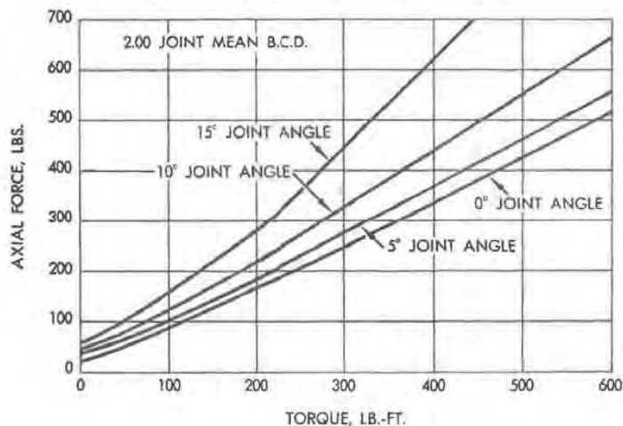
Fig. 29 — Weiss joint axial force characteristics
