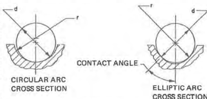
Fig. 11 — Typical ball groove forms
