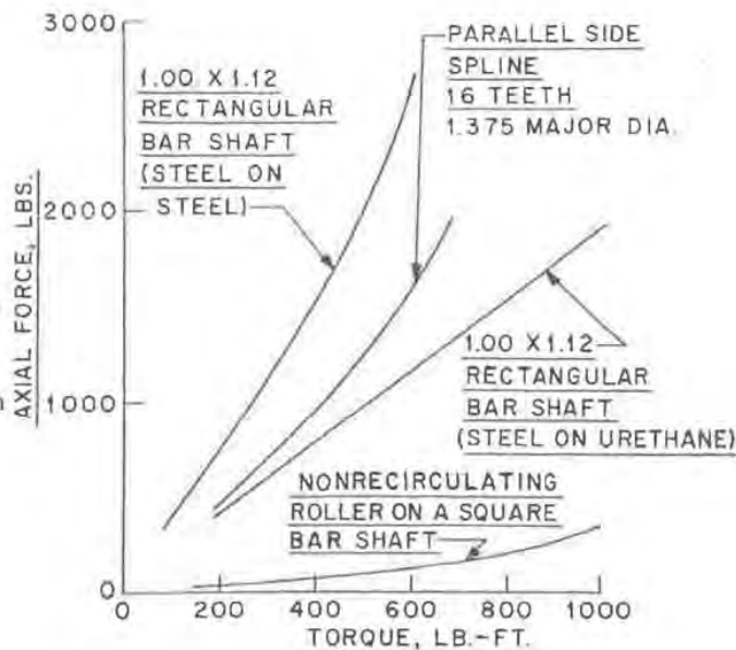
Fig. 23 — Comparison of axial force characteristics of typical agricultural implement telescoping devices with a conventional sliding spline
