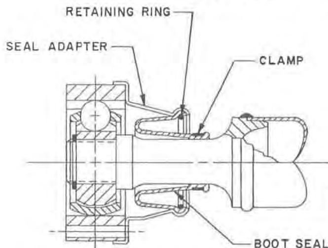
Fig. 6 — Boot seal configuration for high speed driveline application
