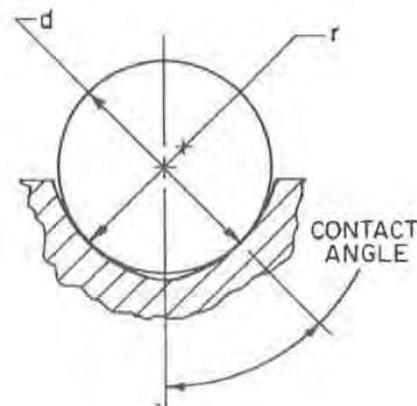
Fig. 4 — Cross section of elliptic arc ball groove
