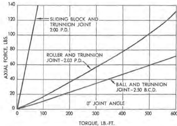
Fig. 26 — Axial force characteristics of end motion type non-constant velocity joints
