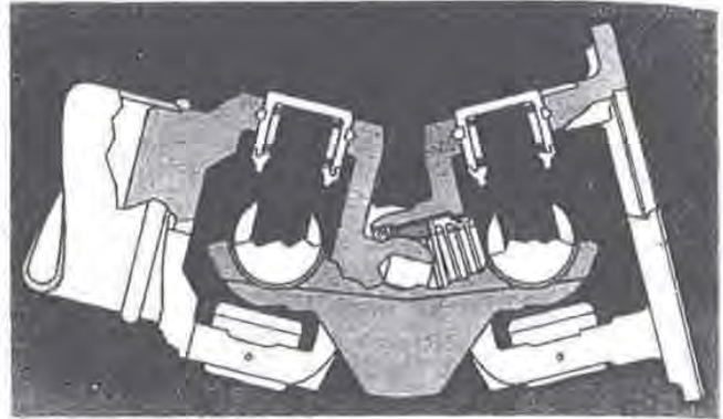
Fig. 13 — Double Cardan joint with angulation stops
