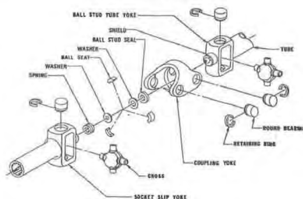
Fig. 8 — Double Cardan universal joint
