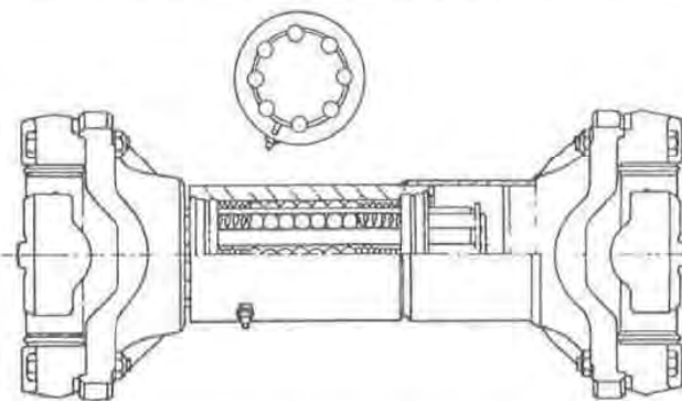
Fig. 18 — Nonrecirculating ball spline with spring return feature in a driveshaft
