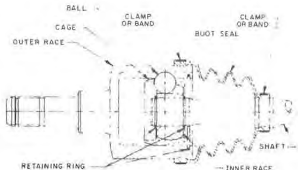
Fig. 1 — Double offset universal joint (end motion type)
