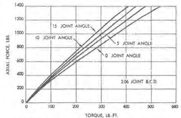
Fig. 31 — Double offset joint axial force characteristics
