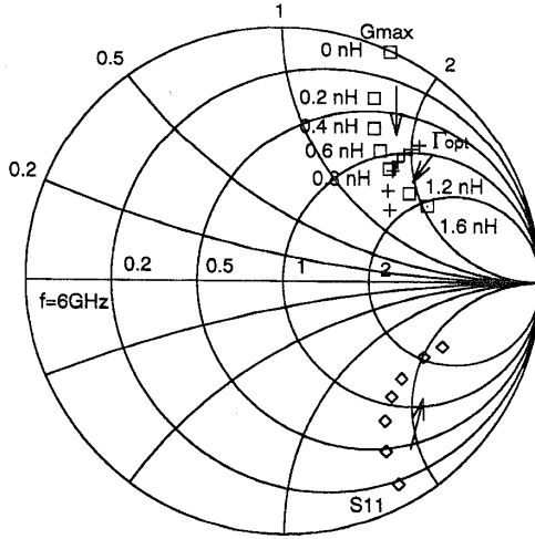
Fig. 5. Impedance mapping of \Gamma_{opt} , G_{max} , and S_{11} of cascode inductive series feedback (CCSF) versus the feedback inductance at 6 GHz. The load resistance is 400 \Omega . The device is 0.5 \mu\text{m} \times 300 \mu\text{m} GaAs MESFET. Note that the simultaneous noise and input power matching is obtained with 0.8 nH series feedback.
