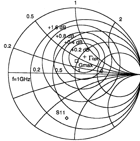
Fig. 3. Constant noise figure circles and G_{max} of cascode resistive parallel feedback (CCPF) for 4 \text{ k}\Omega feedback resistor and 1.7 \text{ k}\Omega load resistor at 1 GHz. The device is \text{nnp} BJT with emitter area 20 \mu\text{m} \times 6 \mu\text{m} from 0.8 \mu\text{m} BiCMOS process.
