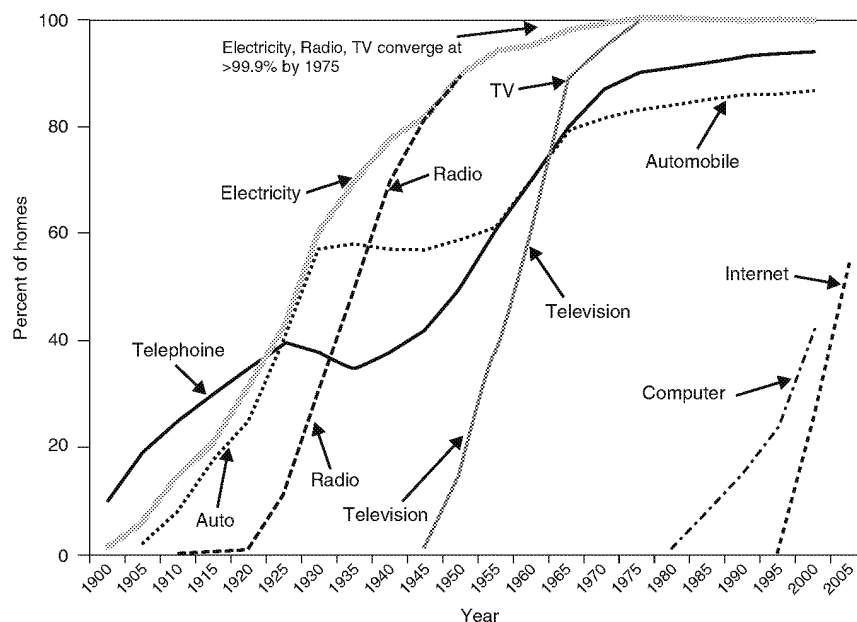
FIGURE 8 Penetration of New Technologies in U.S. Homes, 1900-2005.
