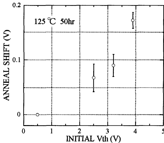
Fig. 10 Electric field dependence of anneal shift Initial V_t is V_t just after programming. The chip is then baked 50hr at 125°C.
