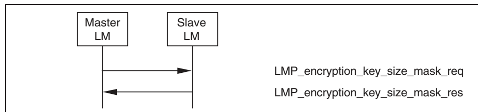
Sequence 42: Request for supported encryption key sizes.
