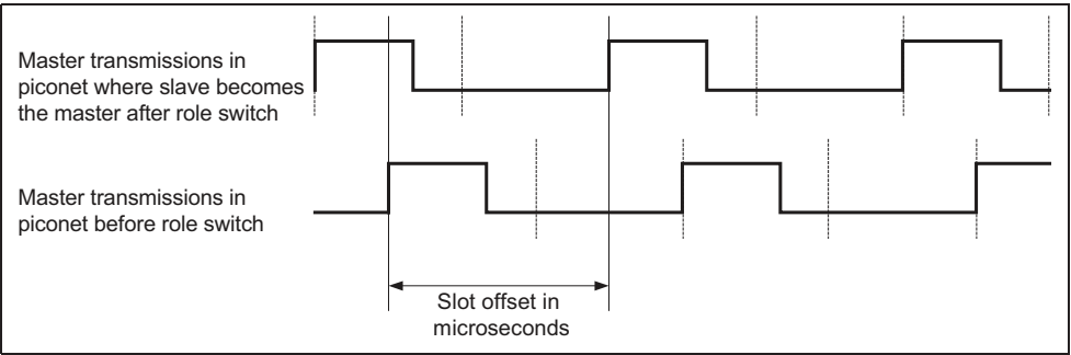
Figure 4.3: Slot offset for role switch
