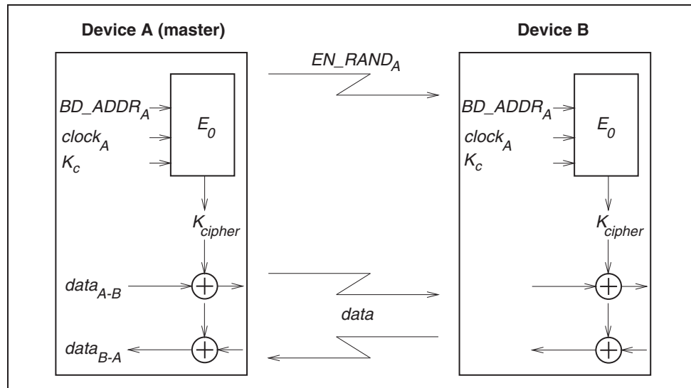
Figure 4.2: Functional description of the encryption procedure
