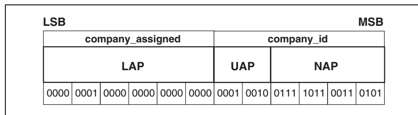
Figure 1.5: Format of BD_ADDR.
