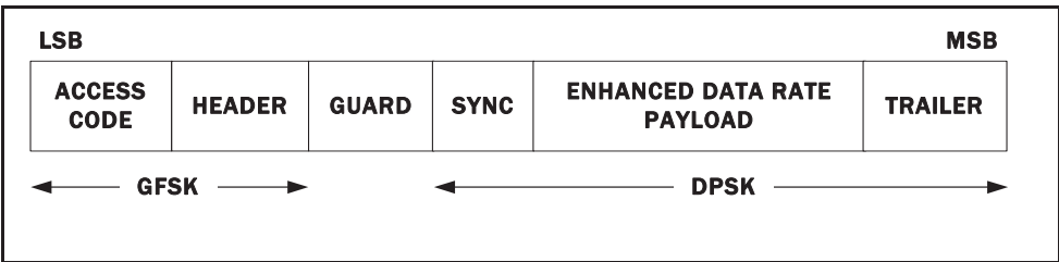
Figure 6.2: General enhanced data rate packet format
