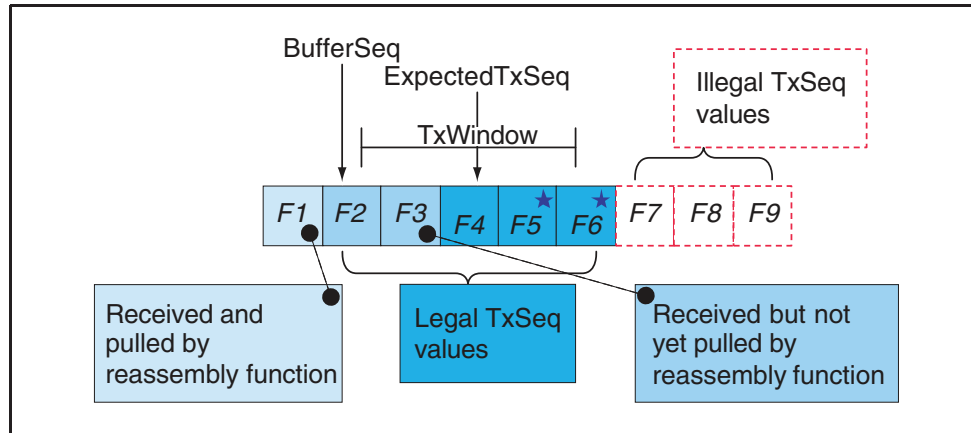
Figure 8.2: Example of the receiver side
