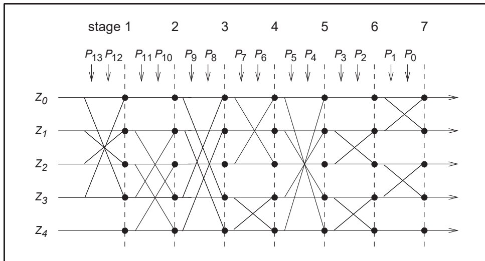
Figure 2.18: Permutation operation for the hop system.
