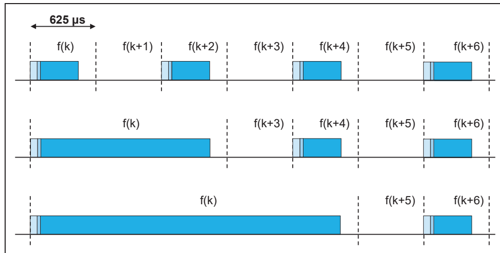
Figure 2.14: Single- and multi-slot packets.
