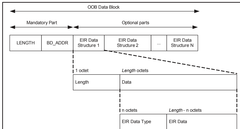
Figure 5.6: OOB Data Block Format
