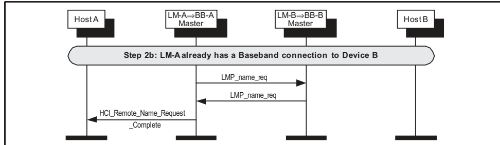
Figure 2.3: Remote name request with baseband connection.
