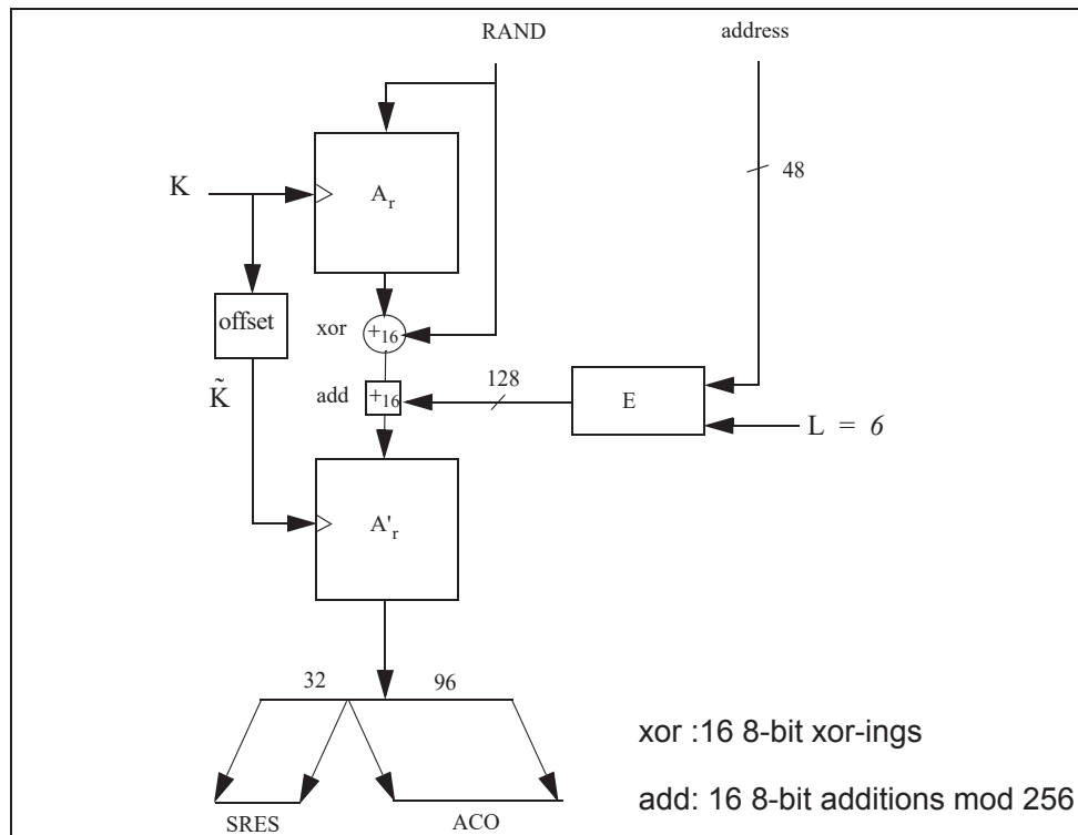
Figure 6.1: Flow of data for the computation of E_I .
