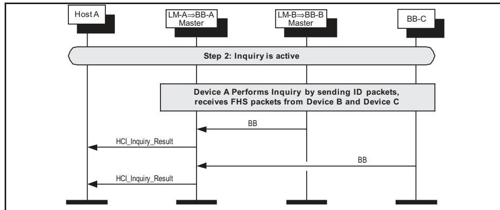
Figure 2.5: LM-A performs inquiry and reports result.
