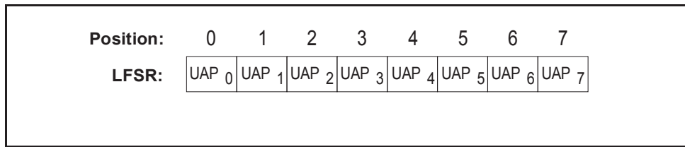
Figure 7.4: Initial state of the HEC generating circuit.
