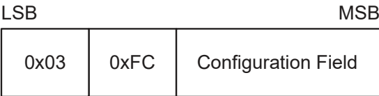
Figure 8.4: Configuration Message Format
