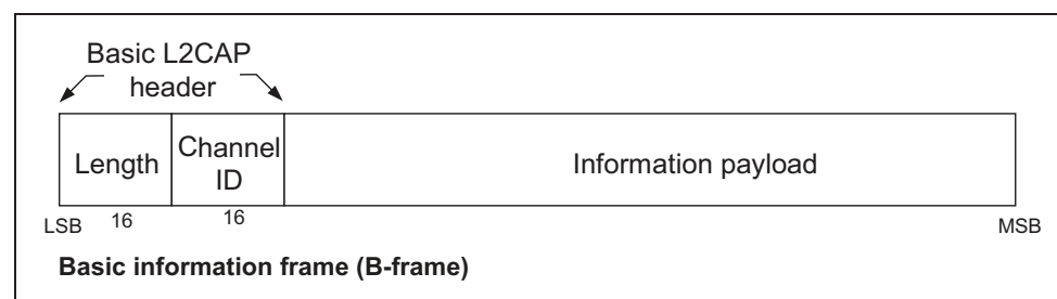
Figure 3.1: PDU format in Basic L2CAP mode on connection-oriented channels (field sizes in bits)
