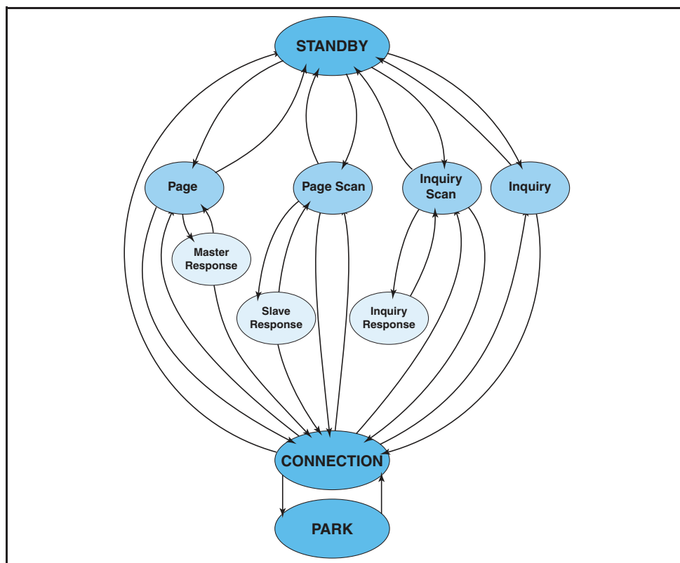
Figure 8.1: State diagram of link controller.
