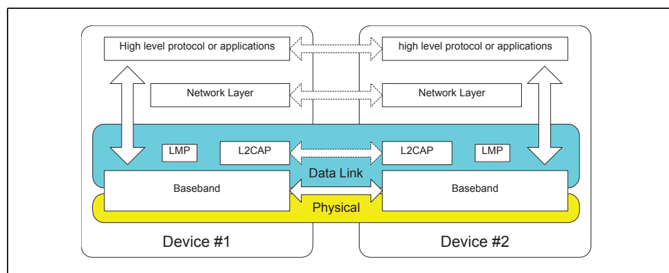
Figure 1.1: L2CAP within protocol layers
