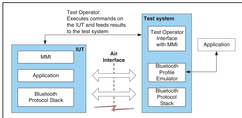
Figure 2.2: General test set-up for profile qualification
