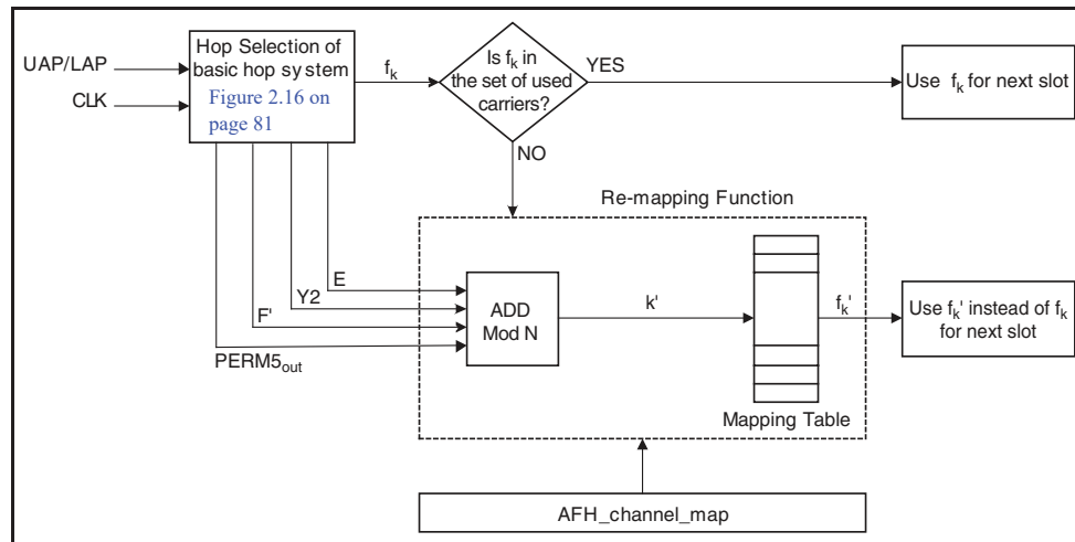
Figure 2.20: Block diagram of adaptive hop selection mechanism
