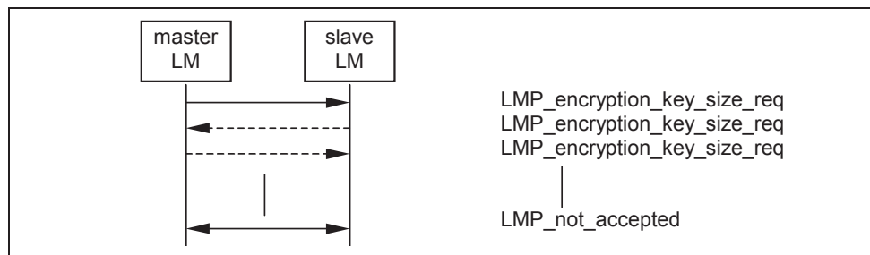
Sequence 35: Encryption key size negotiation failed
