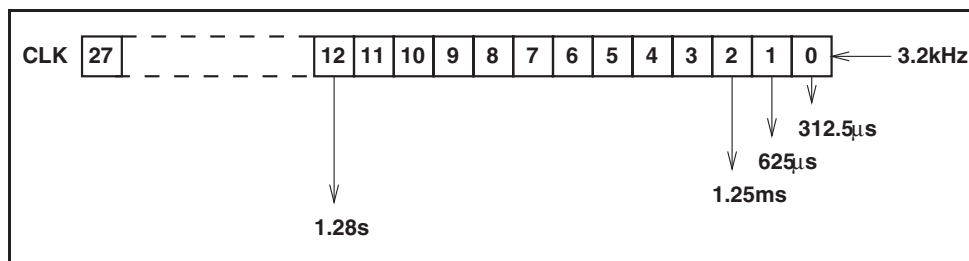
Figure 1.4: Bluetooth clock.
