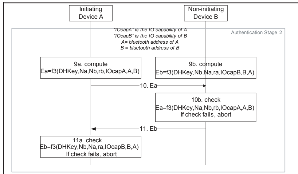
Figure 7.7: Authentication Stage 2
