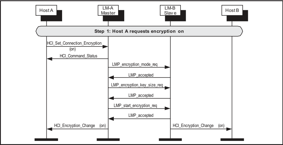
Figure 4.23: Encryption requested.
