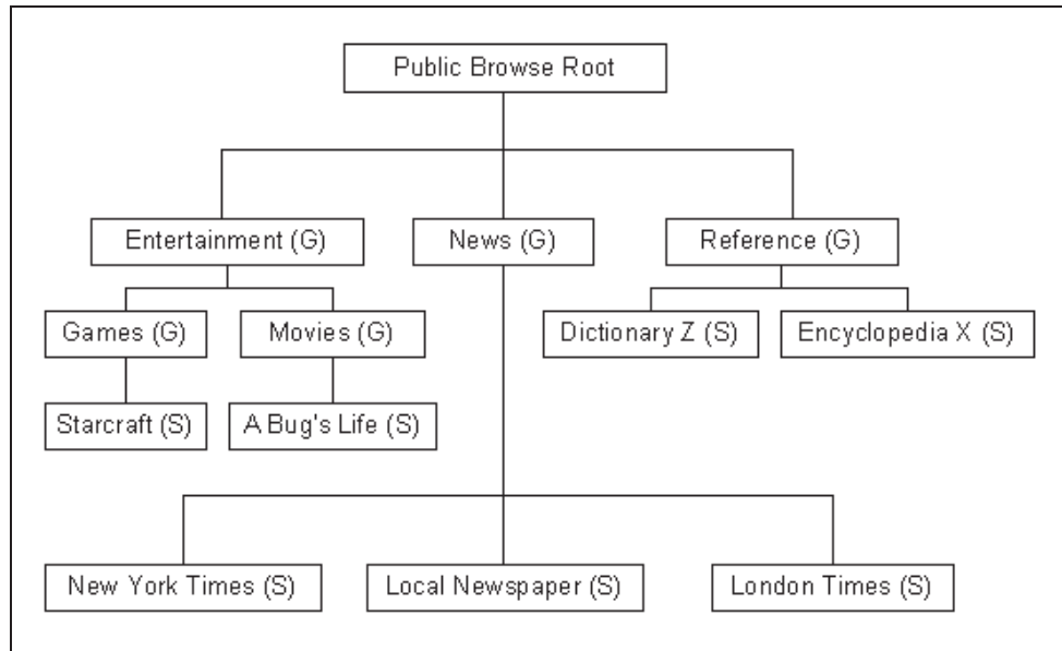
Figure 2.5:
