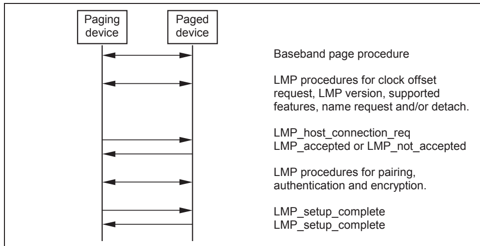
Figure 4.1: Connection establishment.
