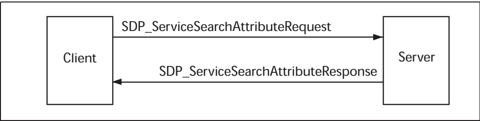
Figure 4.6:
