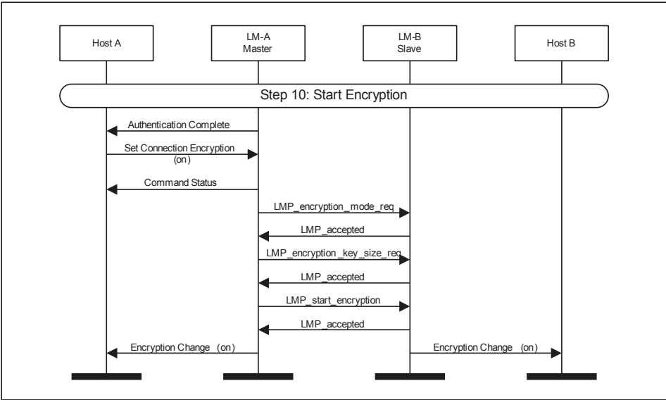
Figure 4.20: Start Encryption
