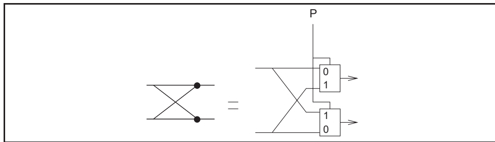
Figure 2.19: Butterfly implementation.
