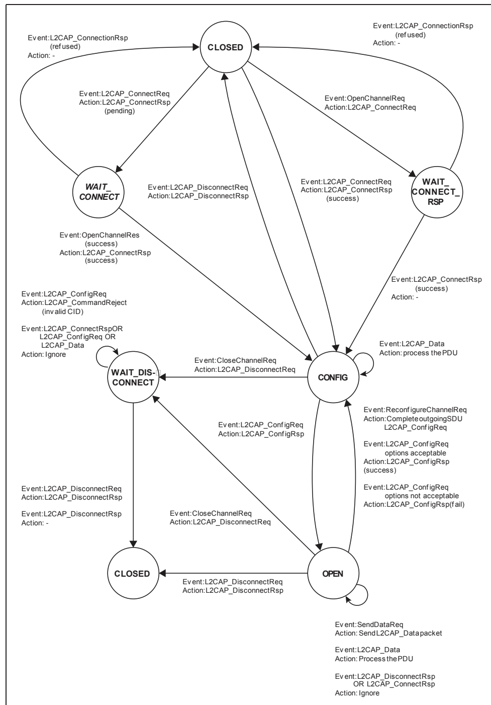
Figure 6.1: States and transitions.
