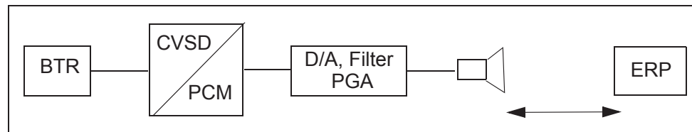
Figure 11.2: RLR measurement set-up.
