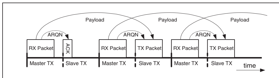
Figure 1.8: Payload & ARQN handling in delayed loopback - start.
