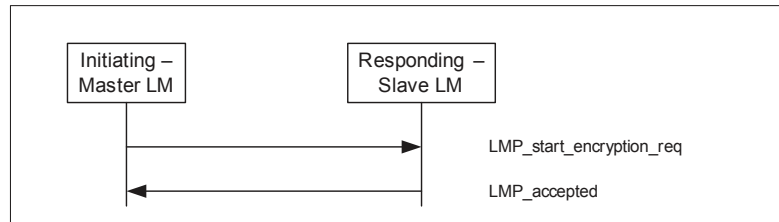
Sequence 40: Initiating Master LM resumes encryption
