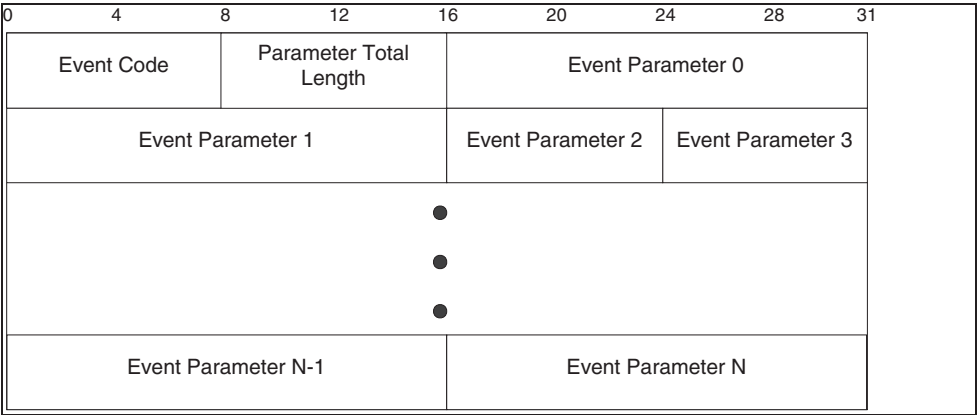
Figure 5.4: HCI Event Packet
