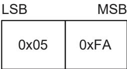
Figure 9.1: Wakeup Message Payload Format
