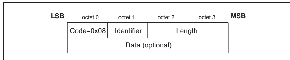
Figure 4.12: Echo Request Packet
