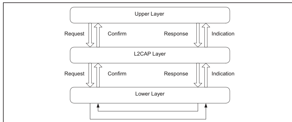
Figure 2.2: L2CAP transaction model.
