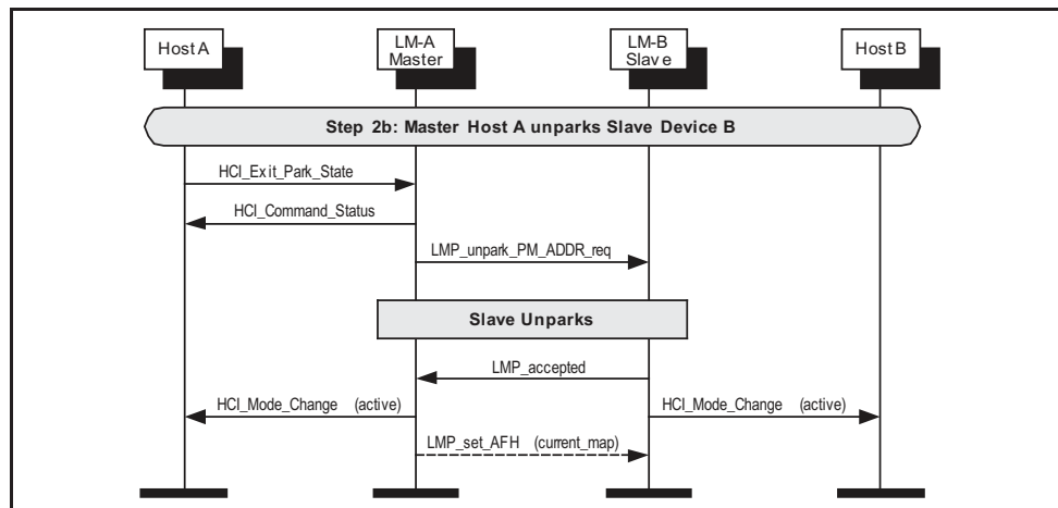
Figure 6.10: Master exits park state with slave.
