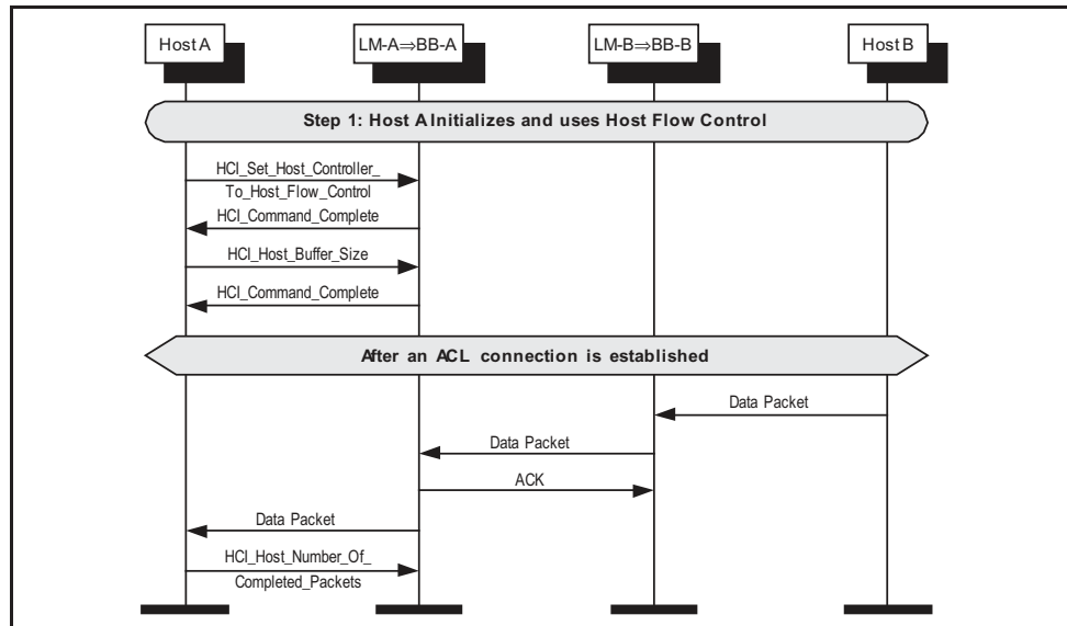
Figure 7.2: Controller to Host flow control.
