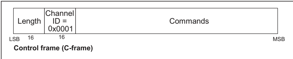
Figure 4.1: L2CAP PDU format on the signaling channel
