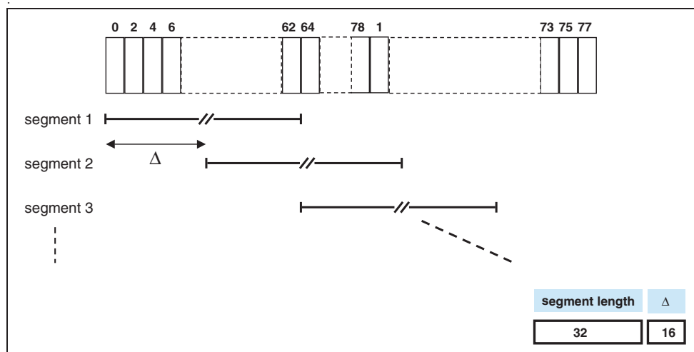
Figure 2.13: Hop selection scheme in CONNECTION state.
