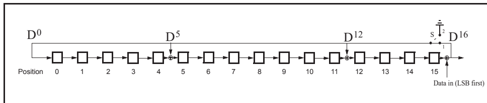
Figure 7.6: The LFSR circuit generating the CRC.
