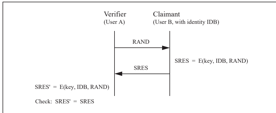
Figure 5.2: Challenge-response for symmetric key systems.
