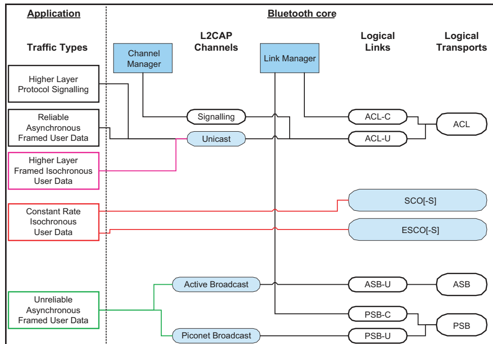
Figure 3.2: Bluetooth traffic bearers
