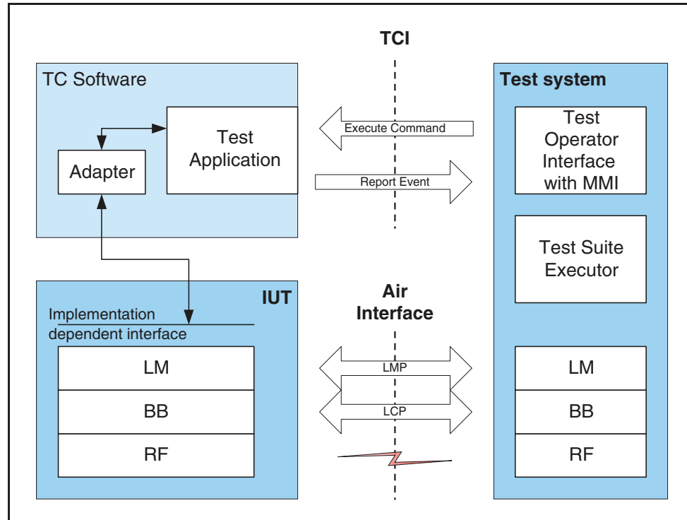
Figure 2.4: BB and LM qualification with “software bearer”
