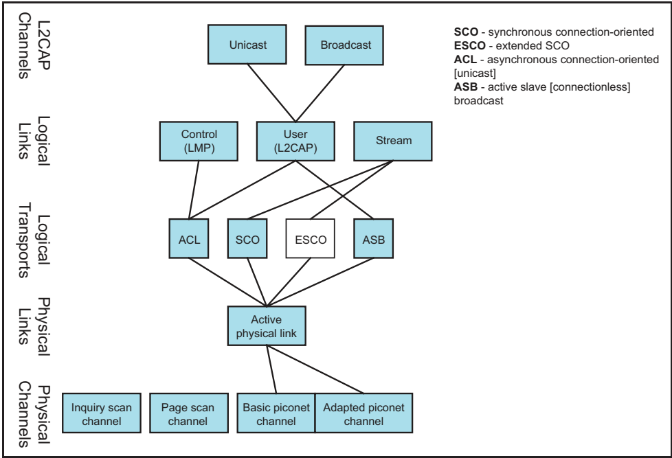
Figure 3.3: Overview of transport architecture entities and hierarchy
