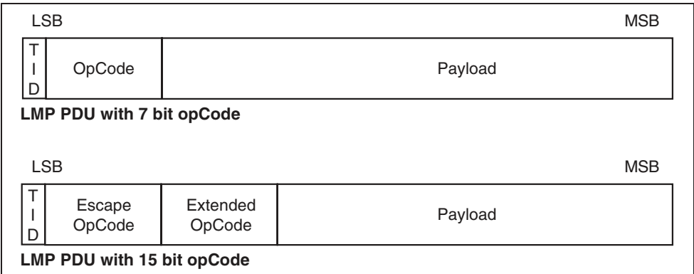
Figure 2.2: Payload body when LMP PDUs are sent.
