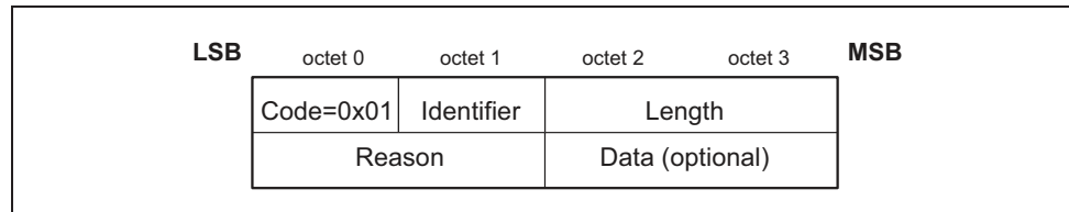
Figure 4.3: Command Reject packet
