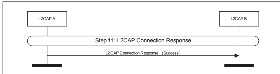
Figure 4.21: L2CAP Connection Response
