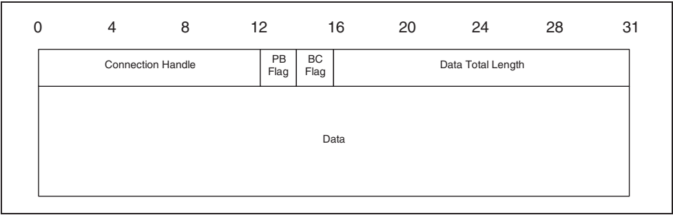
Figure 5.2: HCI ACL Data Packet
