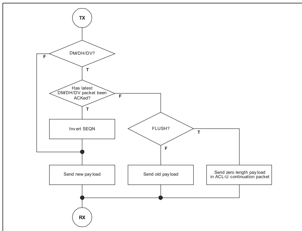
Figure 7.15: Transmit filtering for packets with CRC.
