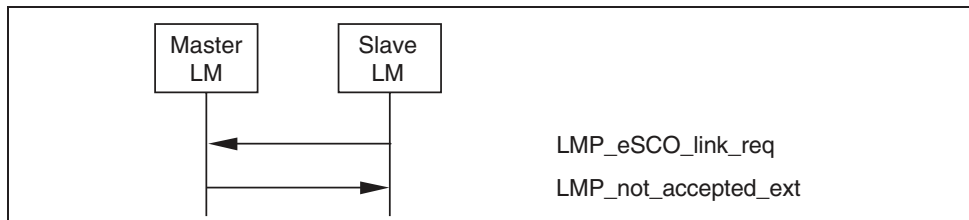
Sequence 95: Master rejects slave's request for an eSCO link.
