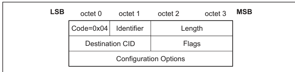
Figure 4.6: Configuration Request Packet
