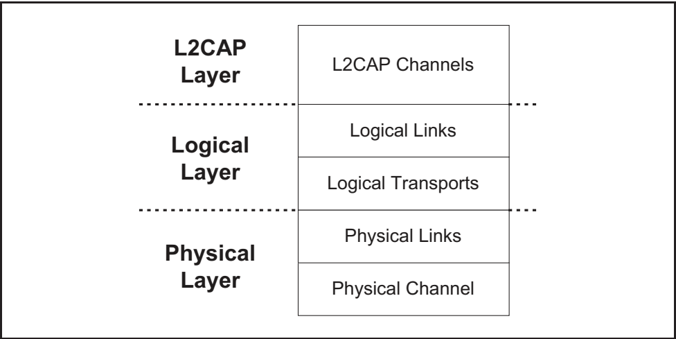
Figure 3.1: Bluetooth generic data transport architecture
