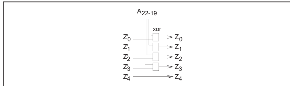
Figure 2.17: XOR operation for the hop system.
