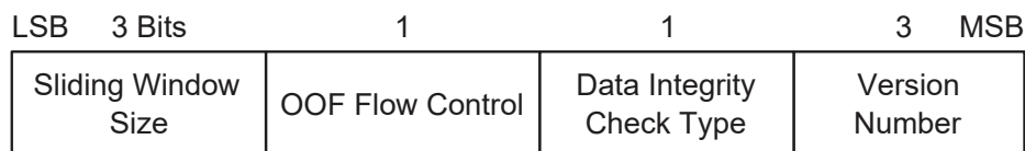
Figure 8.6: Configuration Field Detail
