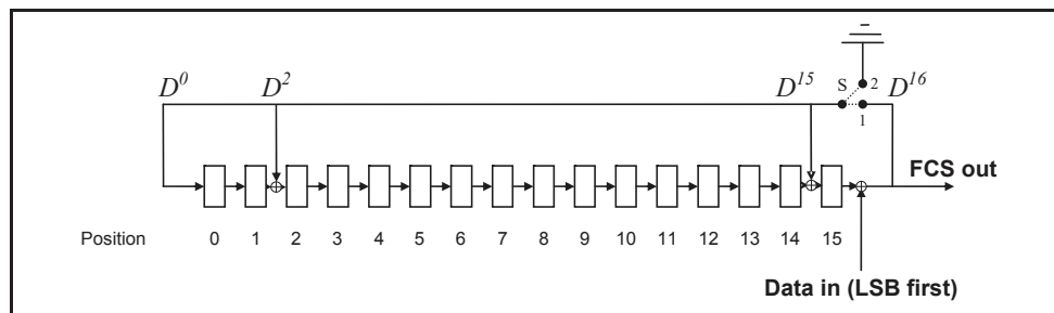
Figure 3.4: The LFSR circuit generating the FCS.
