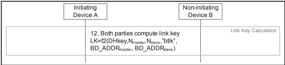
Figure 7.8: Link Key Calculation
