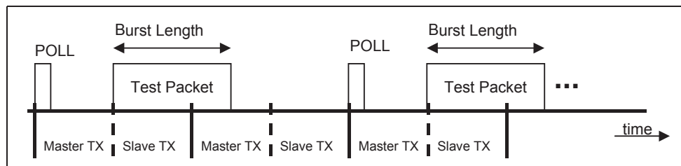
Figure 1.2: Timing for Transmitter Test
