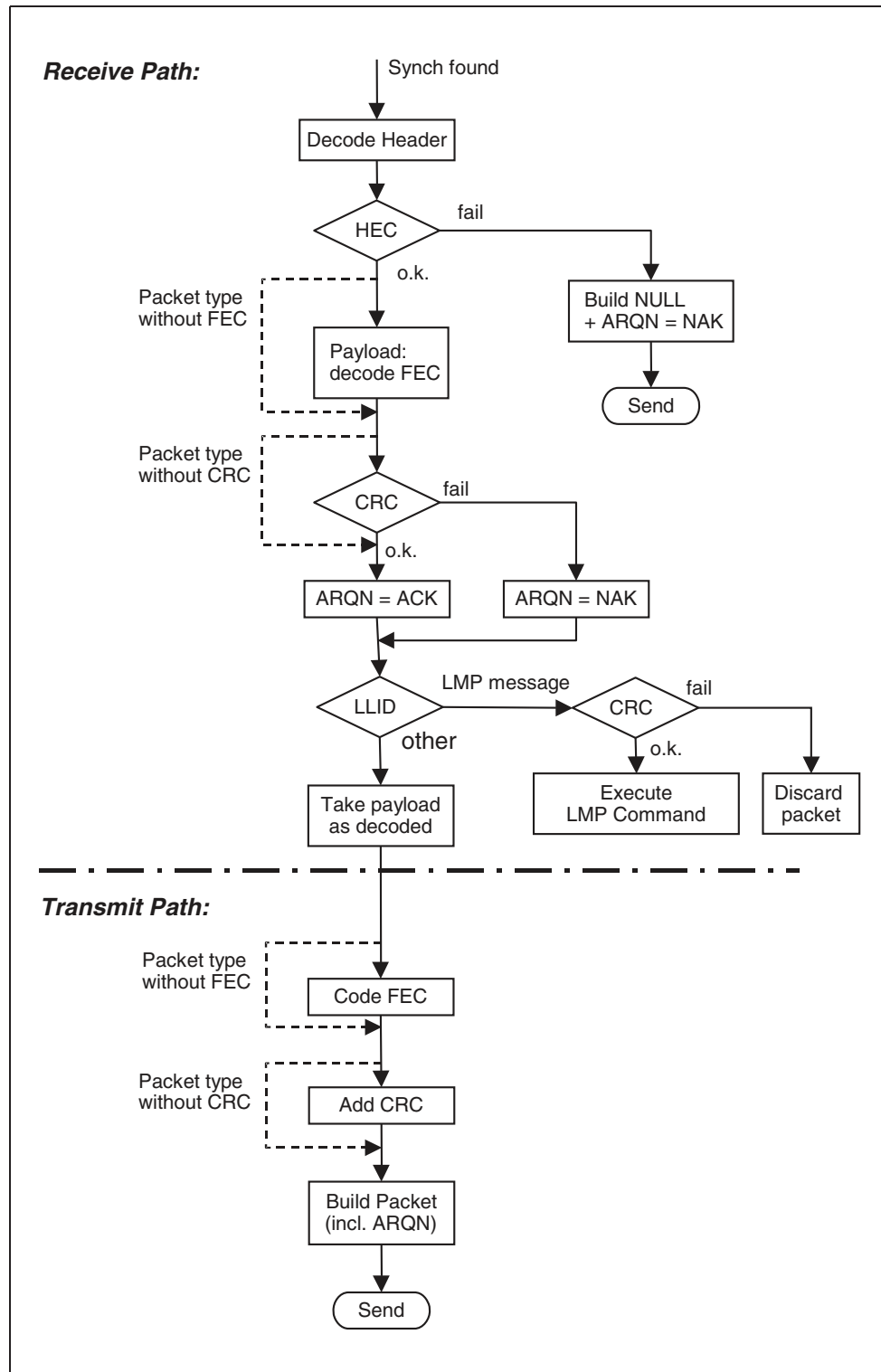
Figure 1.6: DUT Packet Handling in Loop Back Test
