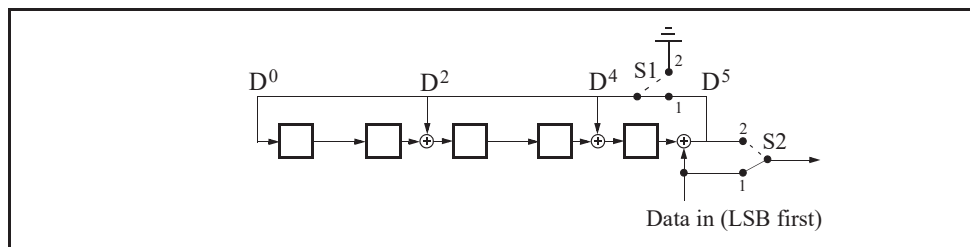
Figure 7.11: LFSR generating the (15,10) shortened Hamming code.
