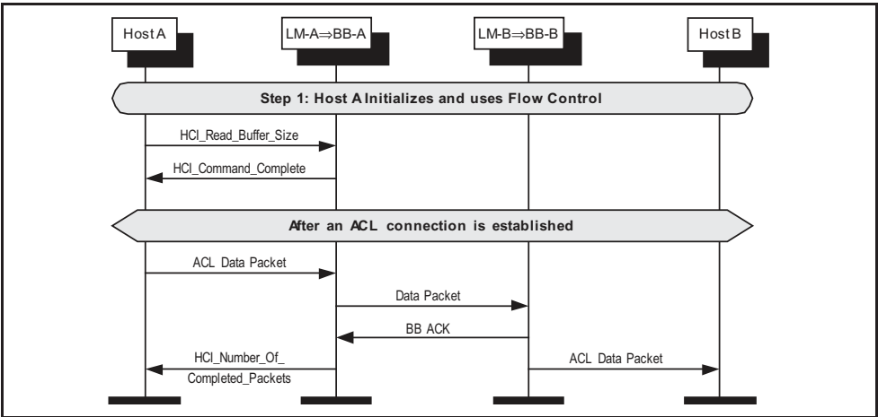
Figure 7.1: Host to Controller flow control.
