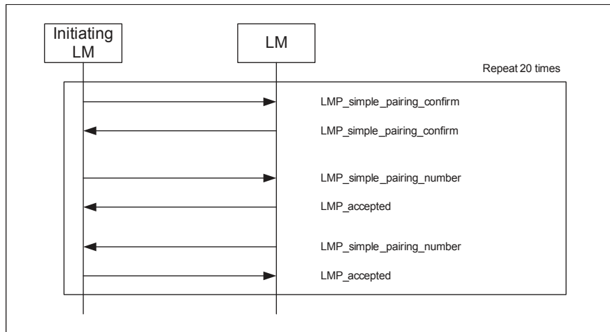
Sequence 51: Authentication Passkey entry
