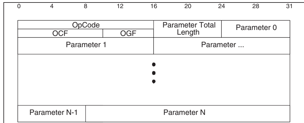
Figure 5.1: HCI Command Packet
