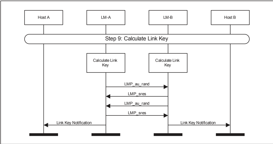
Figure 4.19: Calculate Link Key
