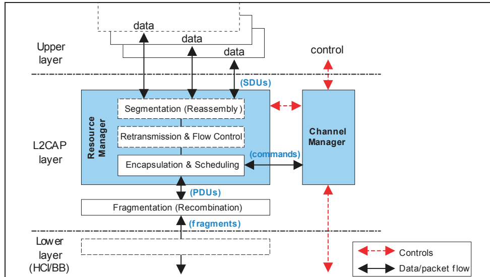
Figure 1.2: L2CAP architectural blocks
