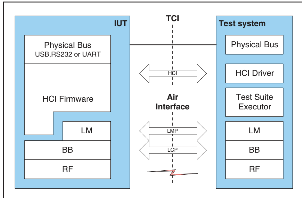
Figure 2.5: General test set-up for HCI qualification
