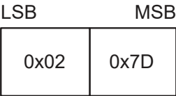
Figure 8.3: Sync Response Message Format
