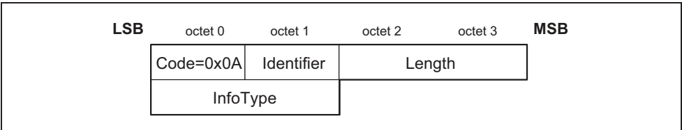
Figure 4.14: Information Request Packet
