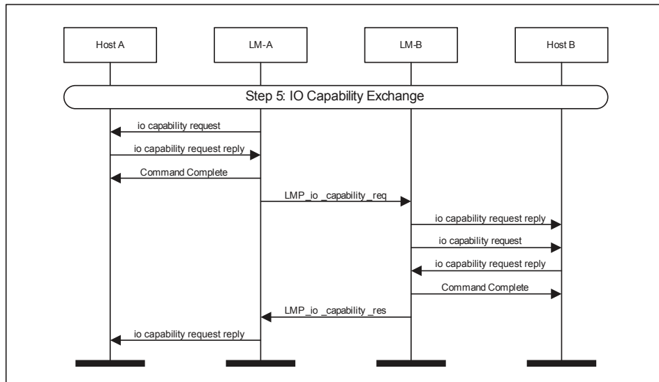
Figure 4.8: IO Capability Exchange
