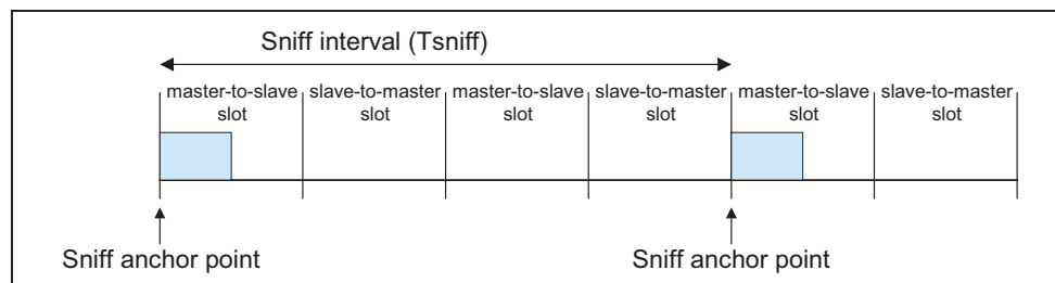
Figure 8.12: Sniff anchor points
