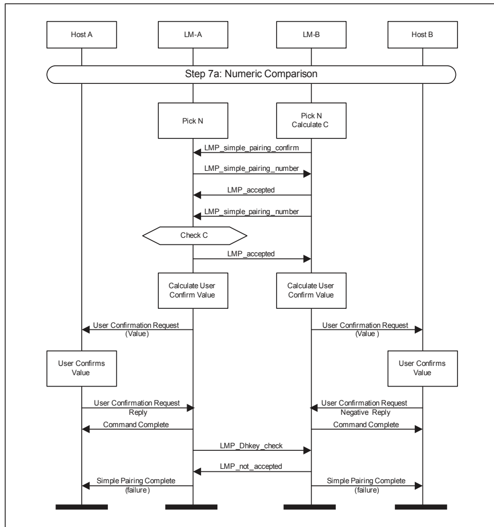
Figure 4.12: Numeric Comparison Failure on Responding Side
