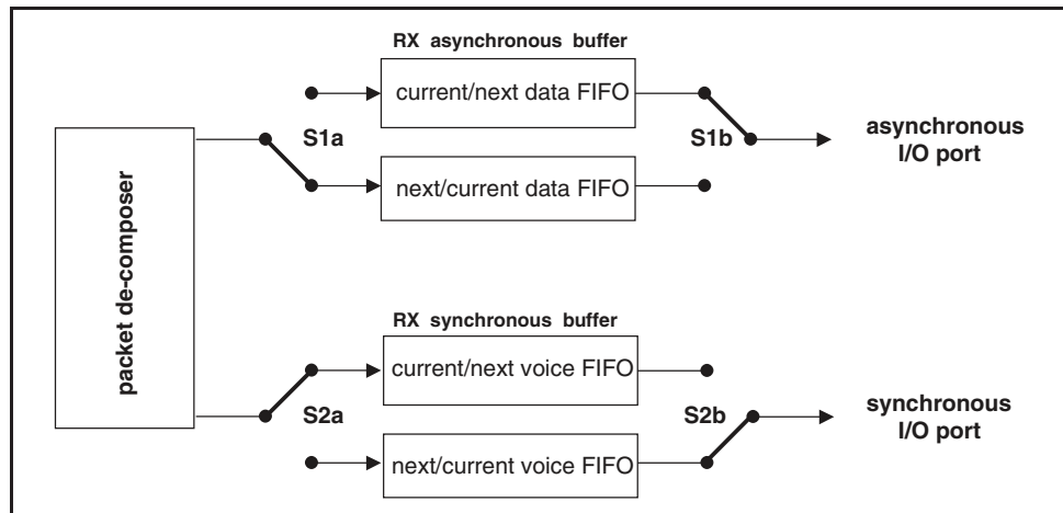
Figure 4.2: Functional diagram of RX buffering
