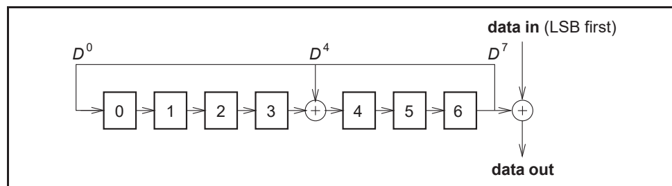
Figure 7.9: Data whitening LFSR.
