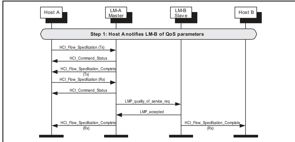
Figure 4.35: QoS flow specification.
