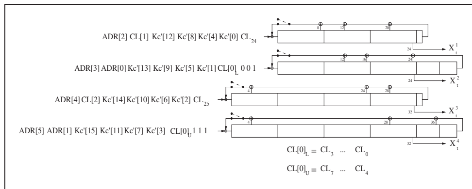
Figure 4.5: Arranging the input to the LFSRs.
