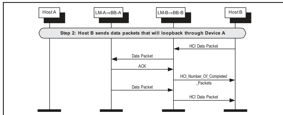
Figure 8.6: Looping back data in Remote Loopback Mode.
