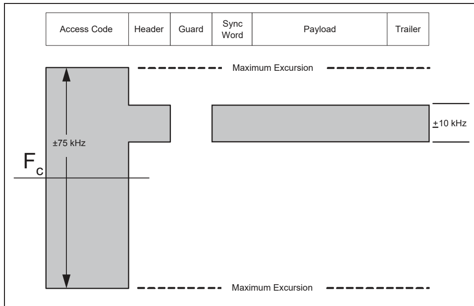
Figure 3.3: Carrier frequency mask
