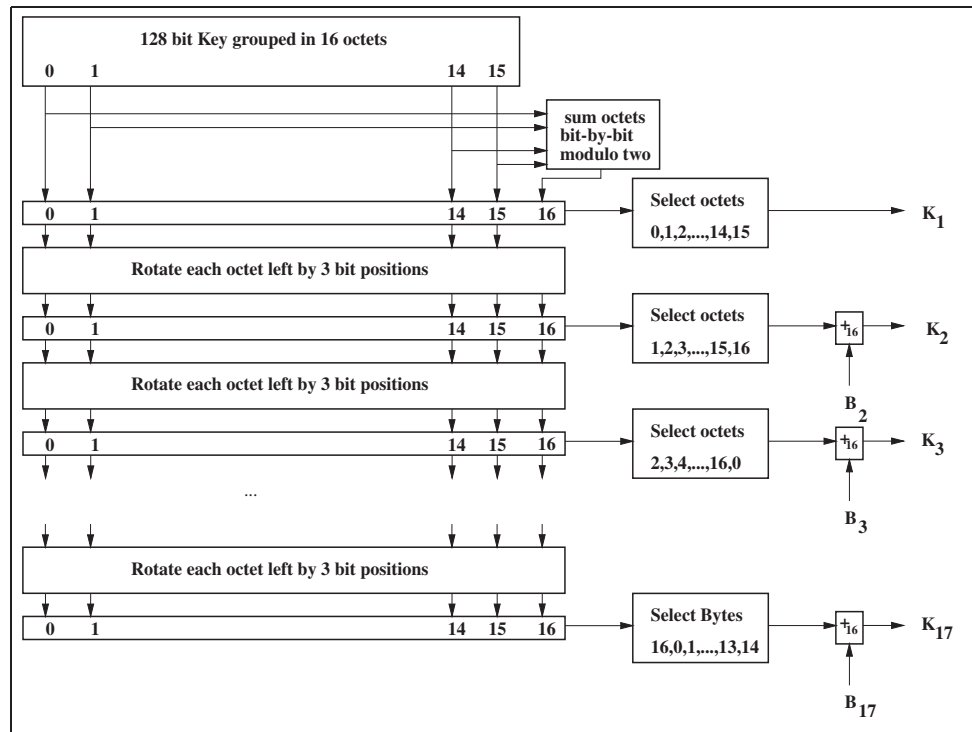
Figure 6.3: Key scheduling in A_1 .
