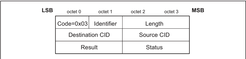
Figure 4.5: Connection Response Packet
