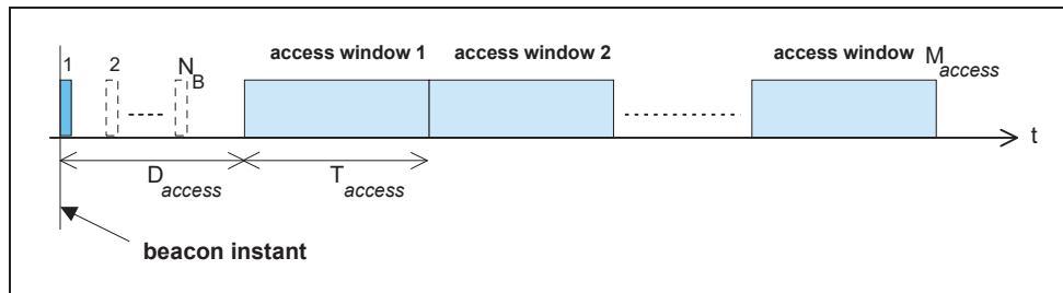
Figure 8.15: Definition of access window
