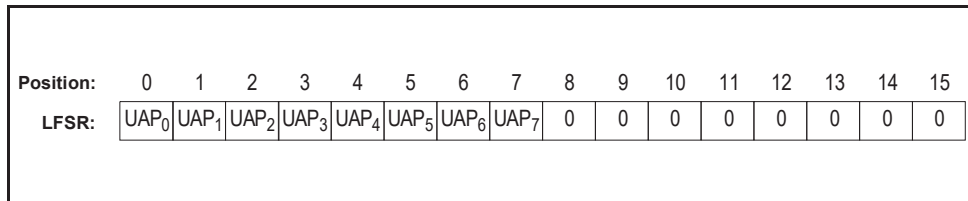
Figure 7.7: Initial state of the CRC generating circuit.
