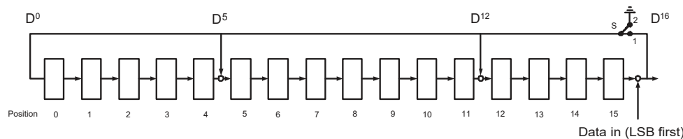
Figure 5.1: The LFSR Circuit Generating the CRC
