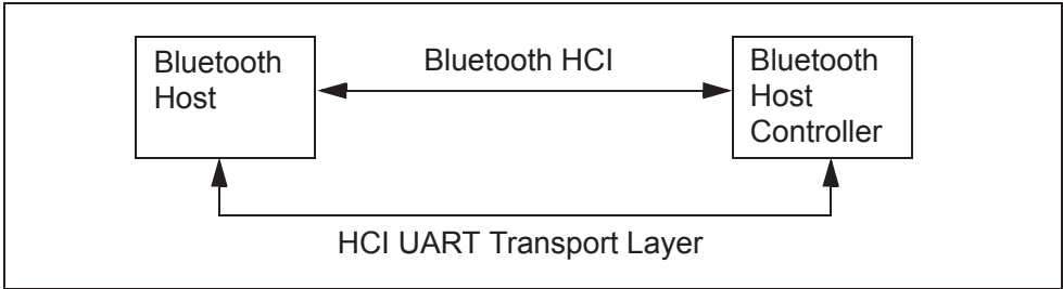
Figure 1.1: HCI UART Transport Layer
