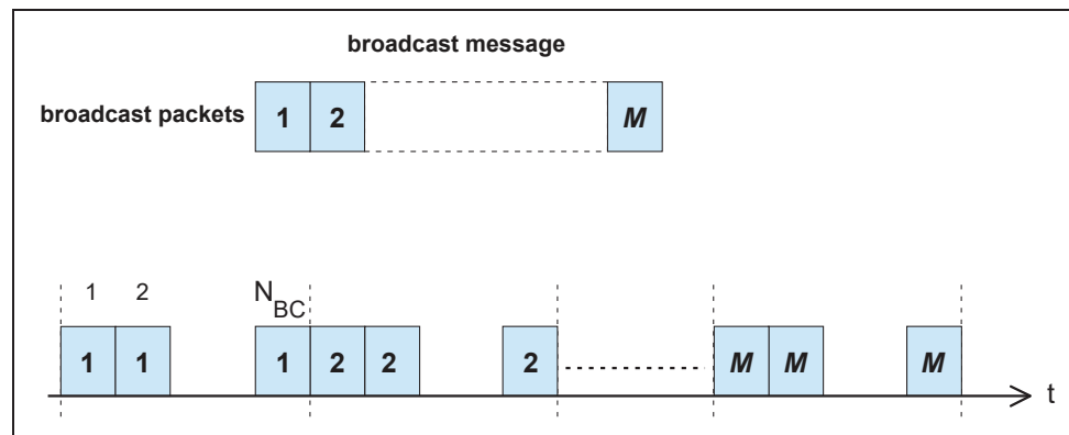
Figure 7.16: Broadcast repetition scheme
