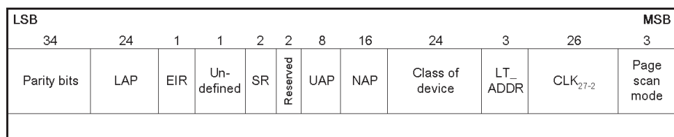
Figure 6.9: Format of the FHS payload.
