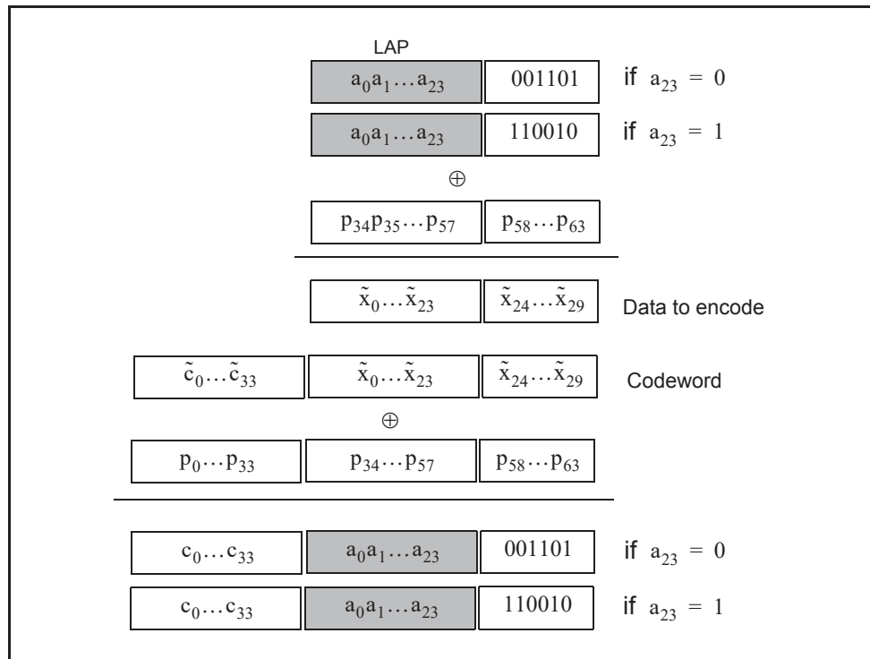
Figure 6.5: Construction of the sync word.
