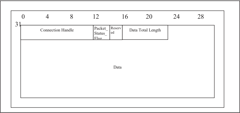
Figure 5.3: HCI Synchronous Data Packet
