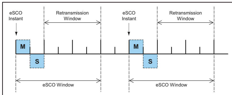
Figure 8.7: eSCO Window Details for Single-Slot Packets
