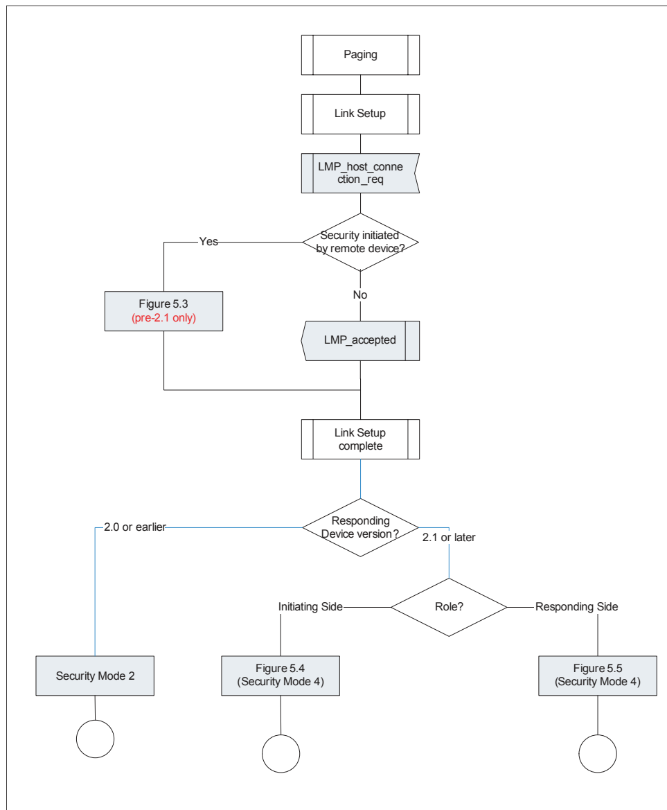
Figure 5.2: Channel establishment with security.
