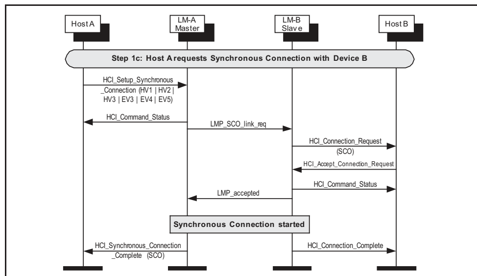
Figure 5.3: Master requests synchronous connection using SCO.
