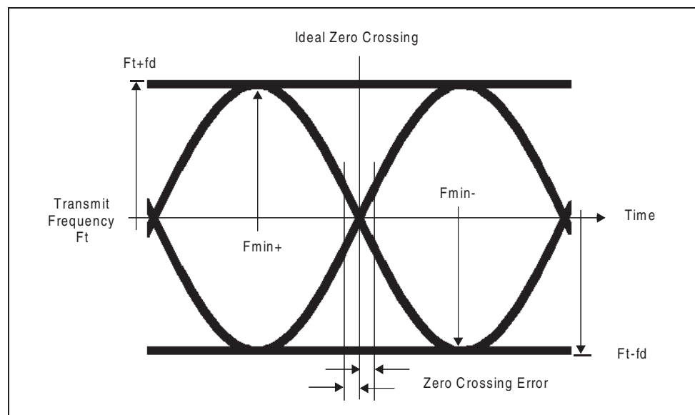
Figure 3.1: GFSK parameters definition.
