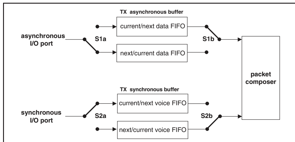
Figure 4.1: Functional diagram of TX buffering.
