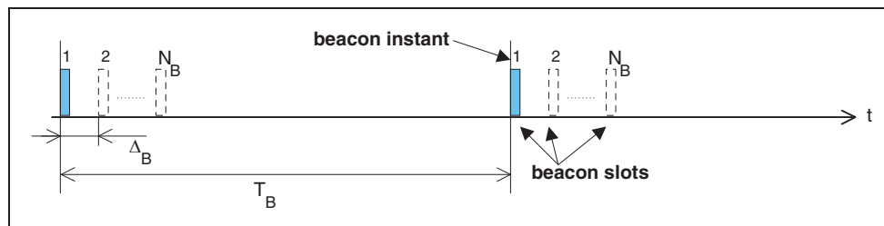
Figure 8.14: General beacon train format
