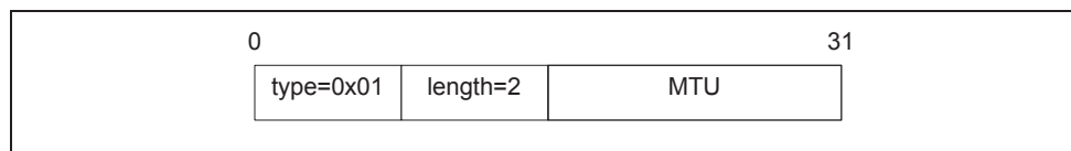
Figure 5.2: MTU Option Format
