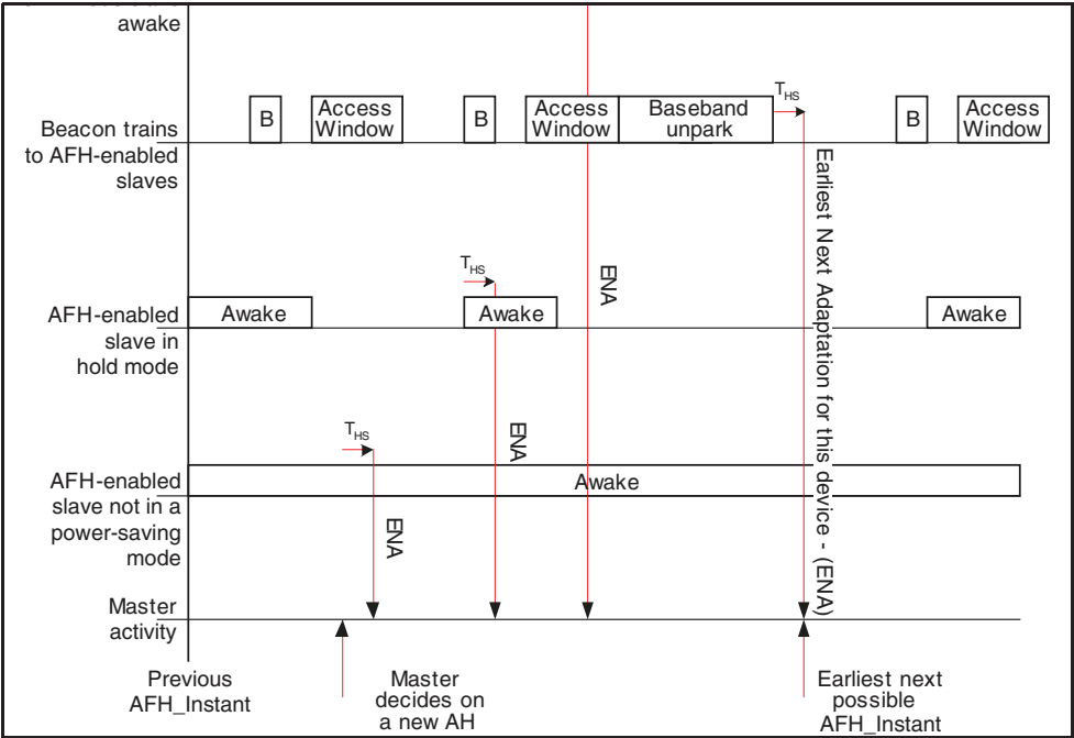
Figure 11.4: Timing constraint on AFH_Instant with slaves in park, hold and sniff
