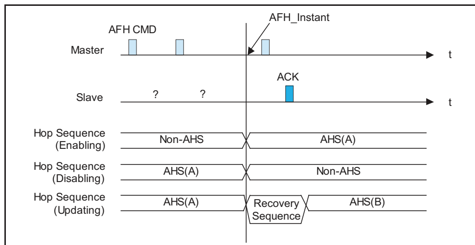
Figure 8.10: Recovery hop sequences
