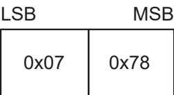
Figure 9.3: Sleep Message Payload Format
