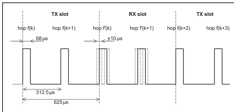
Figure 2.7: RX/TX cycle of transceiver in PAGE mode.
