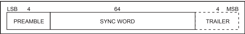
Figure 6.3: Access code format
