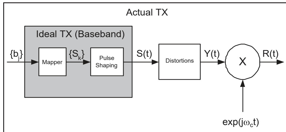
Figure 7.1: TX model.
