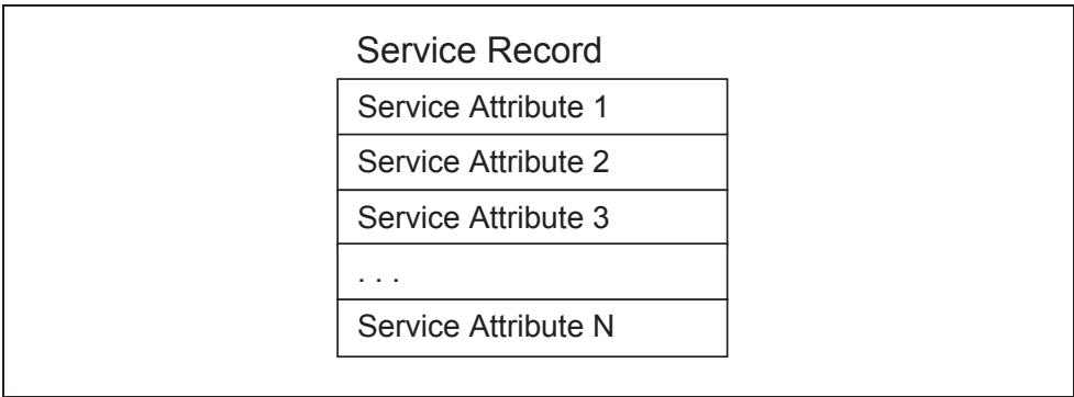
Figure 2.3: Service Record
