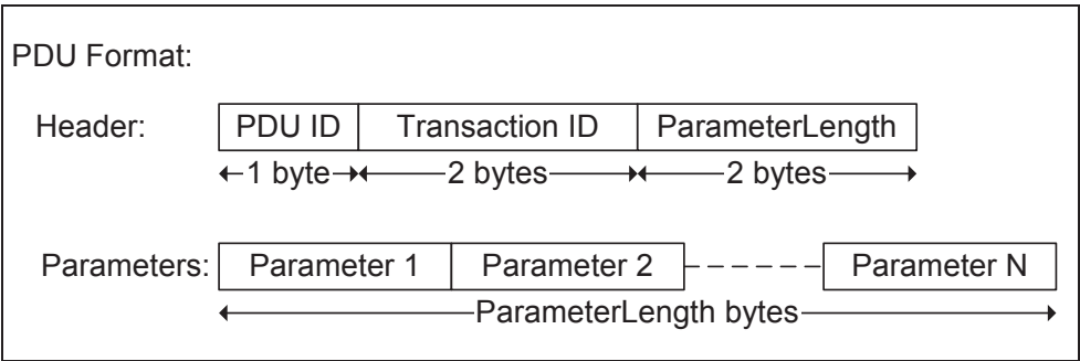
Figure 4.1:
