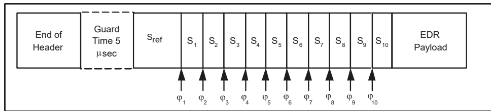
Figure 6.11: Synchronization sequence
