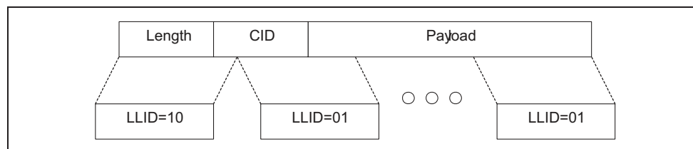
Figure 7.1: L2CAP fragmentation.
