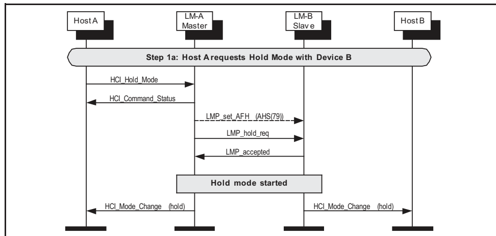
Figure 6.3: Hold request.
