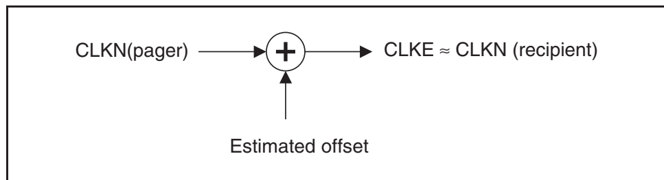
Figure 2.6: Derivation of CLKE.
