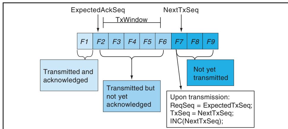
Figure 8.1: Example of the transmitter side
