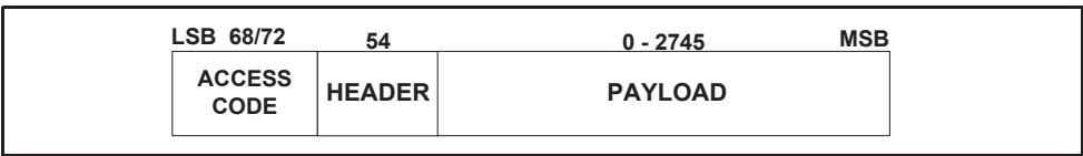
Figure 6.1: General Basic Rate packet format.
