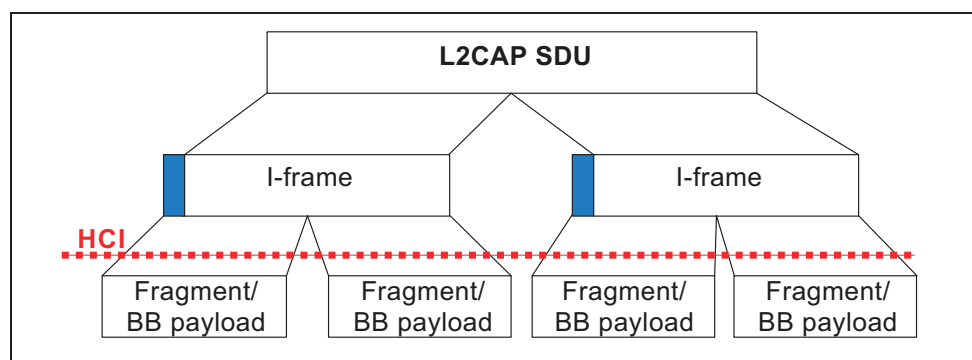
Figure 7.3: Segmentation and fragmentation of an SDU.
