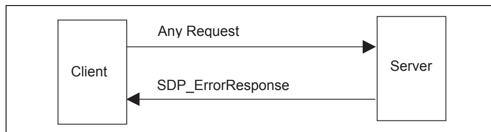
Figure 4.3:
