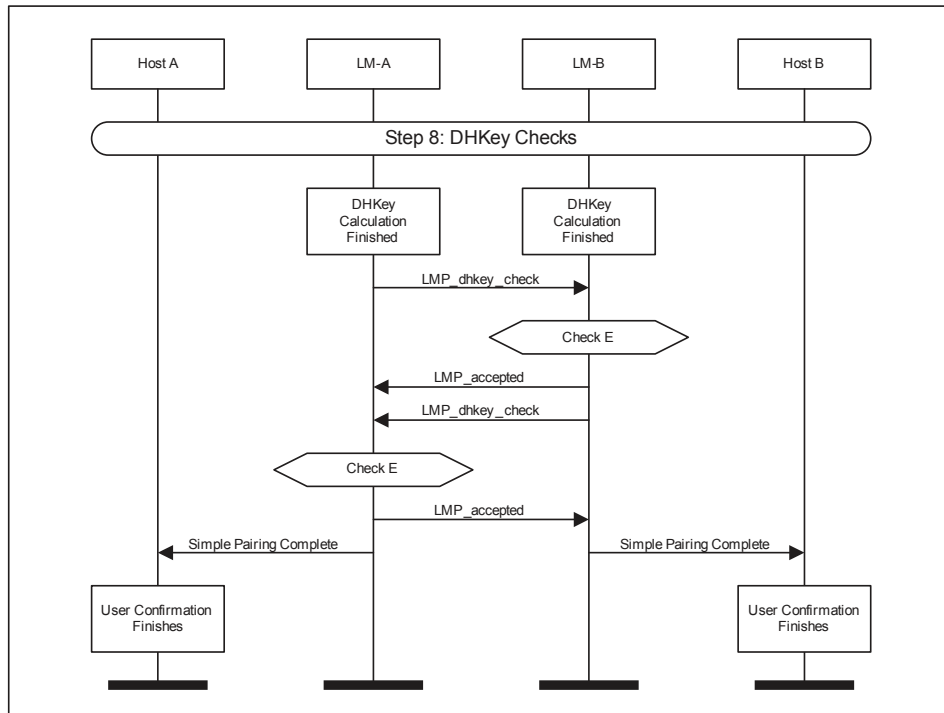
Figure 4.18: DHKey Checks
