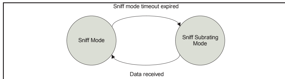
Figure 8.13: Sniff subrating
