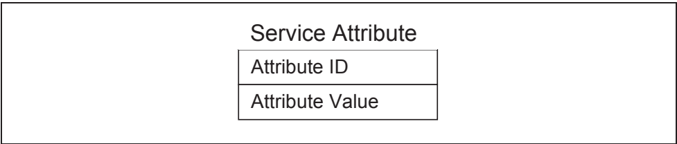
Figure 2.4: Service Attribute
