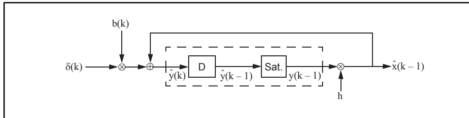
Figure 9.3: Accumulator procedure.
