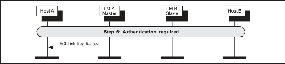
Figure 3.9: Authentication initiated.
