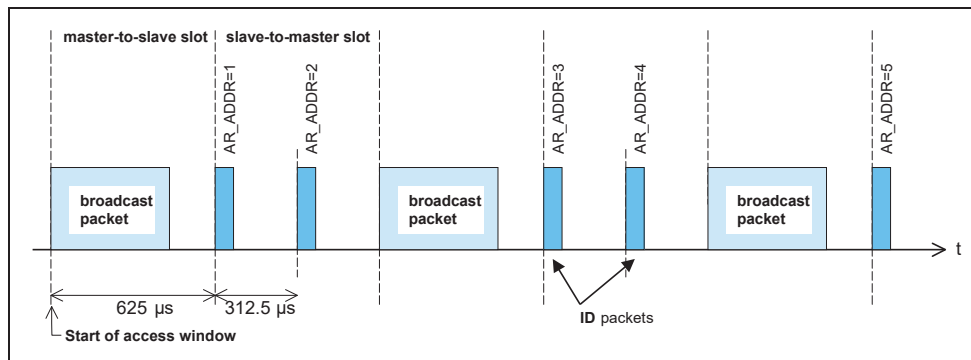
Figure 8.16: Access procedure applying the polling technique.
