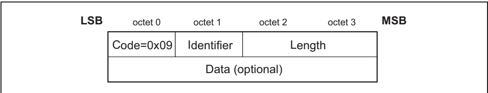
Figure 4.13: Echo Response Packet
