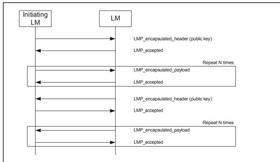
Sequence 46: Public key exchange
