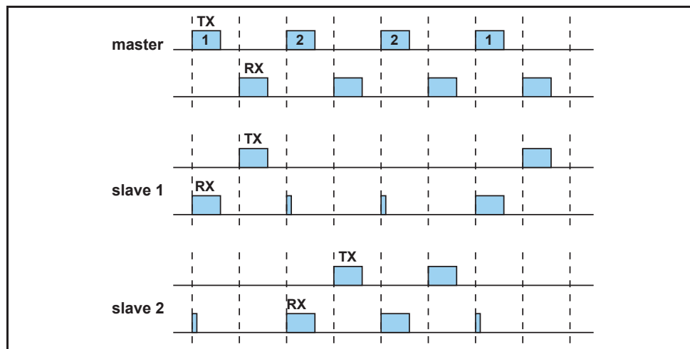
Figure 8.6: RX/TX timing in multi-slave configuration
