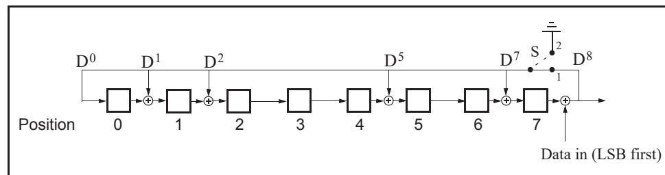
Figure 7.3: The LFSR circuit generating the HEC.
