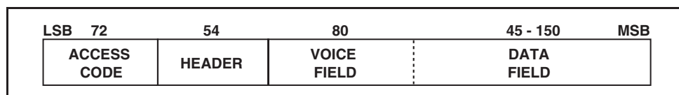
Figure 6.10: DV packet format
