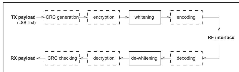
Figure 7.2: Payload bit processes.
