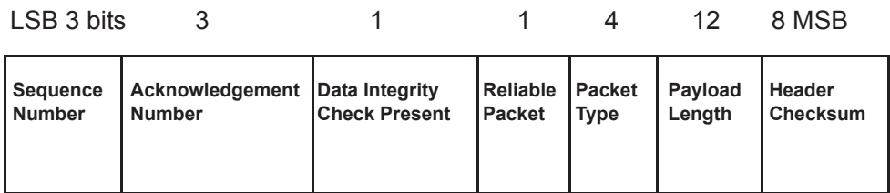
Figure 4.2: Packet Header Format
