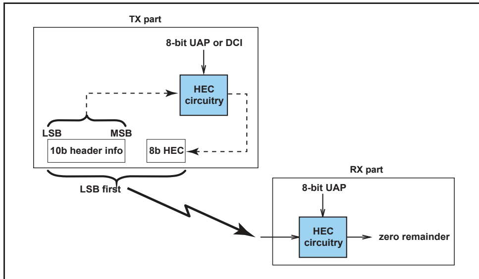
Figure 7.5: HEC generation and checking.
