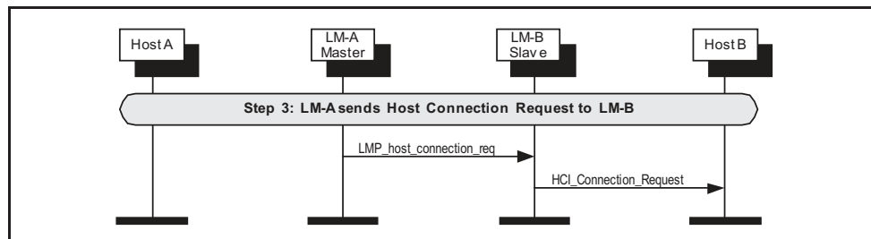
Figure 3.4: LM-A requests host connection.
