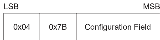
Figure 8.5: Configuration Response Message Format
