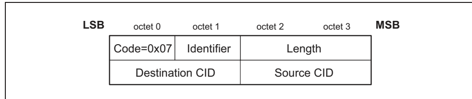
Figure 4.11: Disconnection Response Packet
