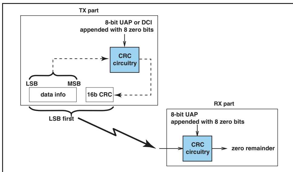
Figure 7.8: CRC generation and checking.
