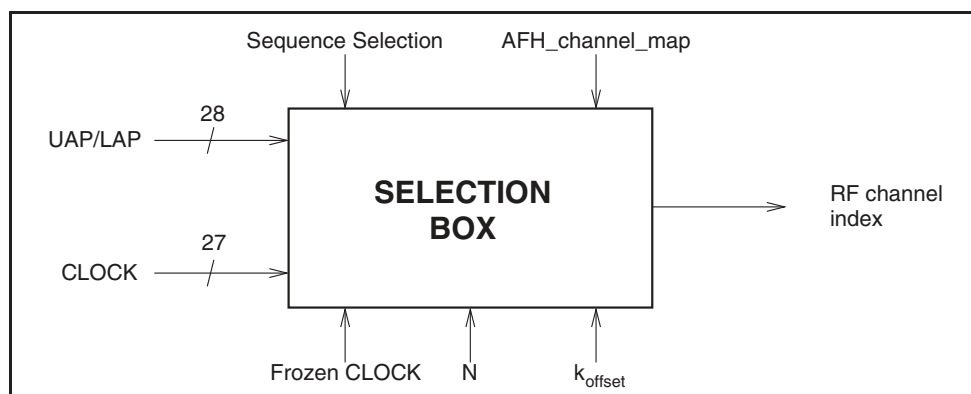
Figure 2.12: General block diagram of hop selection scheme.
