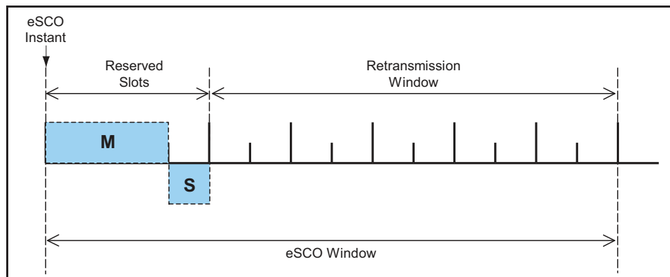
Figure 8.8: eSCO Window Details for Asymmetric Traffic
