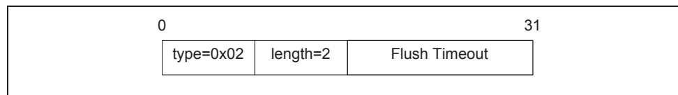
Figure 5.3: Flush Timeout option format.
