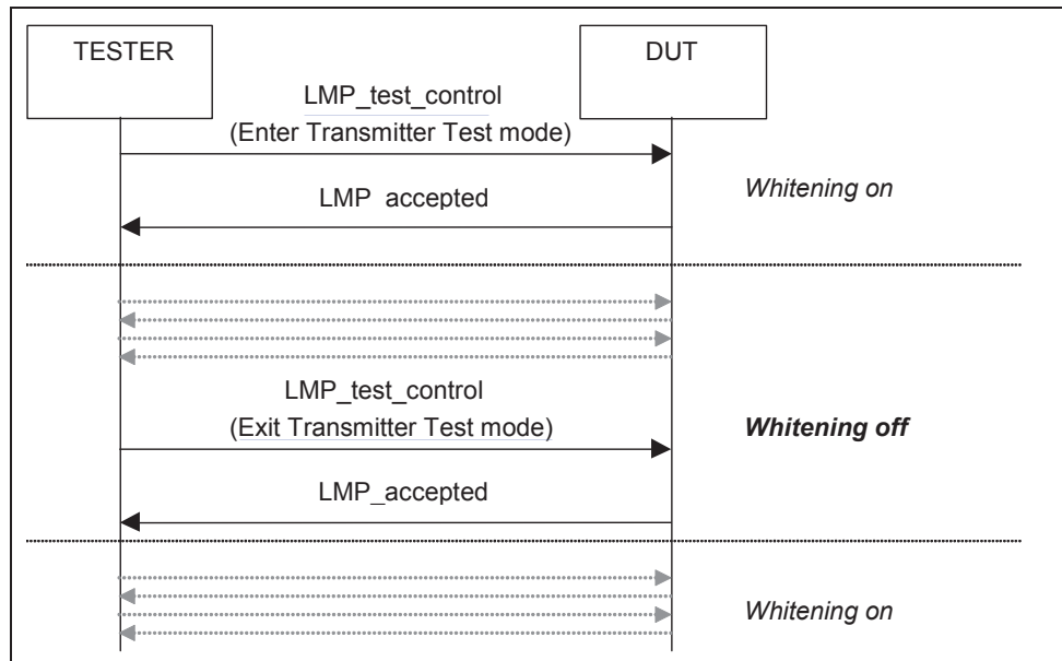
Figure 1.4: Use of whitening in Transmitter mode
