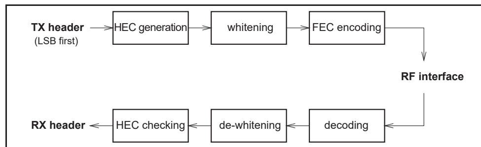
Figure 7.1: Header bit processes.
