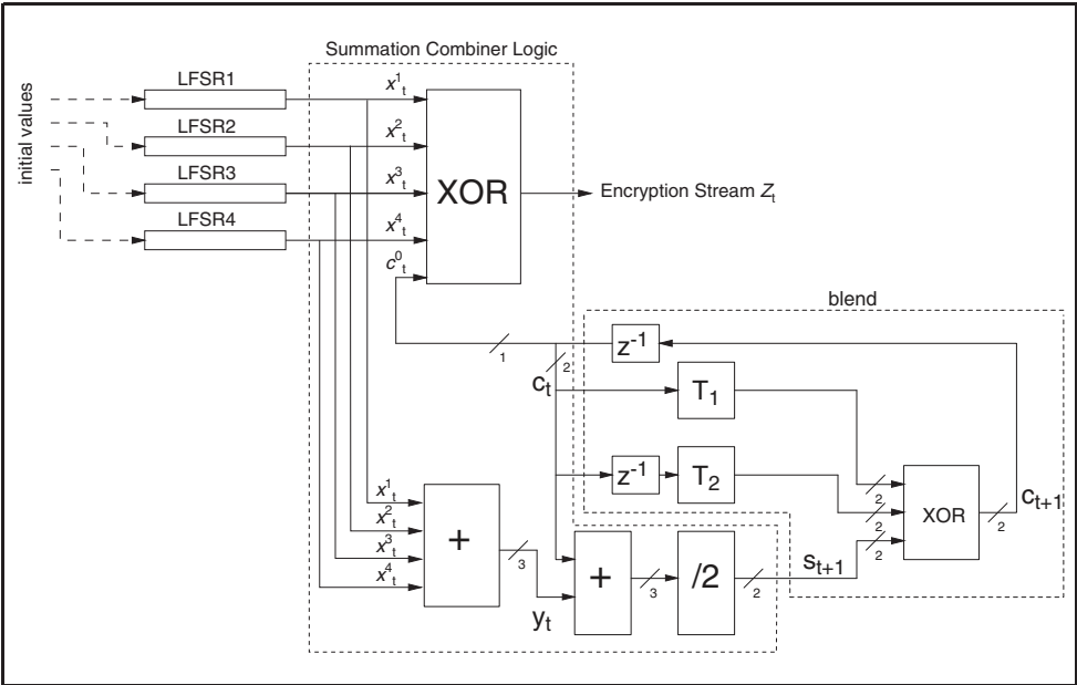
Figure 4.3: Concept of the encryption engine.
