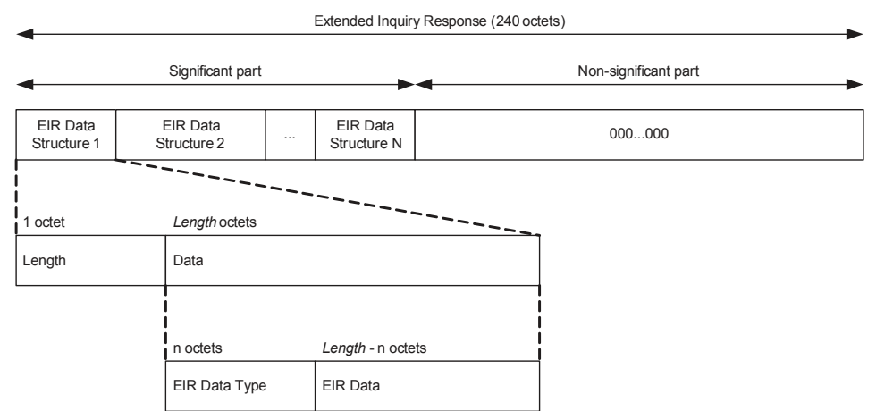
Figure 8.1: Extended Inquiry Response data format
