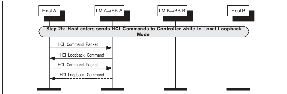
Figure 8.3: Looping back commands in local loopback mode.
