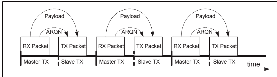
Figure 1.7: Payload & ARQN handling in normal loopback.
