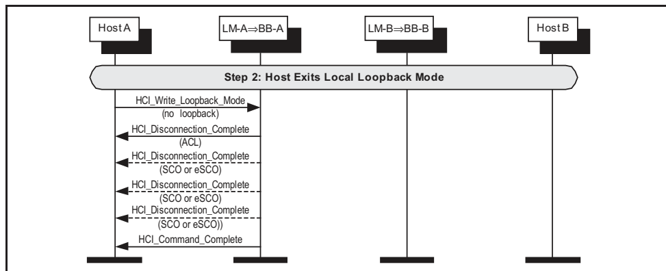
Figure 8.4: Exiting local loopback mode.
