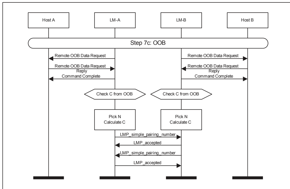
Figure 4.16: OOB Authentication
