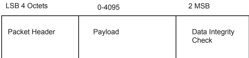
Figure 4.1: Packet Format
