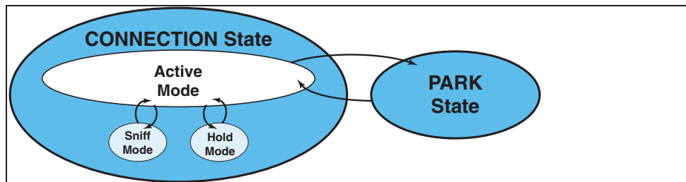
Figure 8.5: Connection state.
