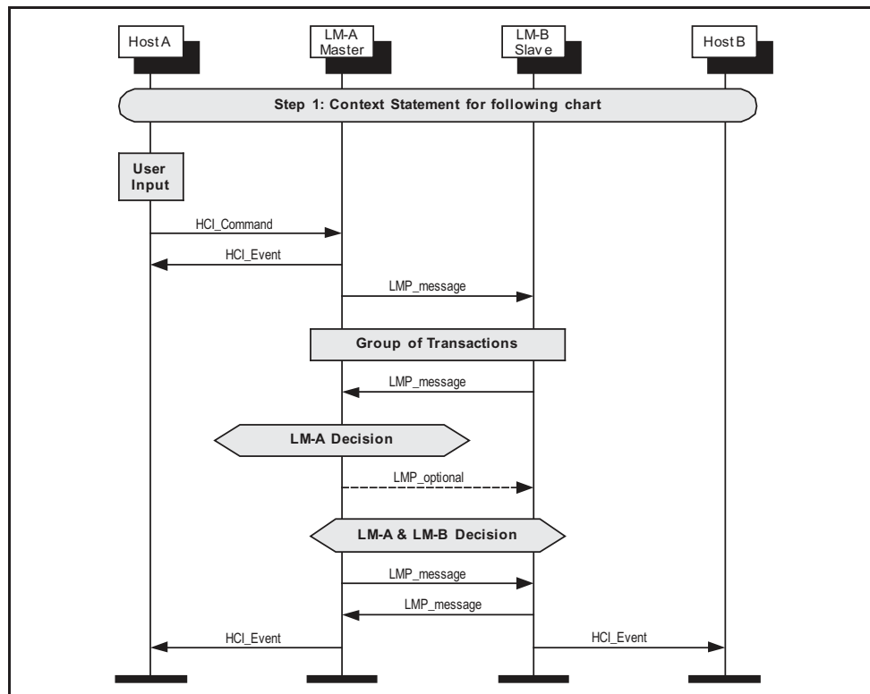
Figure 1.1: Example MSC.
