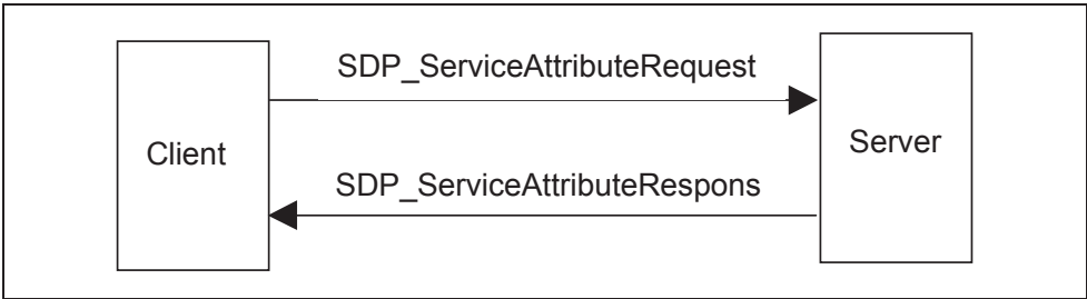
Figure 4.5:
