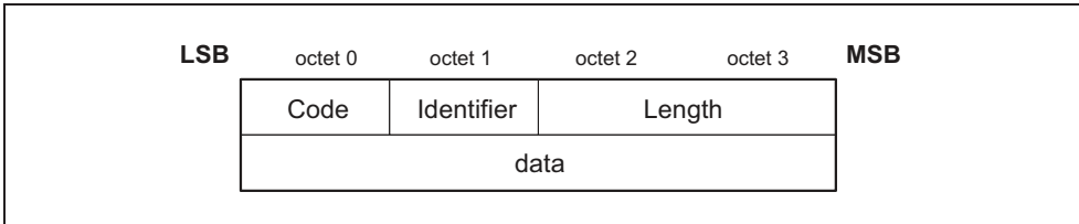
Figure 4.2: Command format
