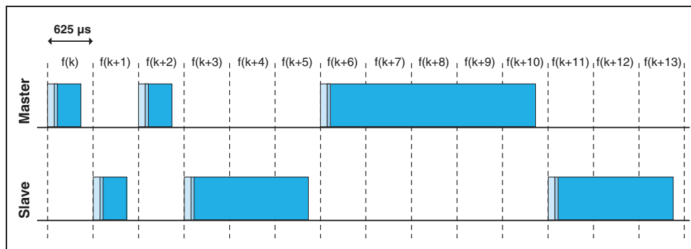
Figure 2.1: Multi-slot packets
