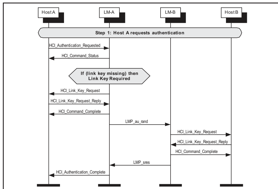
Figure 4.1: Authentication requested.
