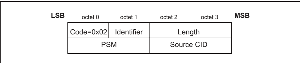
Figure 4.4: Connection Request Packet
