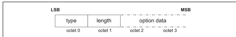
Figure 5.1: Configuration option format
