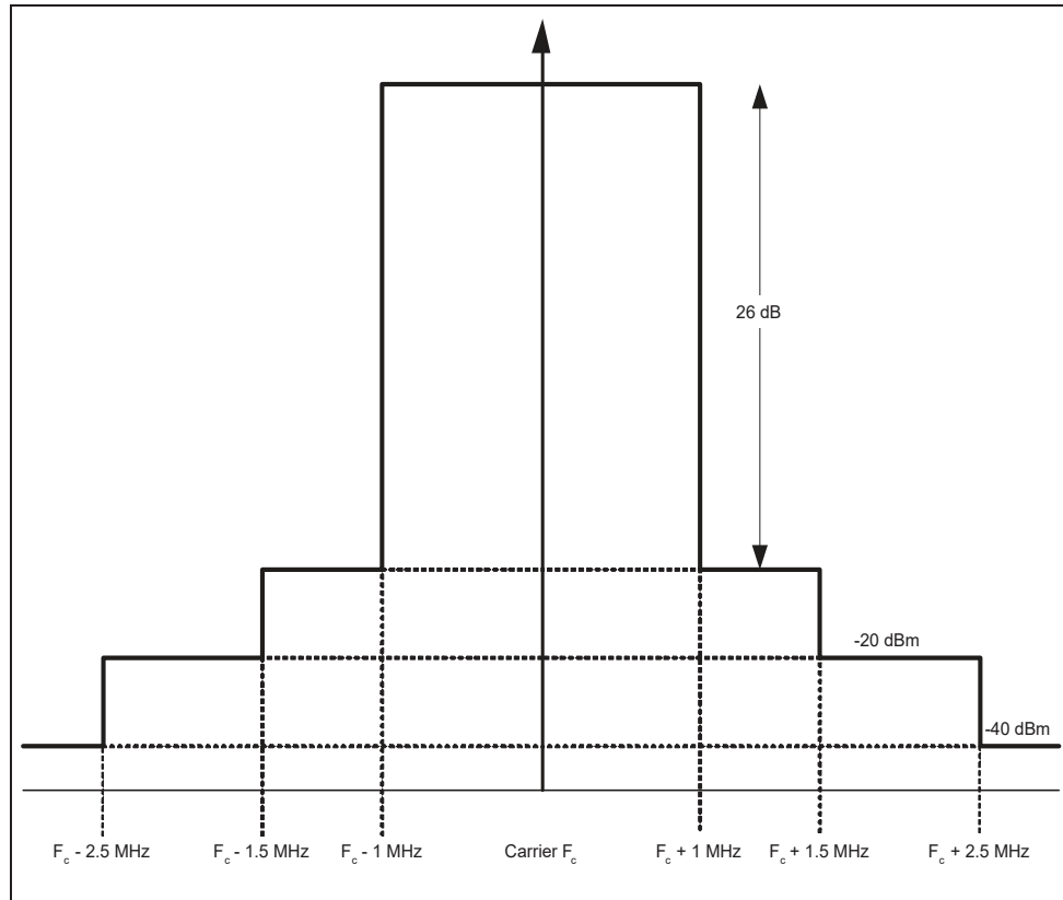
Figure 3.2: Transmitter spectrum mask
