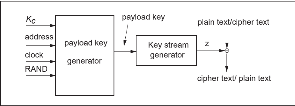
Figure 4.1: Stream ciphering for Bluetooth with E_0 .
