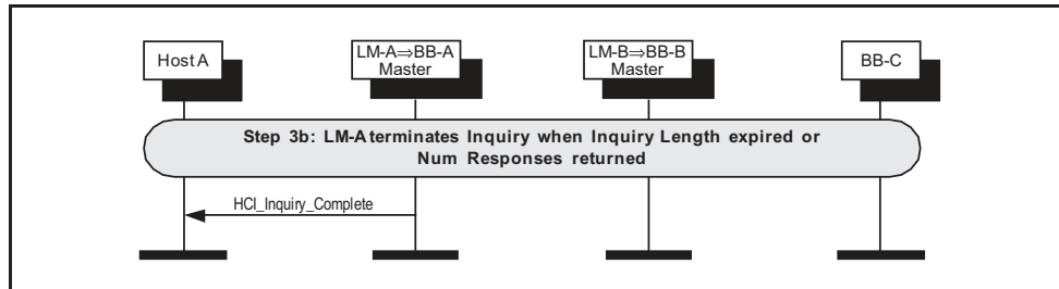
Figure 2.7: LM-A terminates current inquiry.
