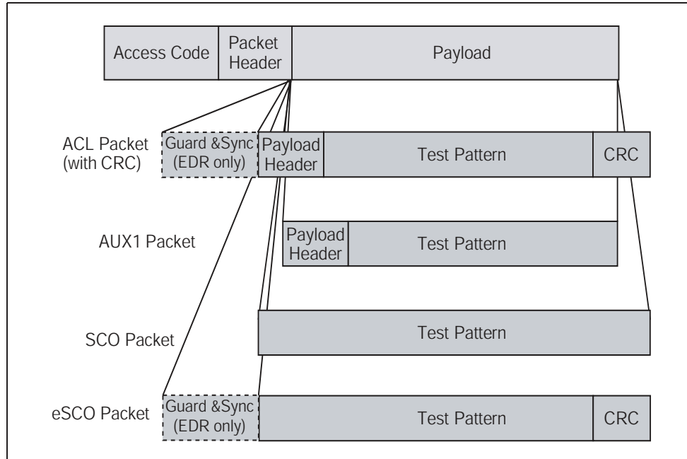
Figure 1.3: General Format of TX Packet
