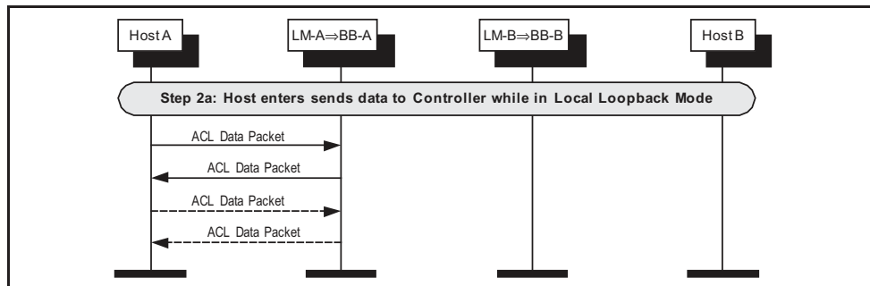
Figure 8.2: Looping back data in local loopback mode.
