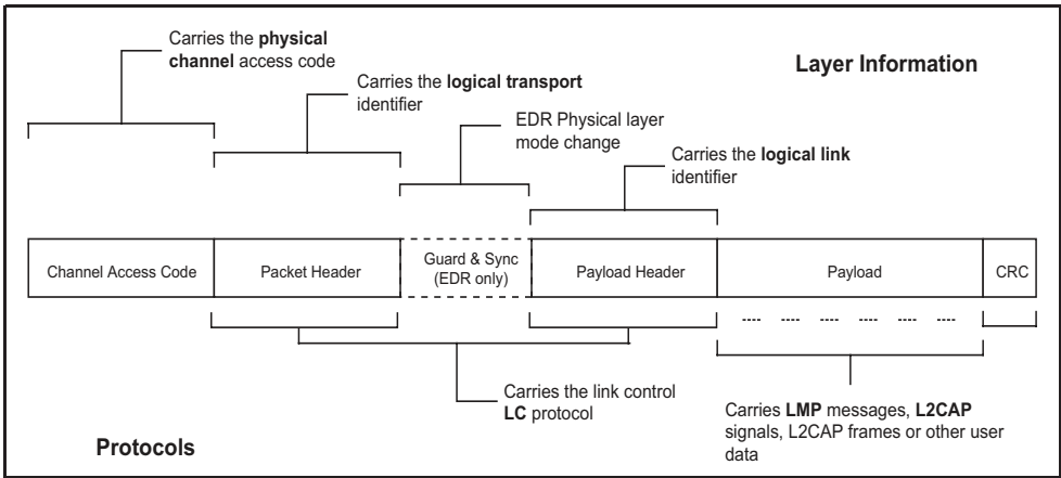
Figure 3.4: Bluetooth packet structure
