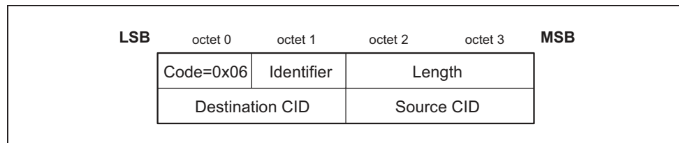
Figure 4.10: Disconnection Request Packet
