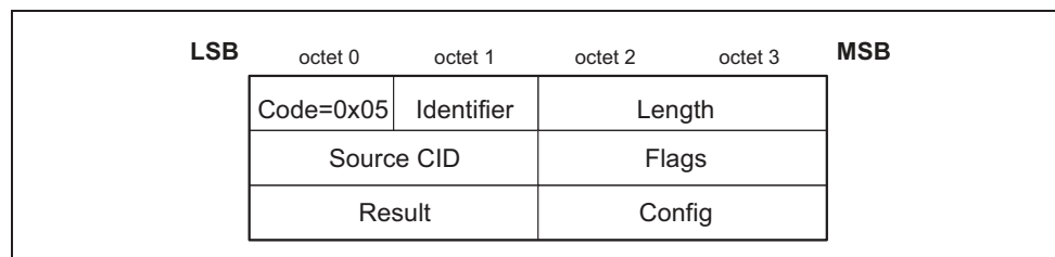
Figure 4.8: Configuration Response Packet
