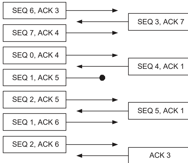
Figure 6.1: Message Diagram Showing Transmission of Reliable Packets
