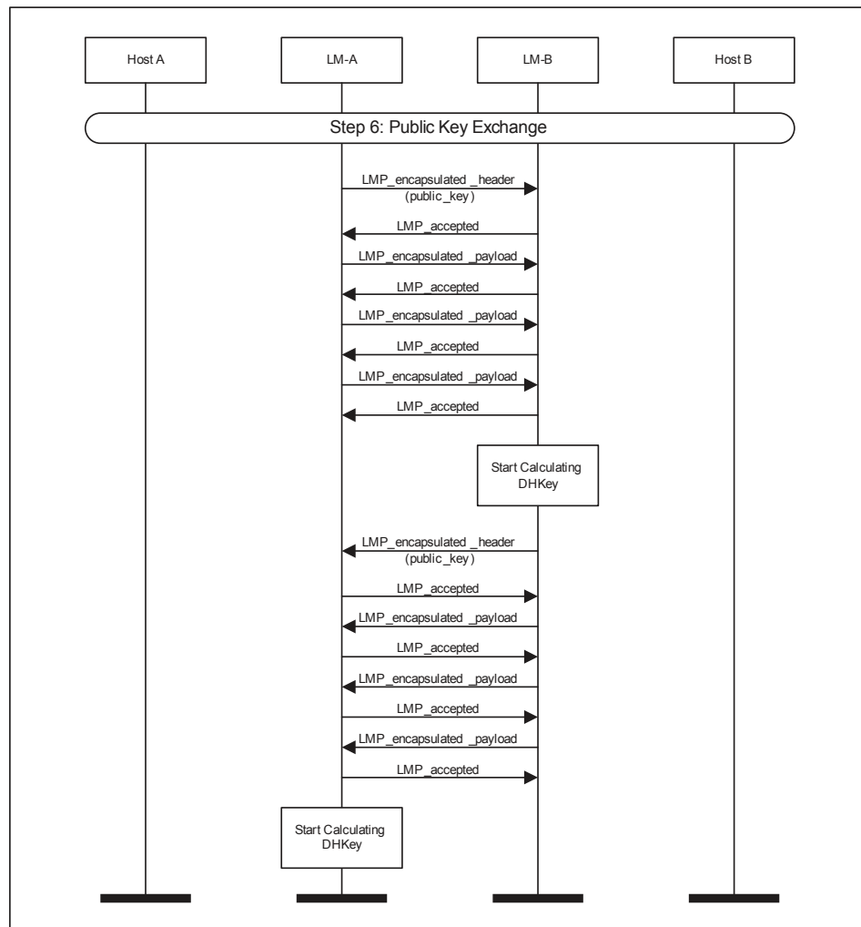
Figure 4.9: Public Key Exchange
