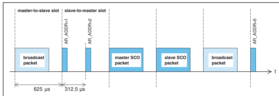
Figure 8.17: Disturbance of access window by SCO traffic
