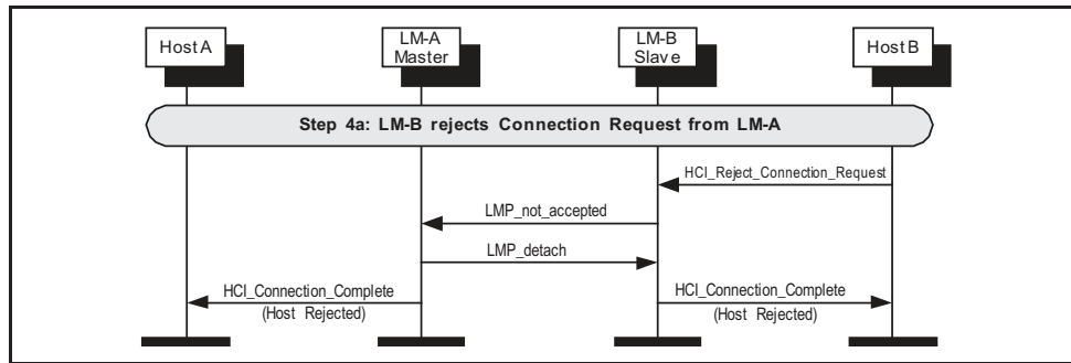
Figure 3.5: Device B rejects connection request.
