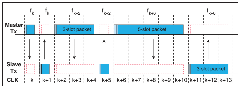
Figure 2.15: Example of the same channel mechanism.
