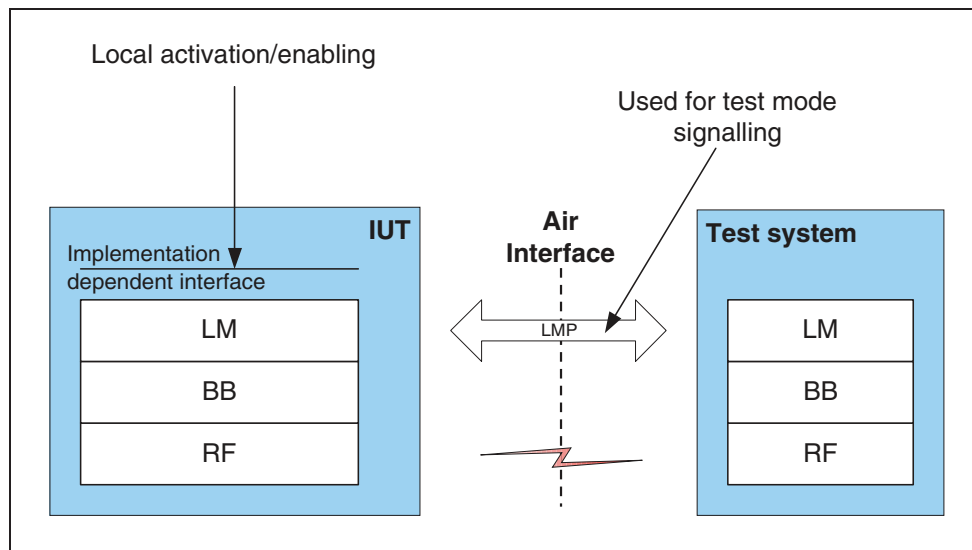
Figure 2.1: General test set-up for RF qualification
