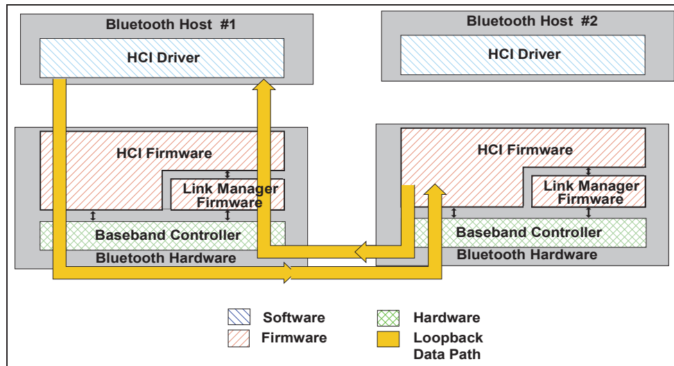
Figure 7.2: Remote Loopback Mode
