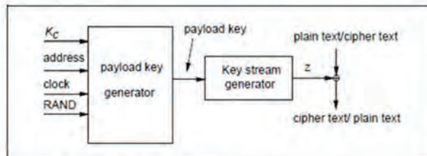
Figure 4.1: Stream ciphering for Bluetooth with E_0 .
