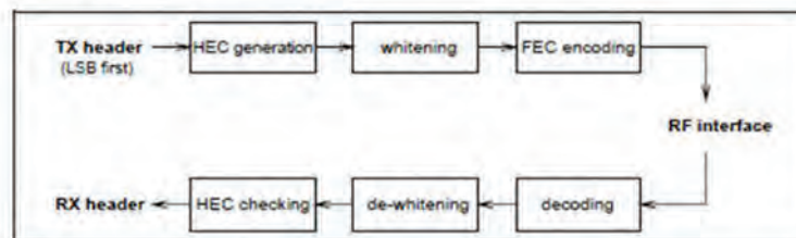
Figure 7.1: Header bit processes.
