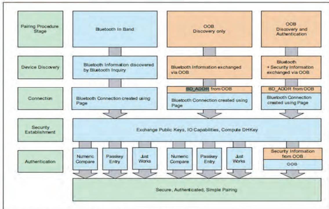
Figure 5.1: Secure Simple Pairing Association Models
