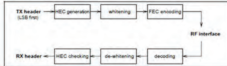
Figure 7.1: Header bit processes.
