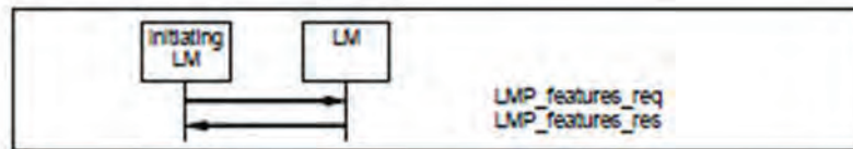
Sequence 08: Request for supported features.
