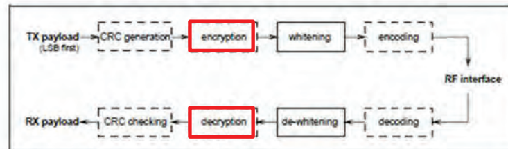
Figure 7.2: Payload bit processes.
