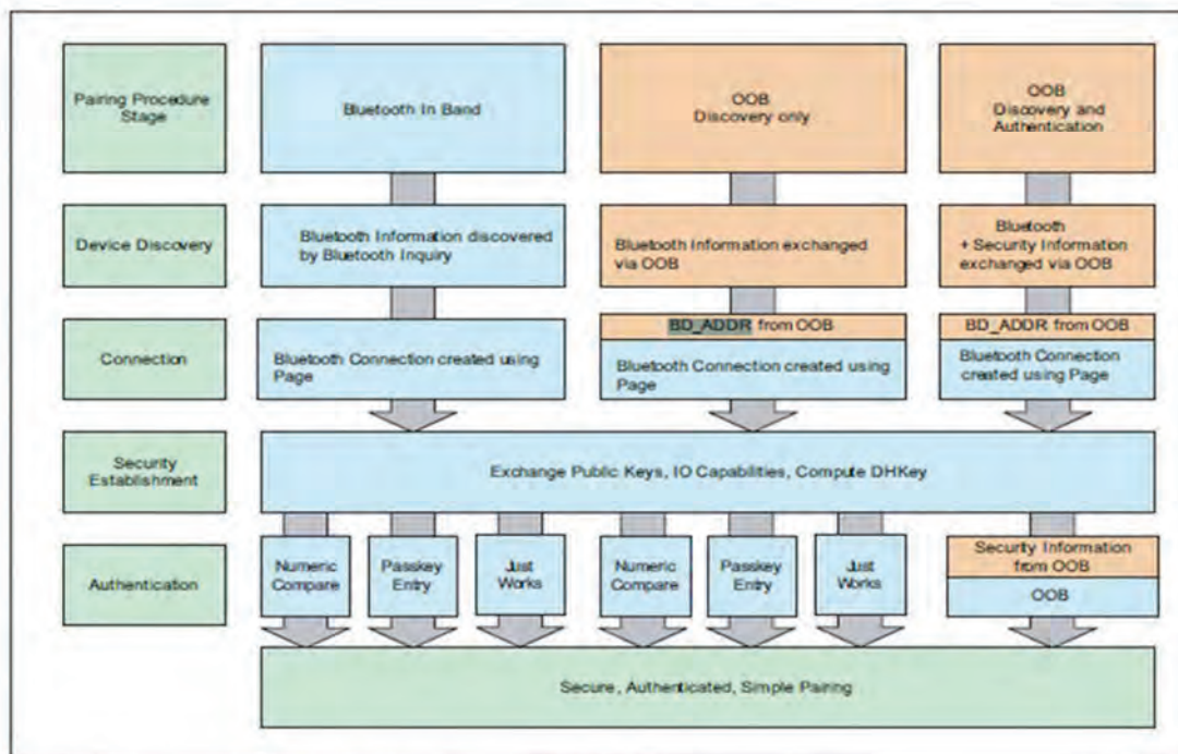
Figure 5.1: Secure Simple Pairing Association Models
