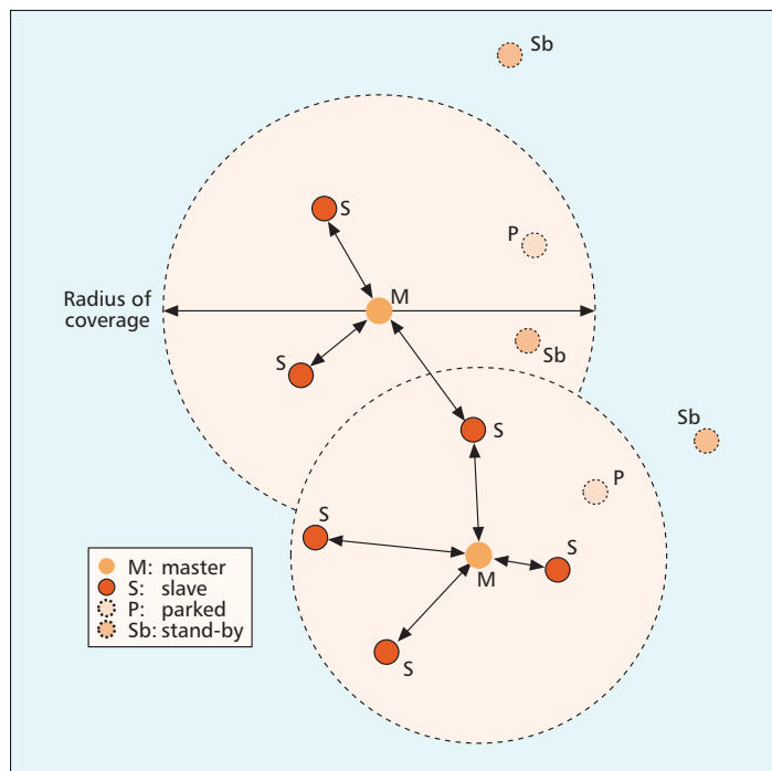
Figure 2. Bluetooth piconets.
