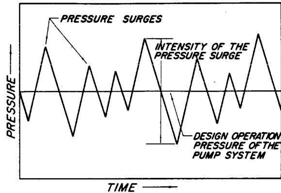
Fig. 2—Pressure-vs-time curve showing the effects of pressure surging.
