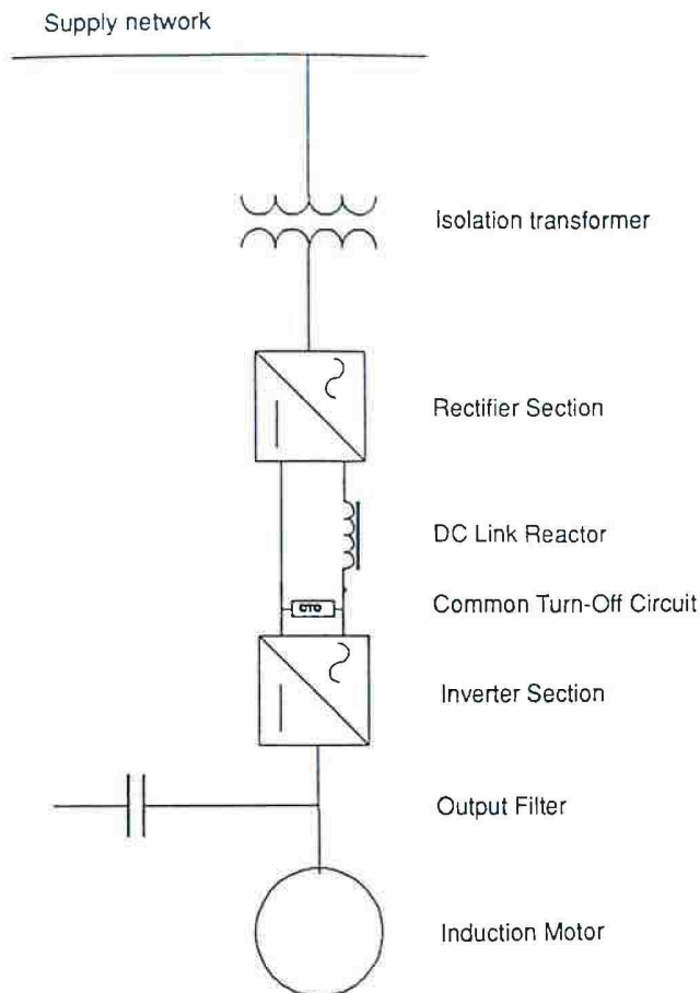
FIG. 20-76 LCI drive with induction motor.
