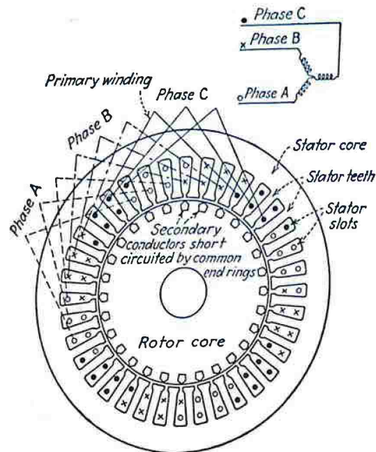
FIG. 20-20 Section of squirrel-cage induction motor, 3-phase, 4-pole, 8/9-pitch stator winding.
