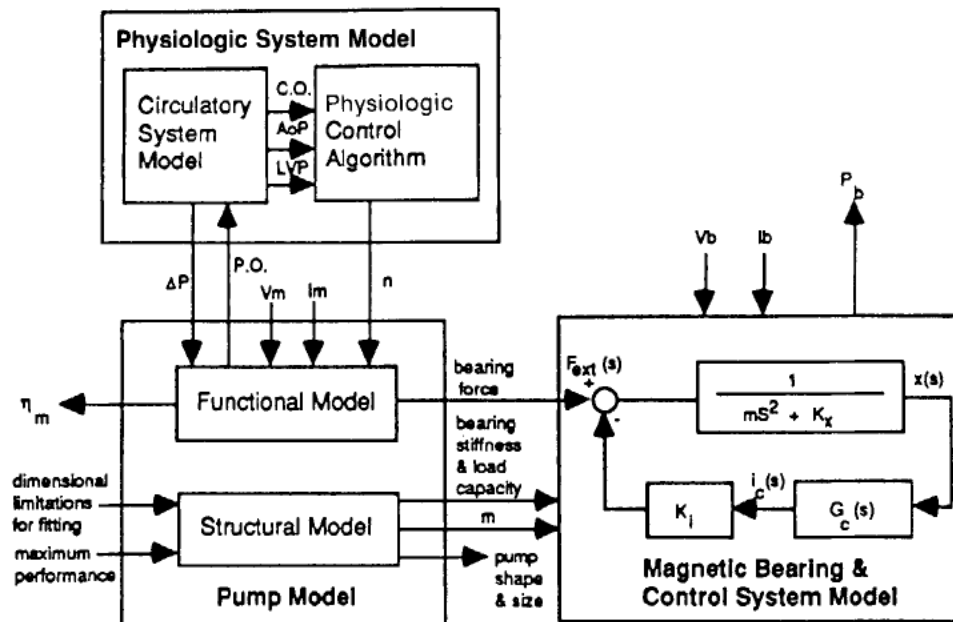
FIG. 2. The CFVAD system is depicted as a functional diagram. C.O., cardiac output; AoP, aortic pressure; LVP, left ventricular pressure; \Delta P , differential pressure across pump; P.O., pump output pressure; n , motor speed; V_m , I_m , and \eta_m , motor voltage, current, and efficiency; m , motor mass; V_b , I_b , and P_b , magnetic bearing voltage, current, and power consumption; G_c(s) , controller transfer function; K_i , actuator gain; K_x , open loop stiffness; i_c(s) , control current; x(s) , rotor position; F_{ext}(s) , external force.
