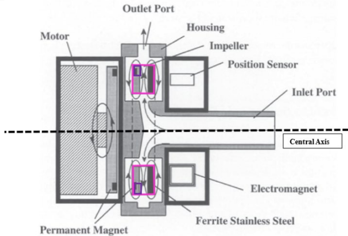
Fig. 2. Schematic cross section of the MSCP
