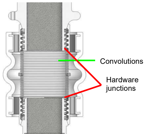
Figure 2A: Inflow cannula preclotting must ensure coating between convolutions and at junction of hardware and graft.
