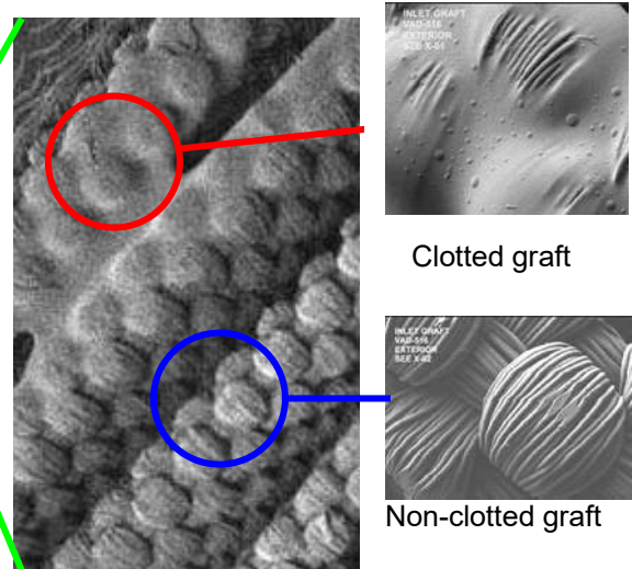
Figure 2B: Scanning electron microscopy after explantation shows preclotting material not completely covering graft.
