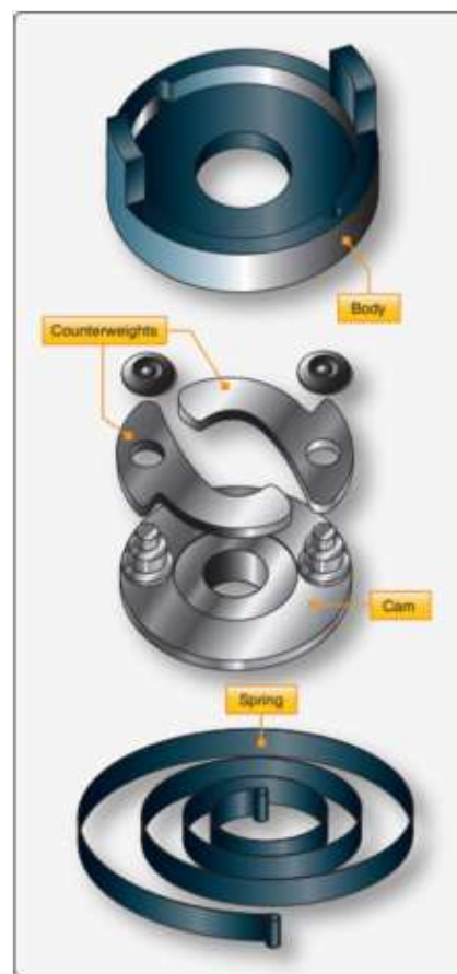
Impulse coupling components.
