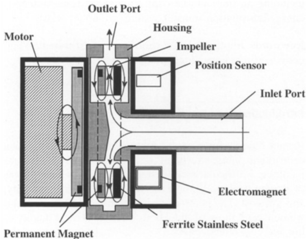
Fig. 2. Schematic cross section of the MSCP
