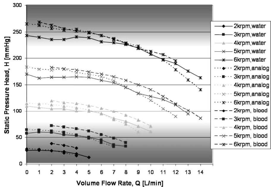
H-Q Characteristic w/ Blood Analog, H 2 O, & Bovine Blood
