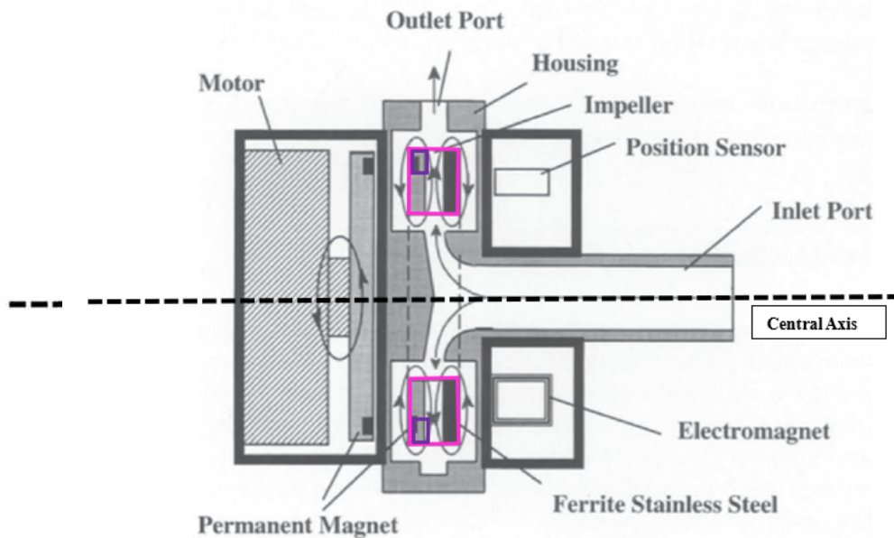
Fig. 2. Schematic cross section of the MSCP
