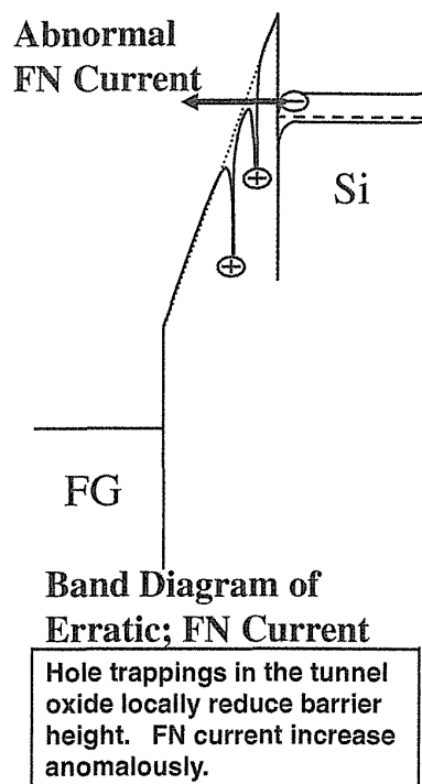
FIGURE 6.69 Schematic model of erratic over-program. Two hole traps in tunnel oxide induce an abnormal FN current.
