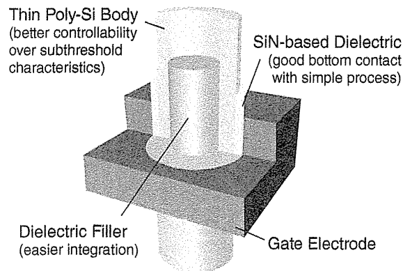
FIGURE 7.15 Concept of ‘macaroni’ body vertical transistor.
