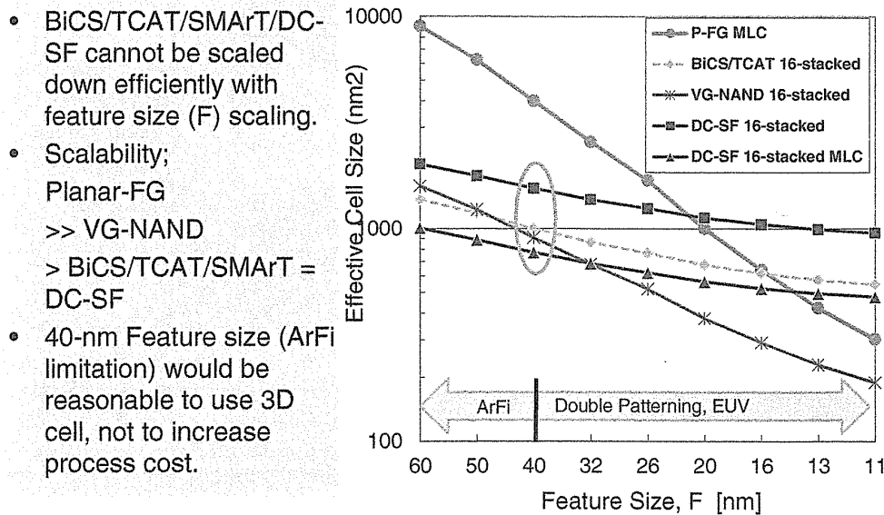
FIGURE 8.4 Scalability of 3D NAND flash memory cell.
