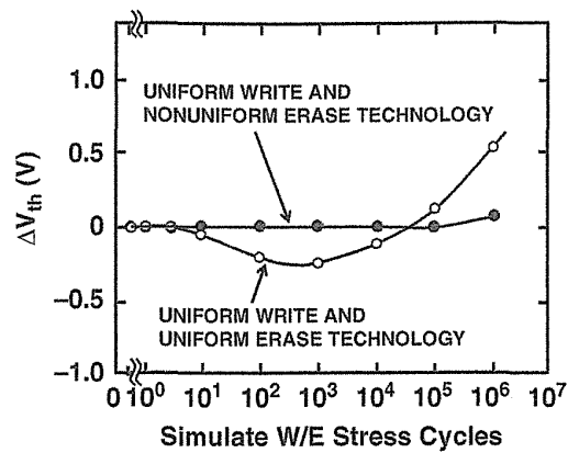
FIGURE 6.7 Threshold voltage shift of the test device in which the floating gate is connected with the control gate, during equivalent program and erase stress on tunnel-oxide. The equivalent program/erase stress condition: In the case of uniform program and uniform erase scheme, high-voltage pulses of 12.0 V, 0.1 ms, and 13.5 V, 0.1 ms are applied to the gate and substrate, respectively. In the case of the uniform program and nonuniform erase scheme, high-voltage pulses of 10.4 V, 0.1 ms and 13.0 V, 0.1 ms are applied to the gate and drain, respectively. In the uniform program and uniform erase scheme, the trapped oxide charges are directly affecting the threshold voltage. However, in uniform program and nonuniform erase scheme, the trapped oxide charges are not directly affecting the threshold voltage. Copyright © 1994 IEICE.
