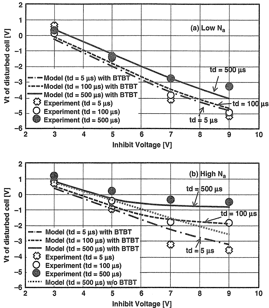
FIGURE 6.58 Disturbed cell V_t as a function of the inhibit voltage in the case of (a) low and (b) high channel boron concentrations of N_a . V_{seed} = 1 V. Initial erased V_t is below -7 V.
