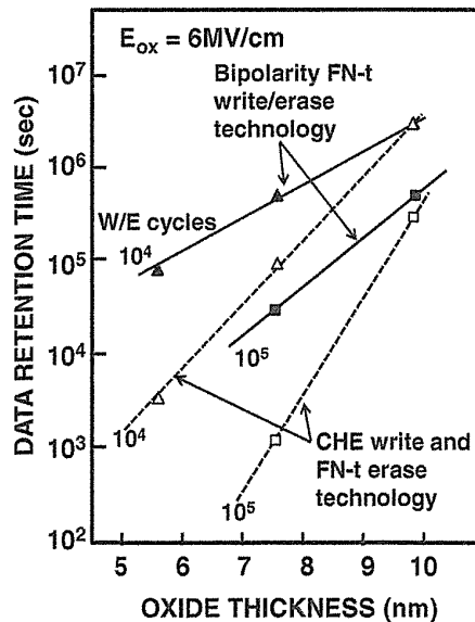
FIGURE 6.39 Data retention time of the flash memory cell after program and erase cycling as a function of tunnel-oxide thickness. Data retention time is defined by the time that V_{th} reaches -1.0\text{ V} during the applied gate voltage stress (accelerated read disturb condition). In bipolarity FN tunneling write/erase scheme, the tunnel-oxide thickness can be reduced with scaling down the flash memory cell.
