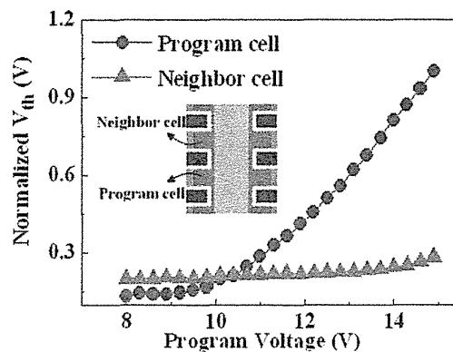
FIGURE 7.83 Program disturbance of neighbor cell. Low V_{\text{pass}_n-2} = 1 V is used.
